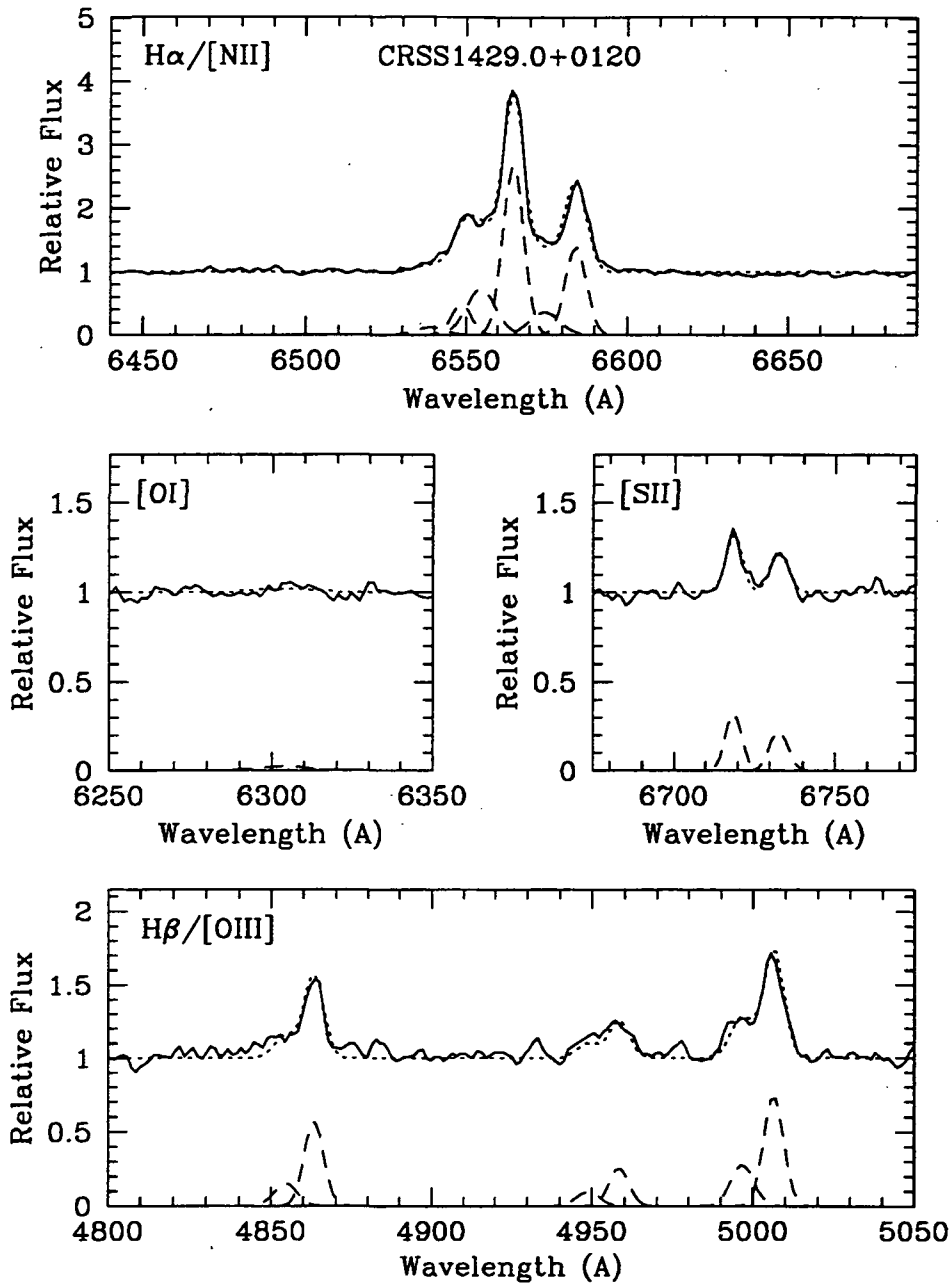
Figure 2 Expanded spectra of the regions around the prominent emission lines in a representative sample of 4 NLXG observed in our sample. The spectra have been corrected to the rest frame and been divided through by a low-order polynomial fit to the continuum. The accepted fit is denoted by the short dashed line. The contribution of the individual emission lines is shown by the longer dashed lines. (a) CRSS1429.0 + 0120: a starburst galaxy with asymmetric [OIII]/H \beta and [NII]/H \alpha .
