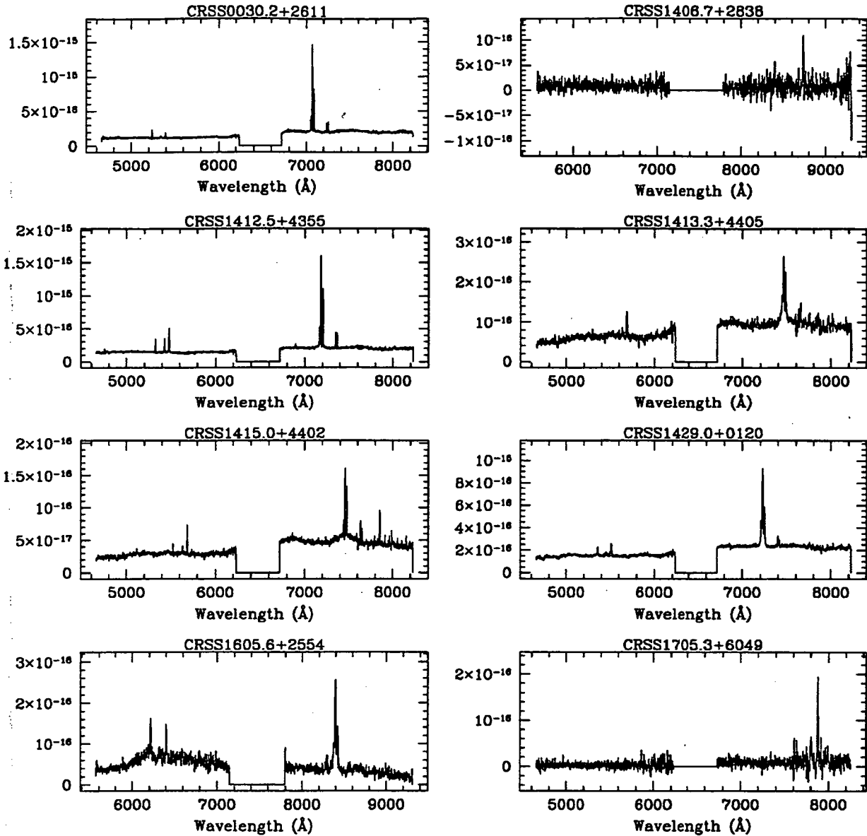
Figure 1 Intermediate-resolution ( 1.5 \text{ \AA} ) spectra for all 17 narrow emission-line galaxies observed in this program.
