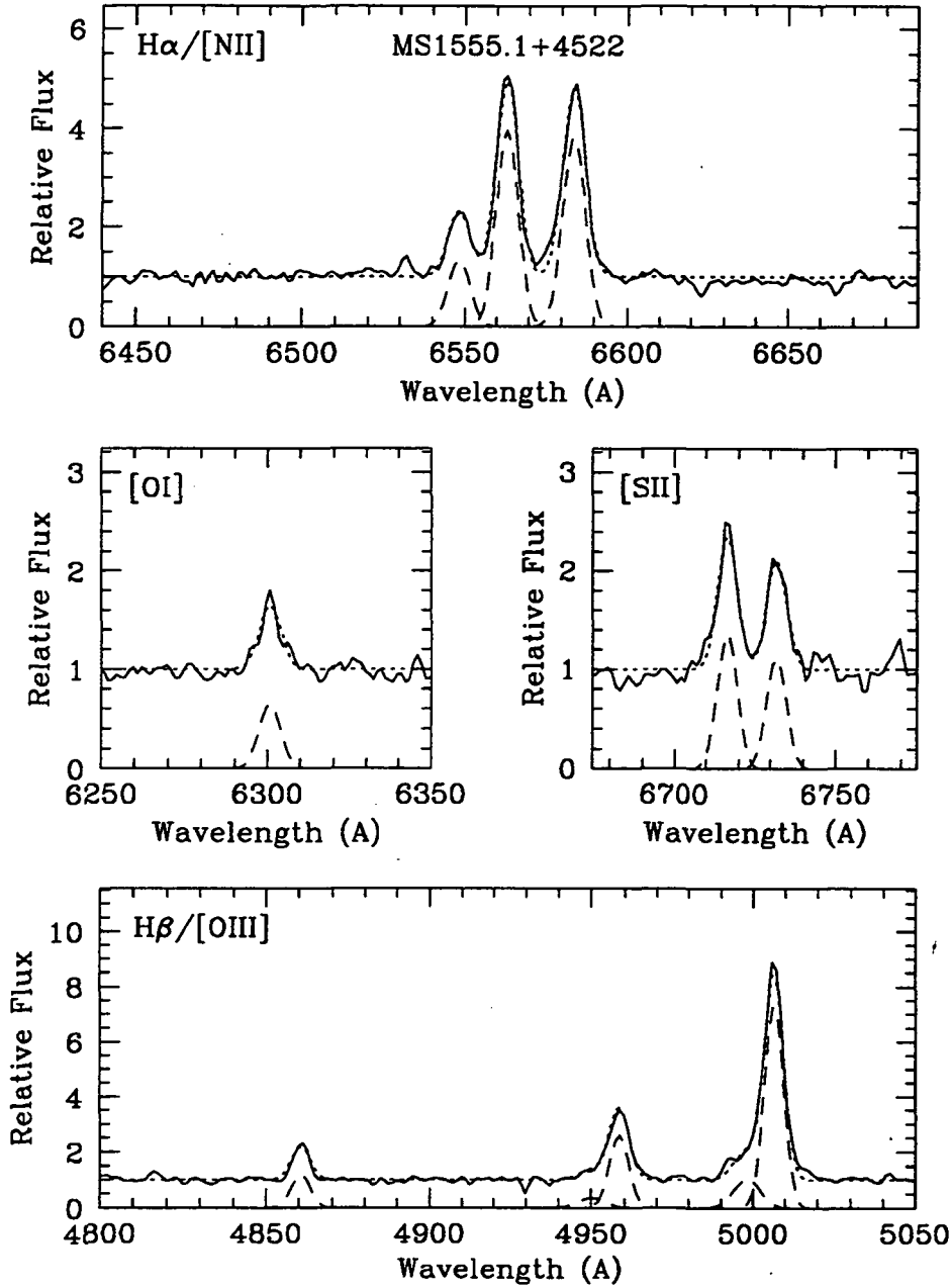
Figure 2(c) EMSS1555.1 + 4522: a Seyfert 2 galaxy with asymmetric [OIII].
