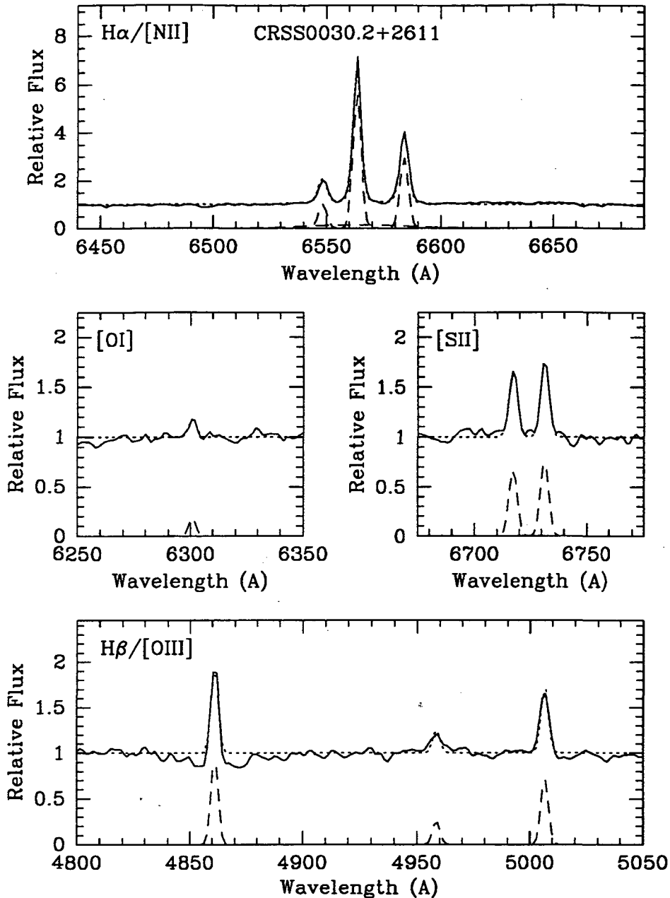
Figure 2(b) CRSS0030.2 + 2611: a starburst galaxy with weak broad H \alpha .
