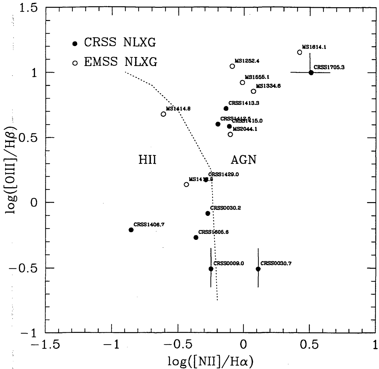
Figure 3 [NII]\lambda 6584/H\alpha - [OIII]\lambda 5007/H\beta emission-line ratio diagram for the NLXGs observed in this paper. CRSS objects are indicated by the filled circles and EMSS objects by the open circles. The division between AGN-like and HII-like spectra (dotted line) is based on the criterion of Baldwin, Philips & Terlevich (1981).
