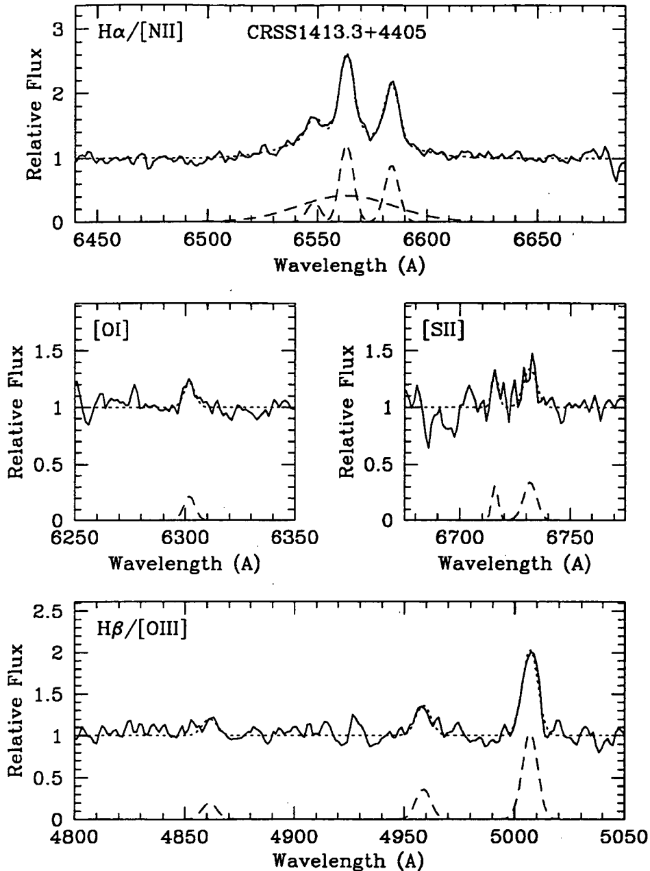
Figure 2(d) CRSS1413.3 + 4405: a Seyfert 1.5 galaxy.
