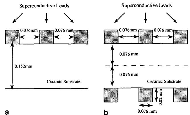
Figure 2 Printing configurations for superconductive leads printed on (a) single side of substrate and (b) both sides of substrate
