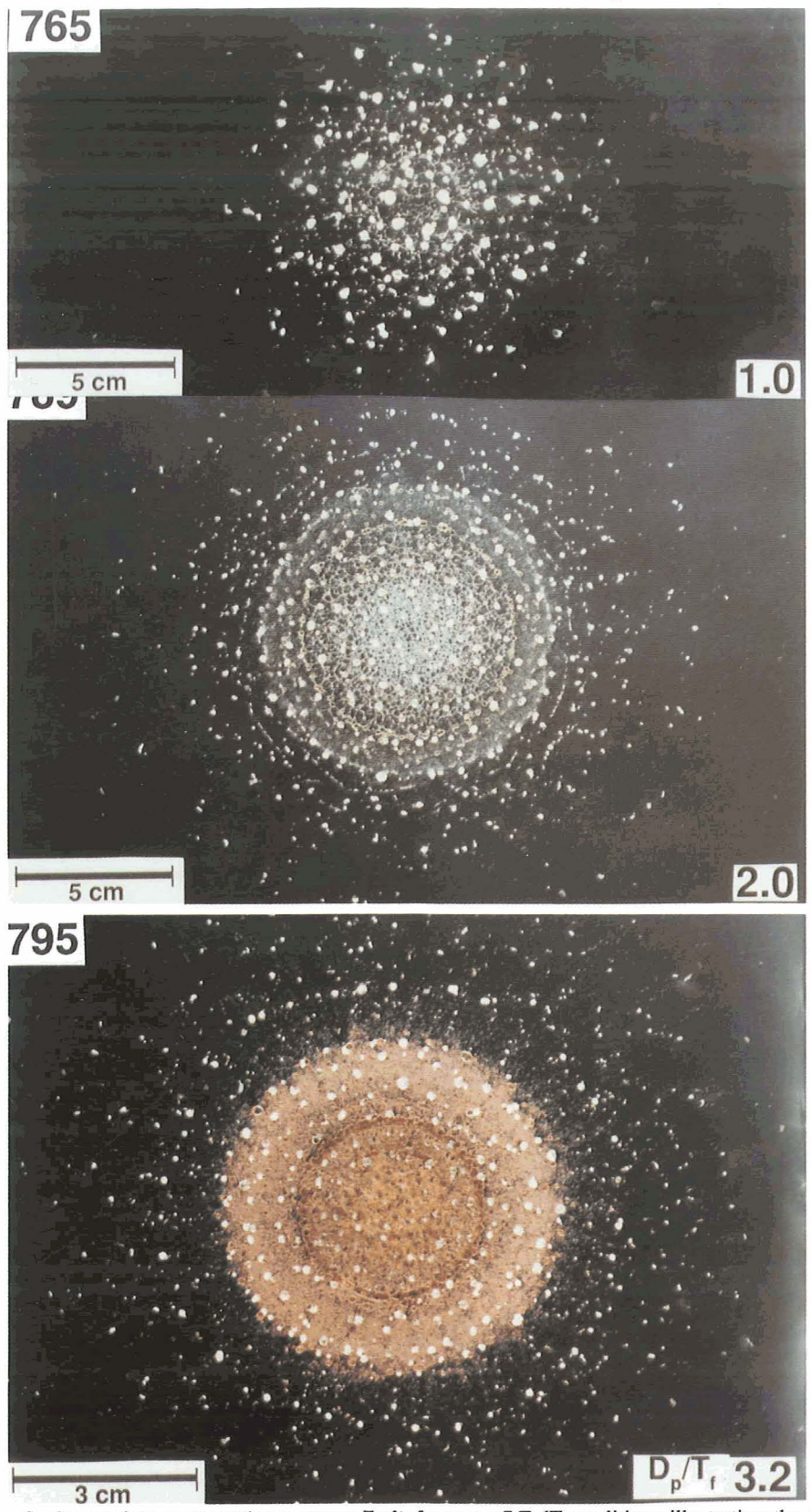
Figure 15e. Details of witness-plate spray patterns over a limited range of D_p/T conditions illustrating the formation of the spider-web patterns (described in the text) resulting from projectile melts at D_p/T = 1 , and the formation of hole-saw ring patterns at D_p/T = 2 ; the D_p/T = 3.175 case employed a copper witness plate to increase visualization of projectile melts (Cu-colored craters), the massive hole-saw ring, and target debris (light-colored craters outside of the major hole-saw ring).
