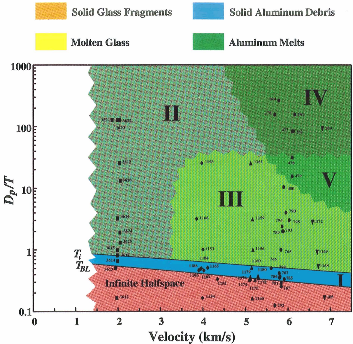
Figure 18. Physical state ( i.e. , molten or solid) of soda-lime glass projectiles and aluminum 1100 target materials composing the exit cloud of penetrated targets at impact velocities of 2 to 7 km/s. No projectile material exits the penetrated target until target thickness becomes thinner than T_i ; depending on the absolute impact velocity and associated peak shock stresses, this material may either be solid (at V < 4 km/s) or molten. The transition from molten to solid projectile species, as portrayed in this figure, is substantially intuitive, yet only solids will result from collisions with ultra-thin targets of \sim D_p/T > 50 , which display substantial central-cluster depressions, if not pitted craters. By the same token, most target mass dislodged from massive targets is solid at all velocities, because most mass dislodged is not shocked beyond the solid/liquid phase transition. Witness-plate evidence for target melt in the form of radial streaks is observed only at V > 5 km/s and D_p/T > 10 . Although the boundaries for these PT states are somewhat intuitive, the important point of this figure is that the PT states of both projectile and target material in a given exit plume depend sensitively and systematically on D_p/T at constant impact velocity.
