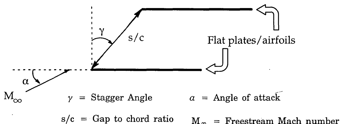
Figure 7.1 Schematic of a typical cascade
