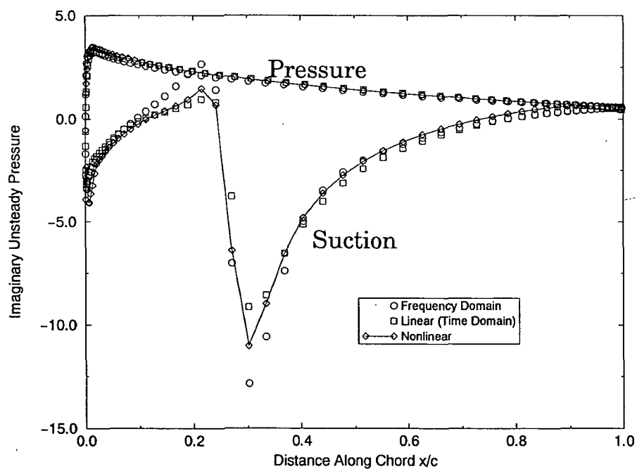
Figure 7.10 Imaginary part of unsteady pressure distribution on transonic 10th std. cfig. due to plunging motion ( \kappa=0.6435 , \sigma=-90^\circ )
