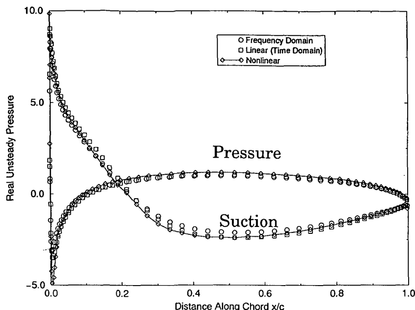
Figure 7.6 Real part of unsteady pressure distribution on subsonic 10th std. cdf. due to plunging motion ( \kappa=0.6435 , \sigma=-90^\circ )
