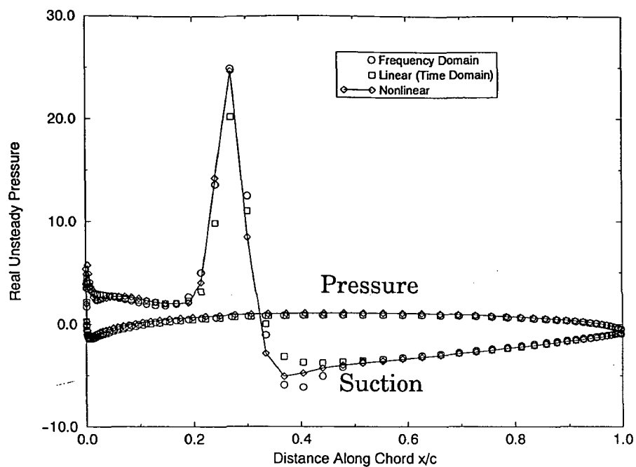
Figure 7.9 Real part of unsteady pressure distribution on transonic 10th std. cfig. due to plunging motion ( \kappa=0.6435 , \sigma=-90^\circ )
