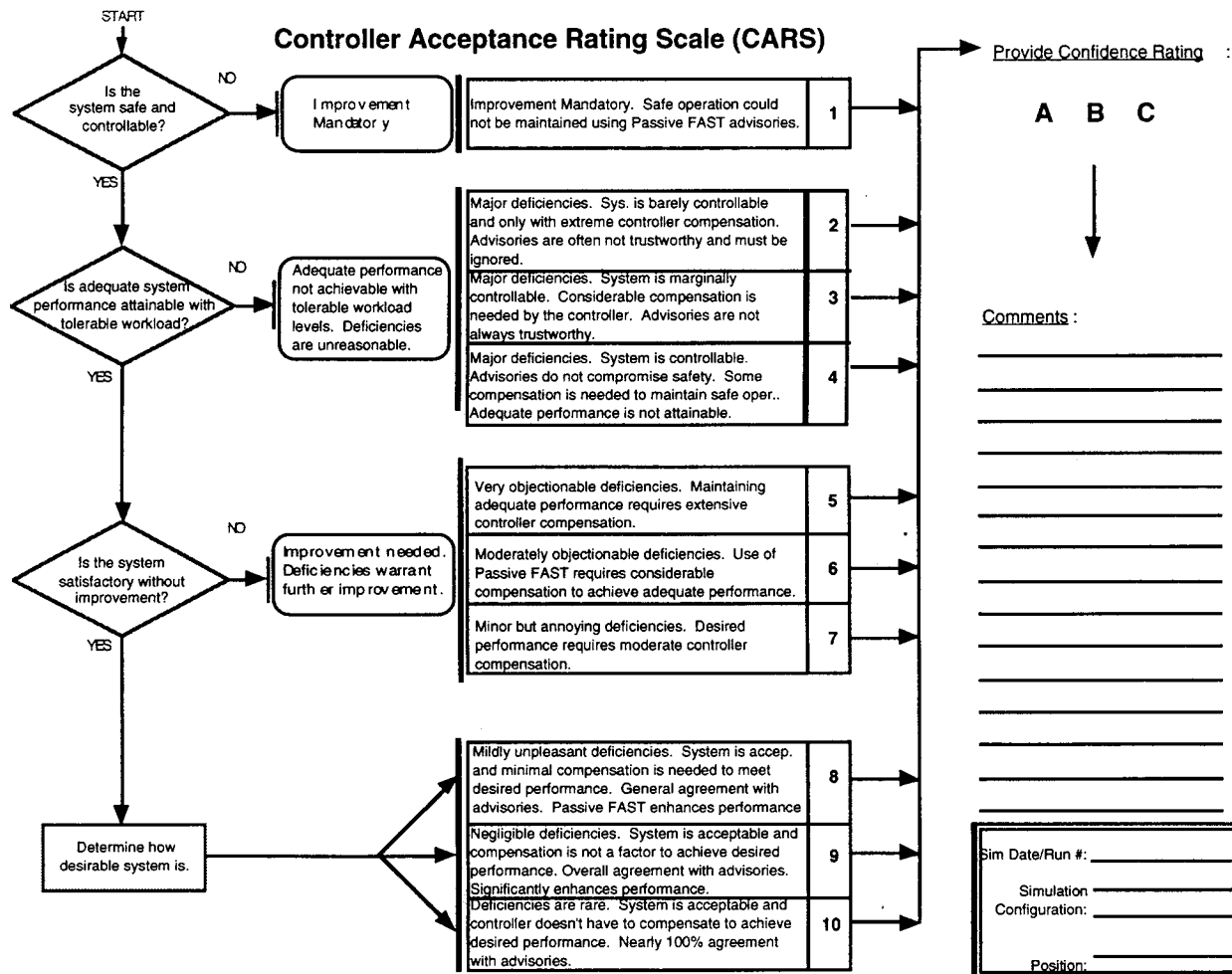
Figure 7. Controller acceptance rating.
