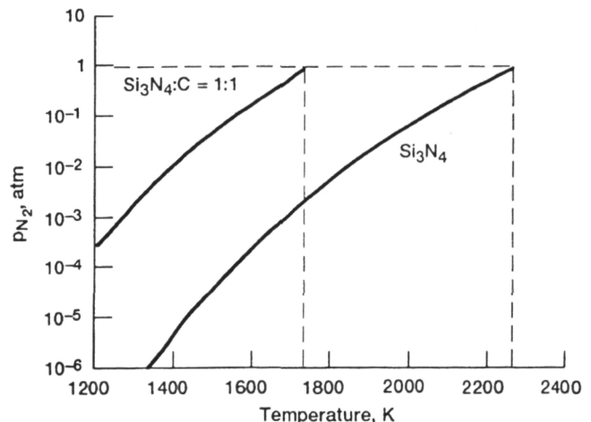
Fig. 1. Calculated pressure of N 2 (g) for Si 3 N 4 and the carbon/Si 3 N 4 system.
