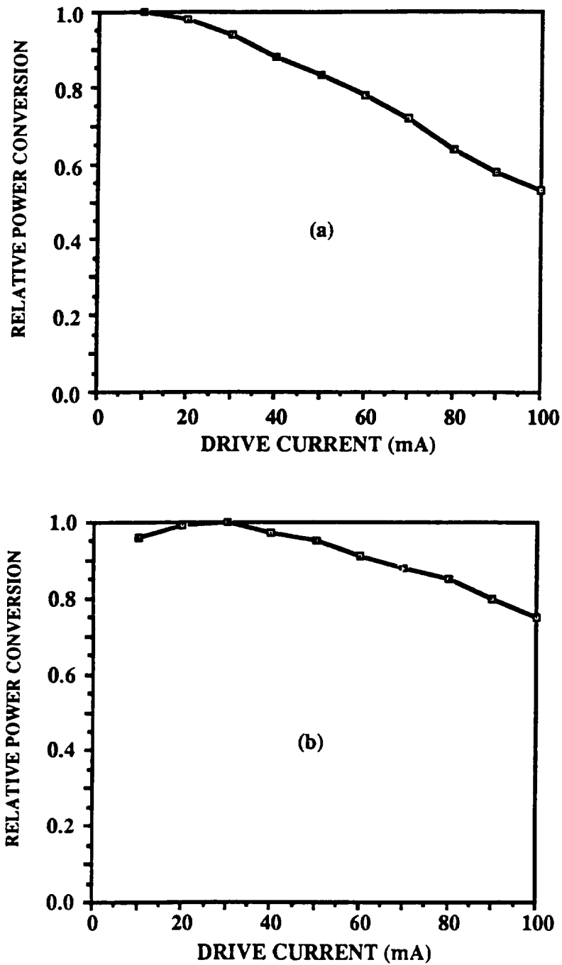
Fig. 1. Relative power conversion of a GaAlAs LED, with a peak emission at 670 nm (a) LED encapsulated in epoxy resin,(b) LED mounted on a proprietary heat dissipation device. (Data from Quantum Devices, Inc.)
