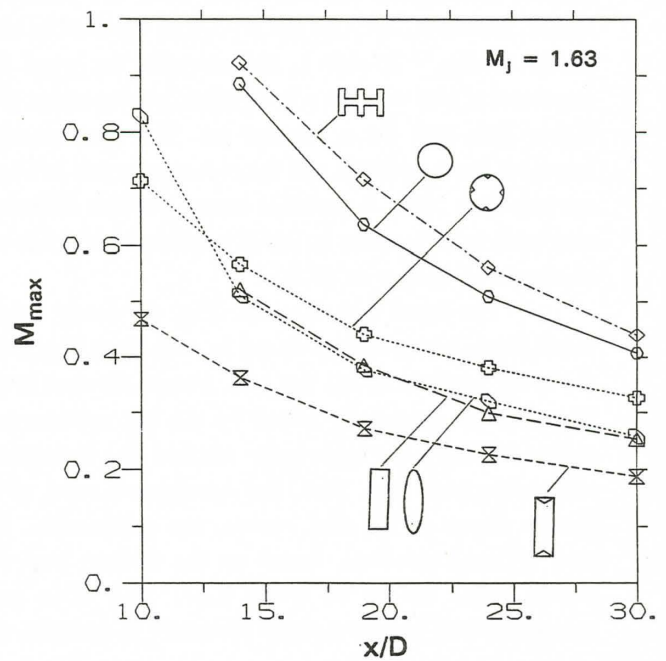
Fig. 5 For M_1 = 1.63 , streamwise variations of maximum Mach number for the six cases.
