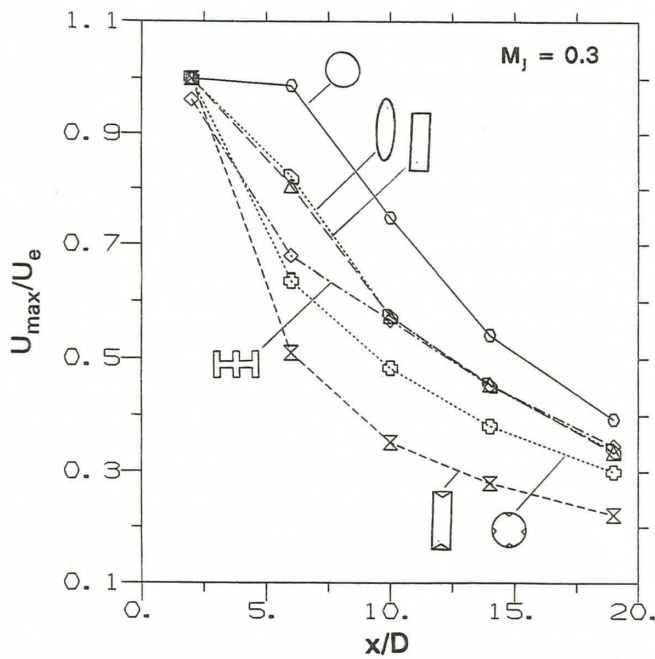
Fig. 4 For M_1 = 0.3 , streamwise variations of maximum mean velocity for the six cases.
