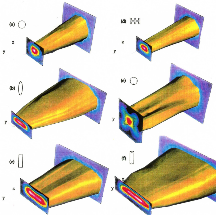
Fig. 3 For M_1 = 1.63 , iso-surfaces of Mach number, M/M_{MAX} = 0.3 , for the six cases. Data cover x/D range of 14-30 in (a), (c) and (d), and 10-30 in the rest of the cases. Co-ordinate origin is at x/D = 8 .
