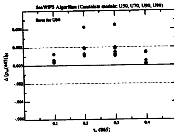
Figure 2b. \Delta[\rho_w(443)]_N as a function of \tau_a(865) for the U80 model, when the candidate aerosol models in the multiple-scattering algorithm are restricted to U50, U70, U90, and U99.
