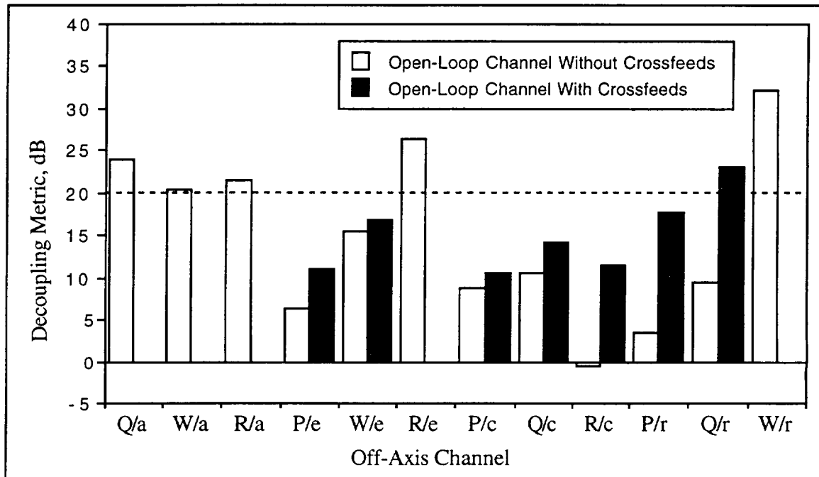
Figure 5. Decoupling Performance Metrics of Compensated System
