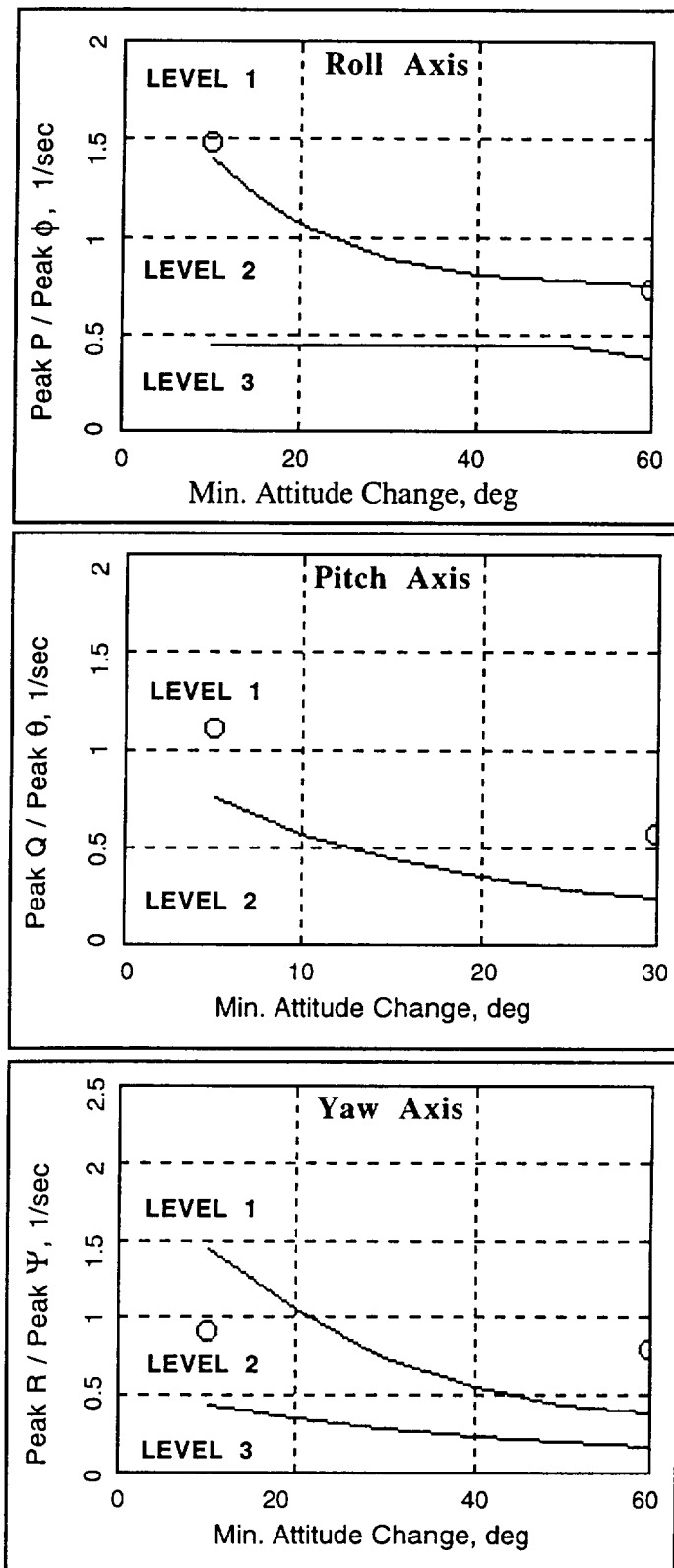
Figure 14. Requirements for Moderate- & Large-Amplitude Attitude Changes.
