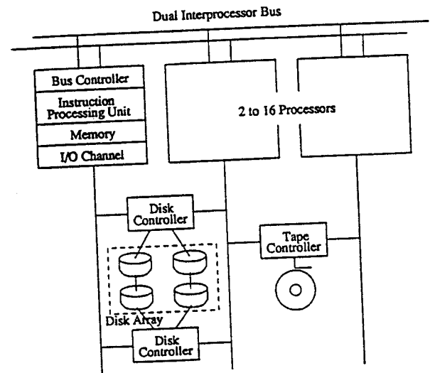
Fig. 1. Tandem GUARDIAN system architecture.
