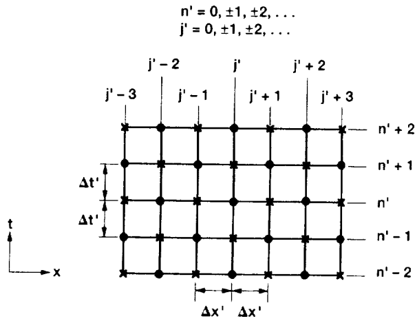
FIG. 18. A regular space-time mesh.
