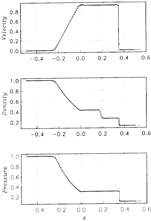
FIG. 12. The Euler solution ( b = 0.5, \alpha = 1, \Delta t = 0.004, CFL \approx 0.88 ).
