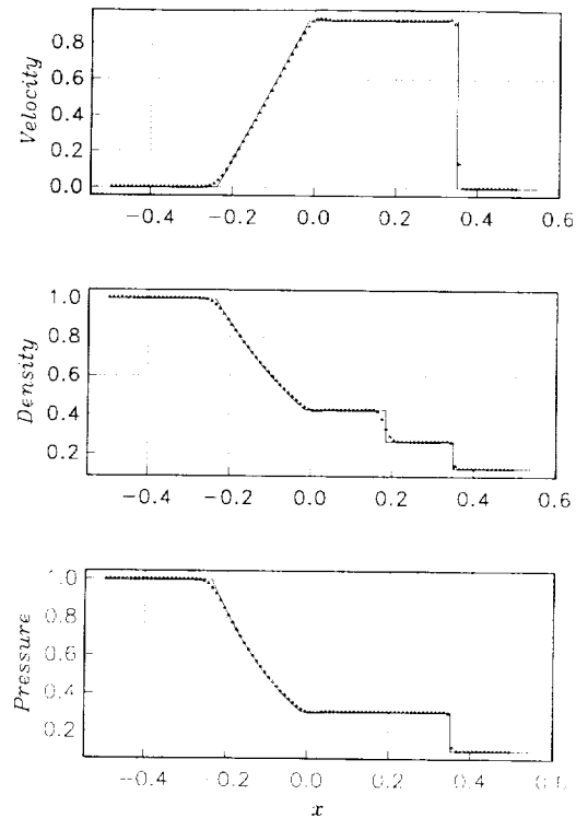
FIG. 7. The Euler solution ( \epsilon = 0.5 , \alpha = 1 , \Delta t = 0.004 , CFL \doteq 0.88 ).
