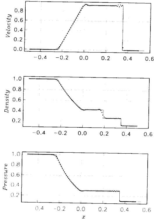
FIG. 6. The Euler solution ( \epsilon = 0.5 , \alpha = 0 , \Delta t = 0.004 , CFL \doteq 0.88 ).
