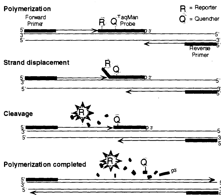
Figure 4-1. Taq DNA polymerase activity in TaqMan PCR. In a single cycle of PCR, the initial steps are template denaturation and annealing of that denatured DNA template with the forward and reverse primers, as well as the tagged TaqMan probe(both steps not depicted). After which, the enzyme's polymerization dependent 5'-3' endonuclease activity frees the reporter dye from the neighbor effects of the quencher dye, so it can produce a signal that is proportional to the PCR amplification. Cleavage of the TaqMan probe does not affect forward primer extension. (Modified from TaqMan™ Reagent Kit Protocol, Perkin Elmer/Applied Biosystems). 9
