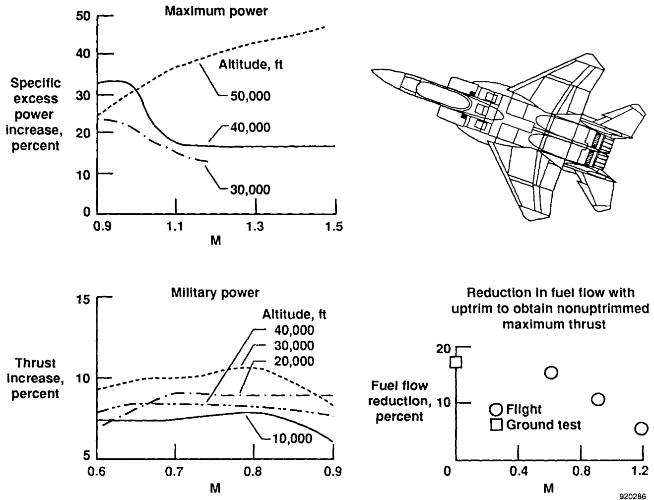
Figure 33. Propulsion-efficiency benefits provided by HIDEDEC modifications to the F-15 airplane.
