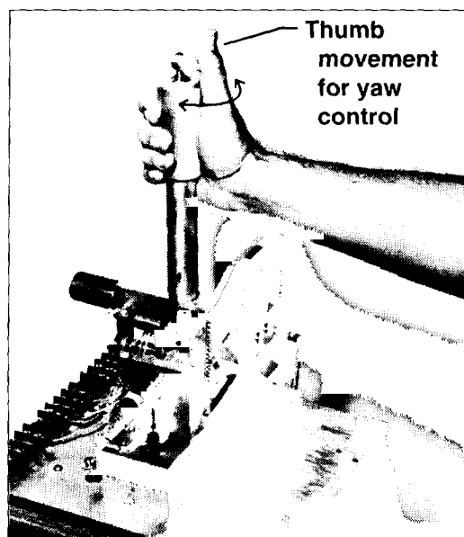
Three axis control stick
