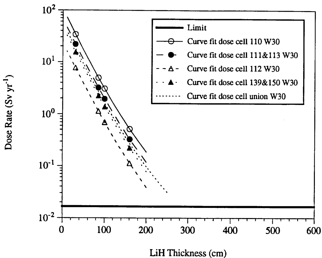
Figure D.c Curve fit of the photon dose rates inside the six crew compartments due to one SP-100 reactor neutron interactions through the shield with a 30-cm thick tungsten layer and a variable lithium hydride thickness.
