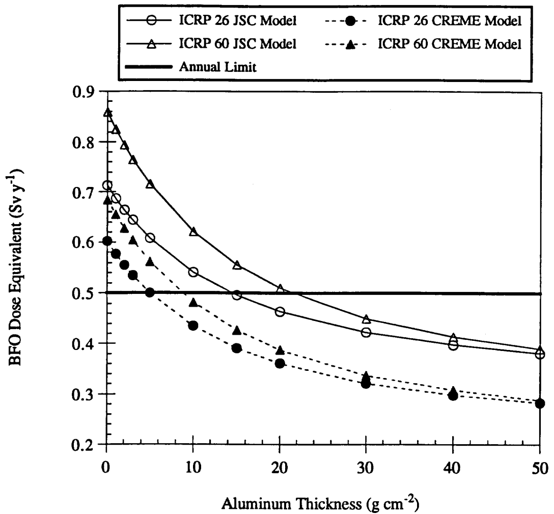
Figure 2.4 Influence of the quality factor variations between ICRP Publication 26 and ICRP Publication 60 on the BFO dose equivalent from GCR as a function of shielding thickness for solar minimum. Calculations performed using the 1976-1977 GCR spectra of Badhwar and O'Neill (1992) and the CREME model.
