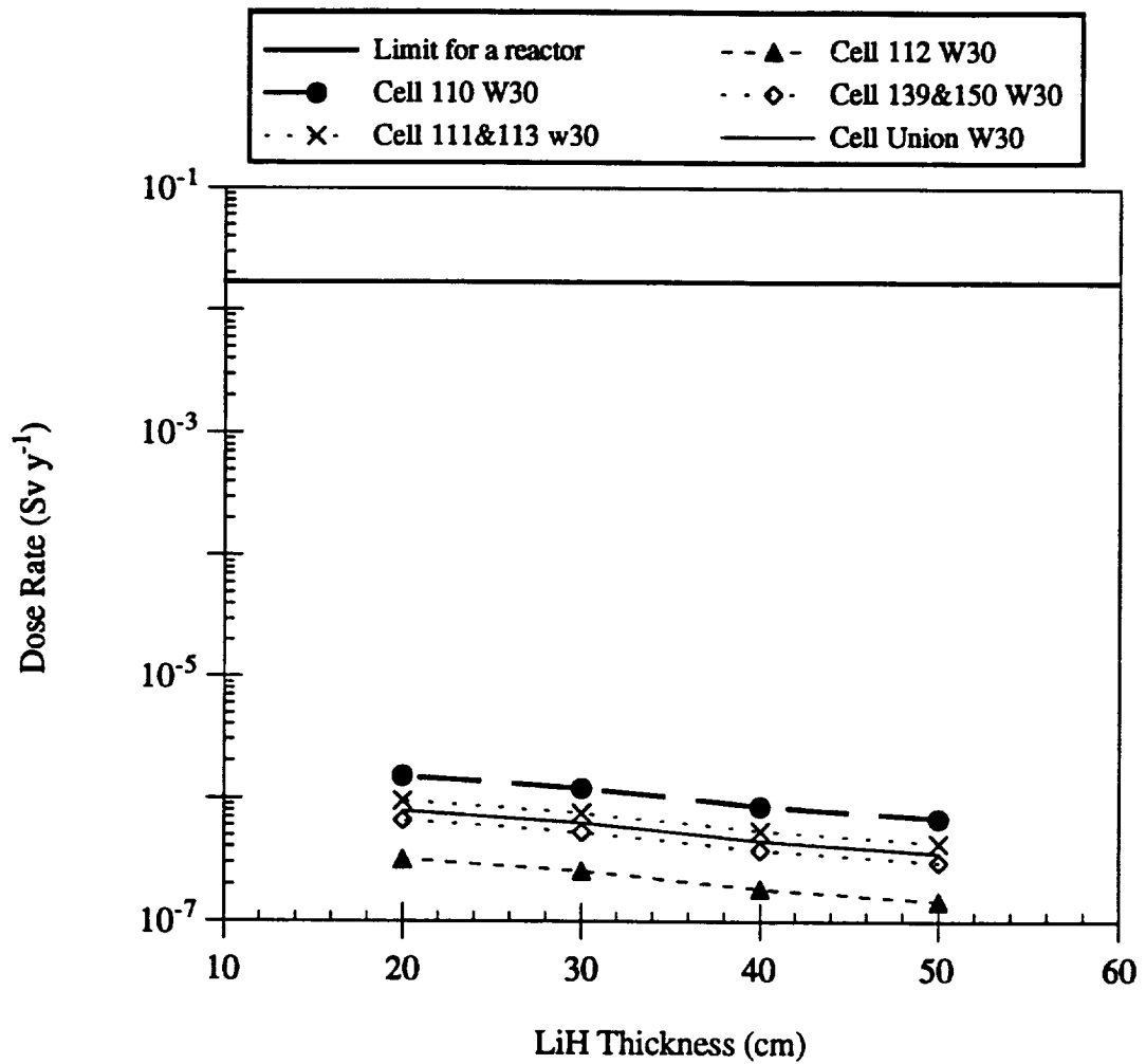
Figure 5.7 Photon dose rates inside the six crew compartments due to the photon source of one SP-100 reactor with a 30-cm thick tungsten layer and a variable lithium hydride thickness.
