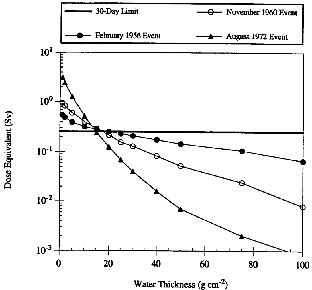
Figure 2.5 Depth-dose equivalent (Sv) in tissue (5 cm depth) as a function of water shield thickness for three Anomalous Large Solar Particle Events. (1 g cm -2 of water is equivalent to a thickness of 1 cm of aluminum).
