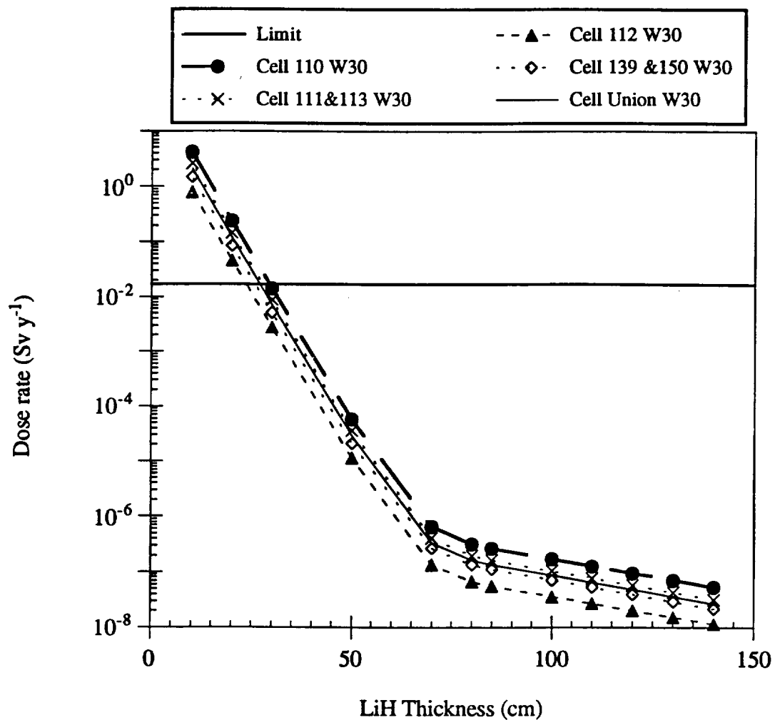
Figure 5.13 Total dose rates inside the crew compartment from the neutrons and photons created from one SP-100 reactor with a 30-cm thick tungsten layer and a variable lithium hydride thickness.
