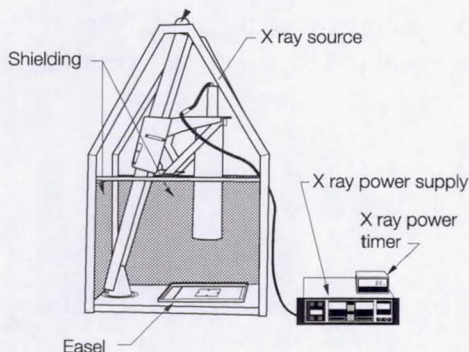
Figure 3: X-ray device
