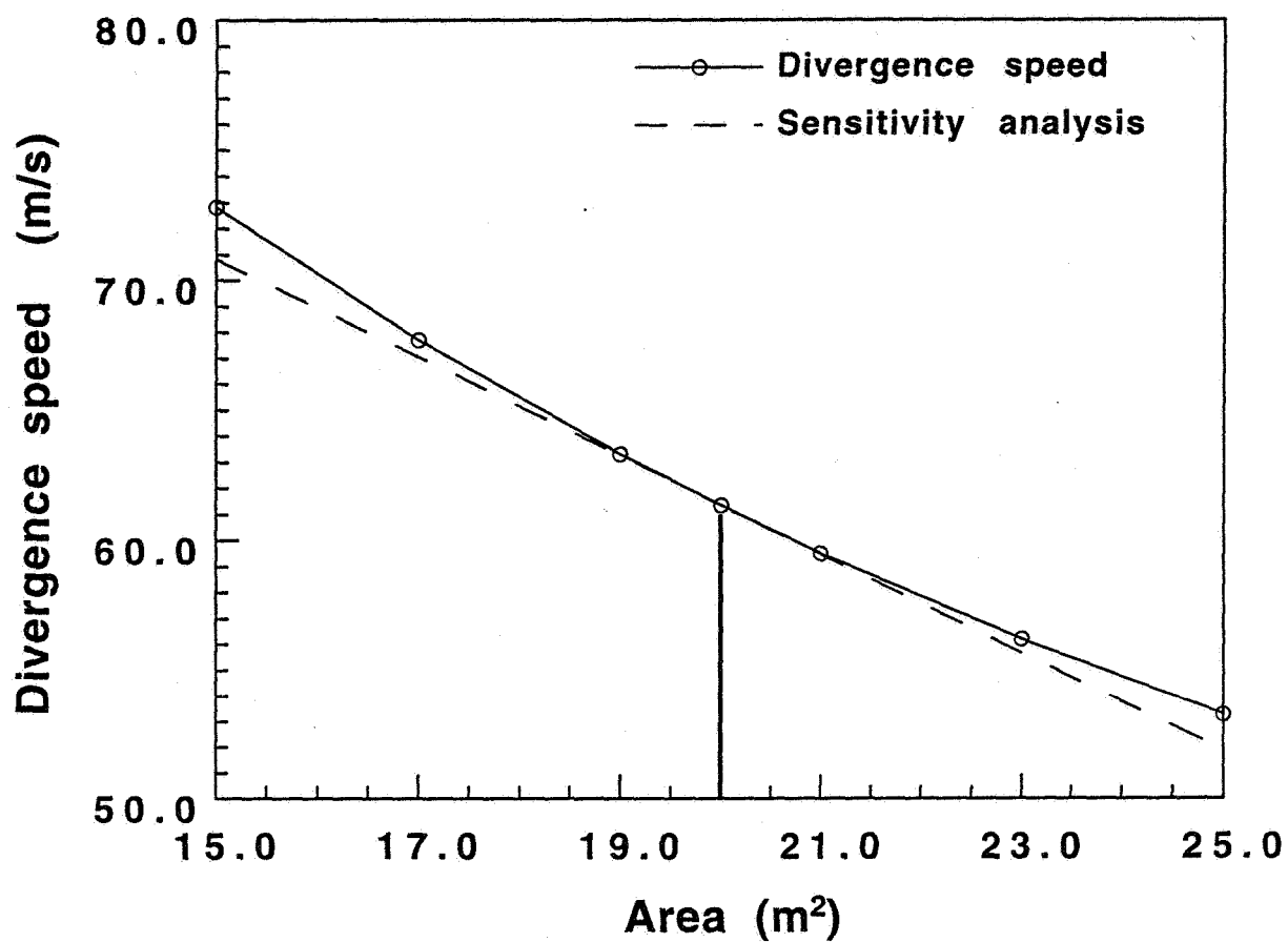
Fig. 3.13 Divergence speed vs Area ( M=0.7 ) ( AR=10 , Area=20m^2 , TR=0.5 , Sweep=0^\circ )
