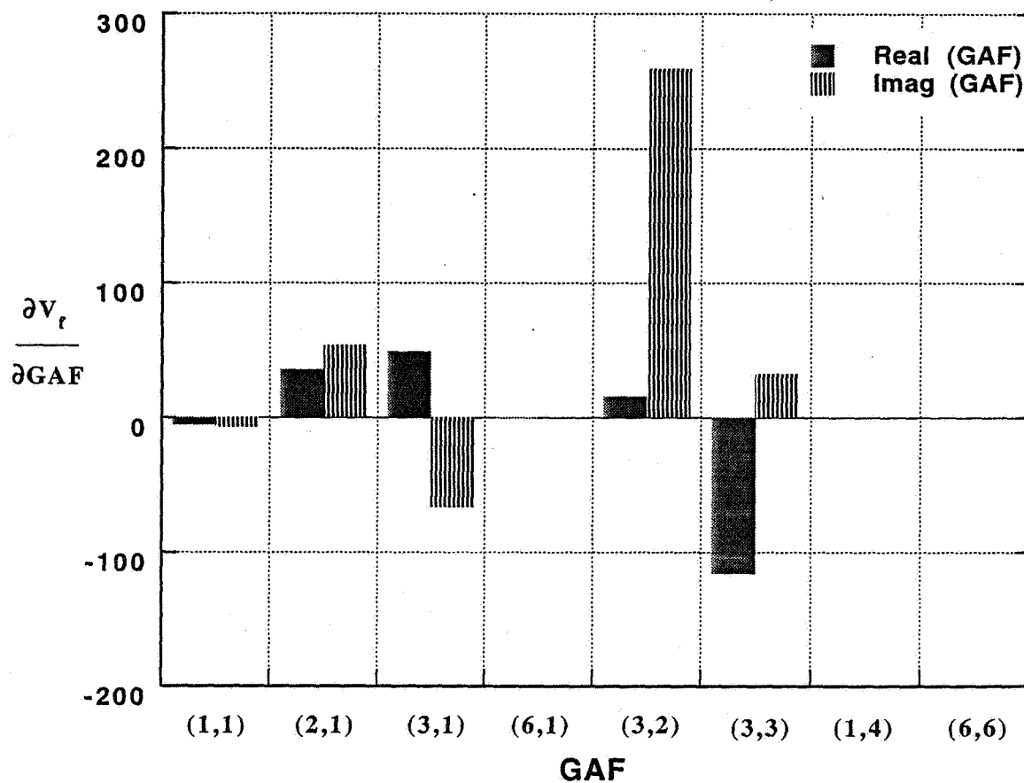
Fig. 5.19 Flutter speed sensitivity to nondimensional generalized aerodynamic forces (GAF) ( M=0.6 ) in (m/s)
