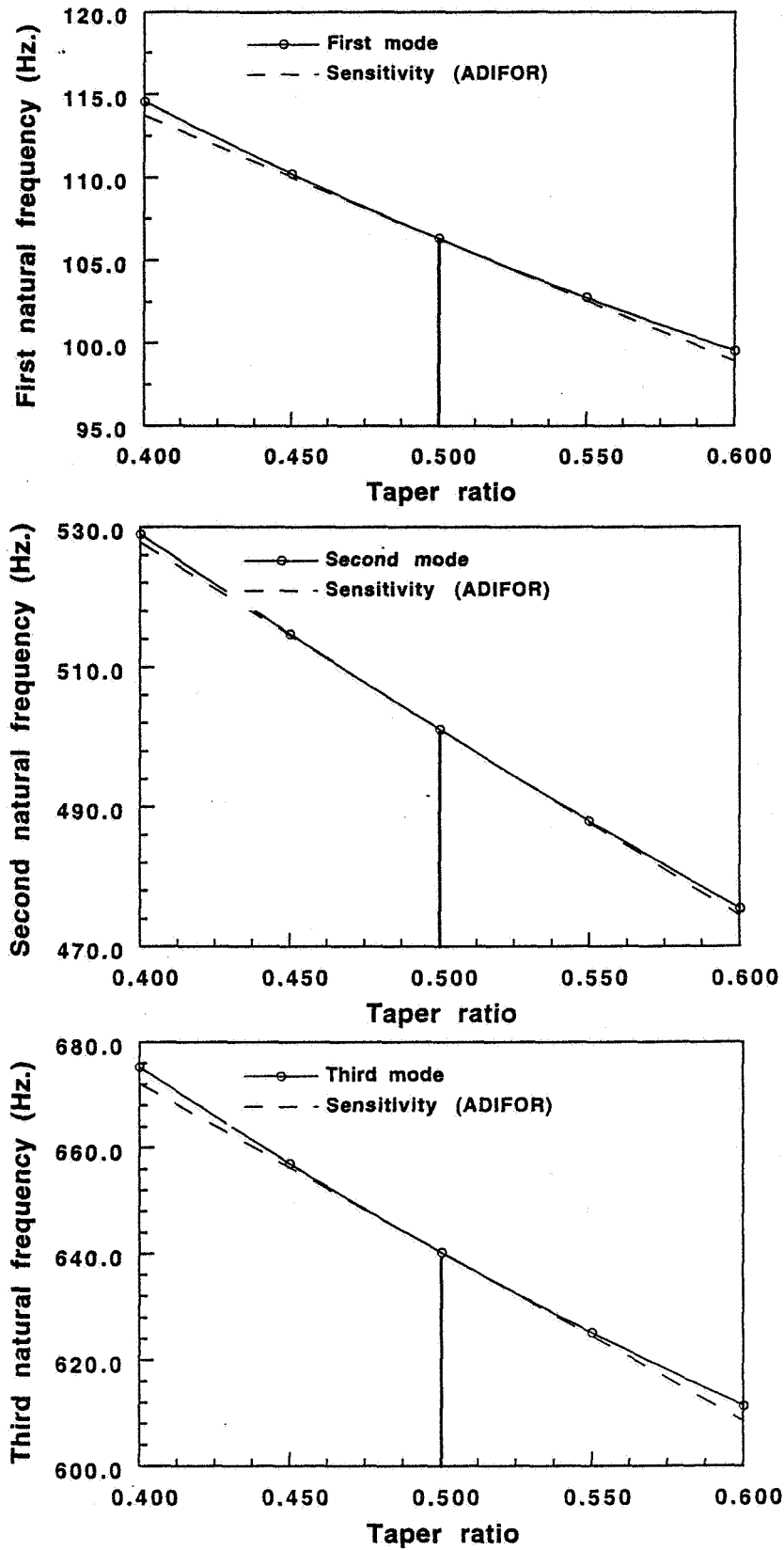
Fig. 6.3 First three natural frequencies vs Taper ratio for a thick plate
