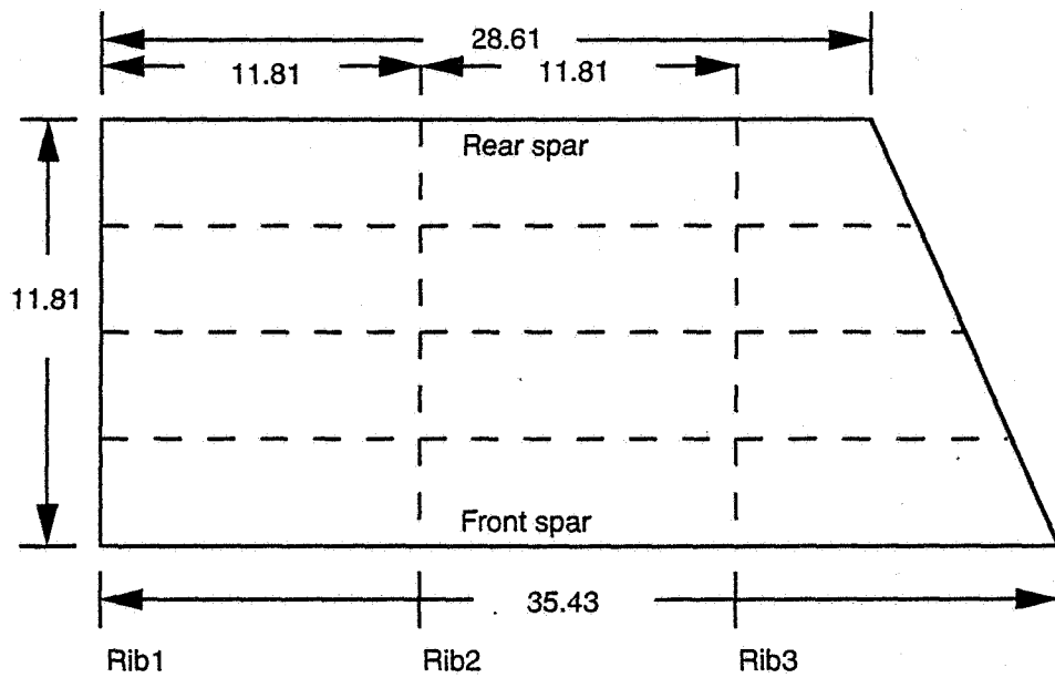
PLANFORM DIMENSIONS
