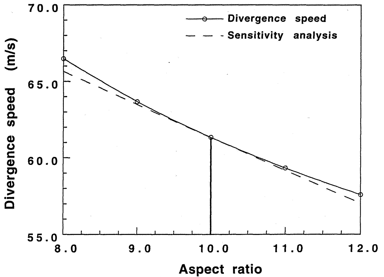
Fig. 3.12 Divergence speed vs Aspect ratio ( M=0.7 ) ( AR=10 , Area=20m^2 , TR=0.5 , Sweep=0^\circ )
