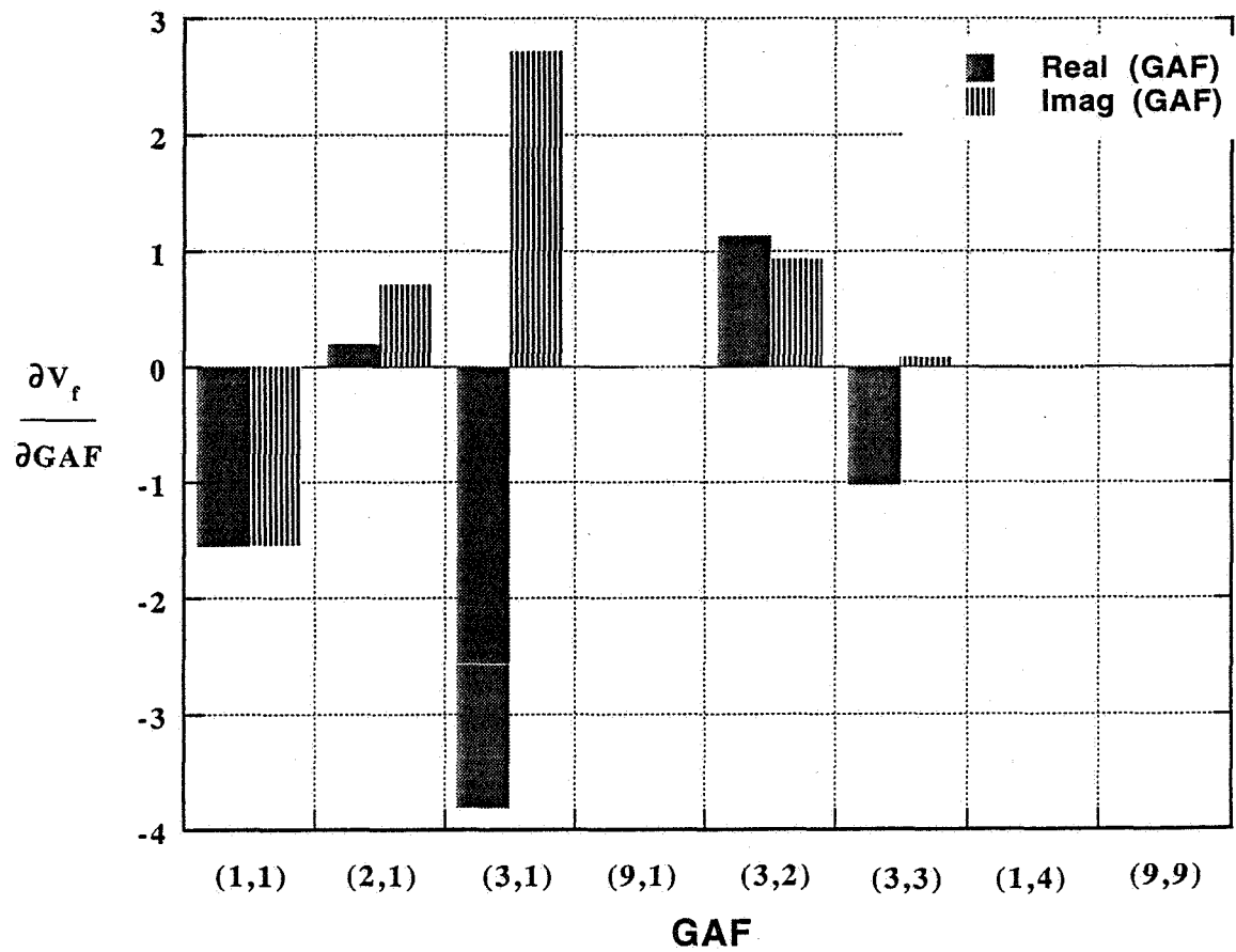
Fig. 4.7 Flutter speed sensitivity to nondimensional generalized aerodynamic forces (GAF) ( M=0.6 ) in (m/s)
