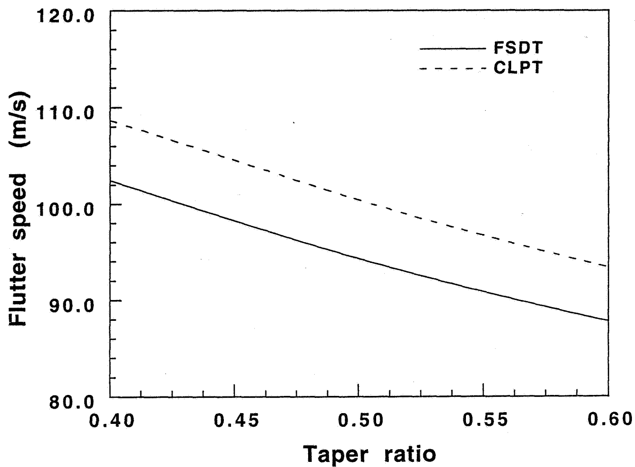
Fig. 6.7 Effect of transverse shear on flutter [Flutter speed vs Taper ratio ( M=0.6 )] ( AR=10 , Area=20m^2 , Sweep=30^\circ )
