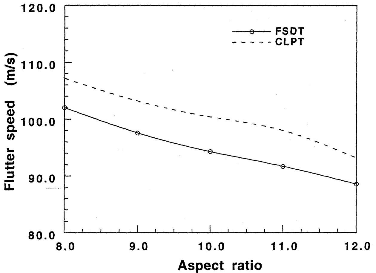
Fig. 6.5 Effect of transverse shear on flutter [Flutter speed vs Aspect ratio ( M=0.6 )] (Area=20m 2 , TR=0.5 , Sweep=30°)
