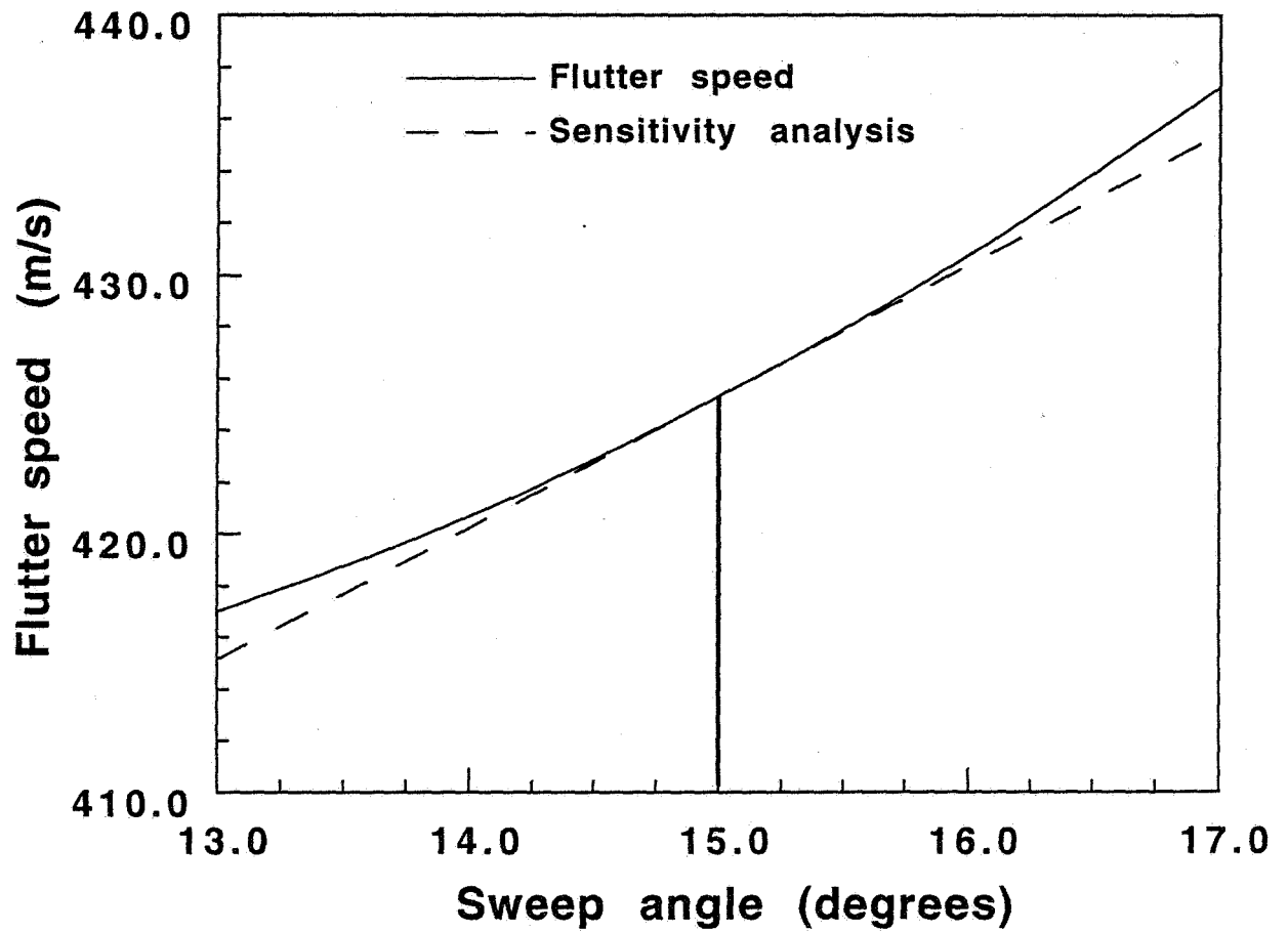
Fig. 5.16 Flutter speed vs Sweep angle ( M=0.6 ) ( AR=3.33 , Area=7.5m^2 , TR=0.5 , Sweep=15^\circ )
