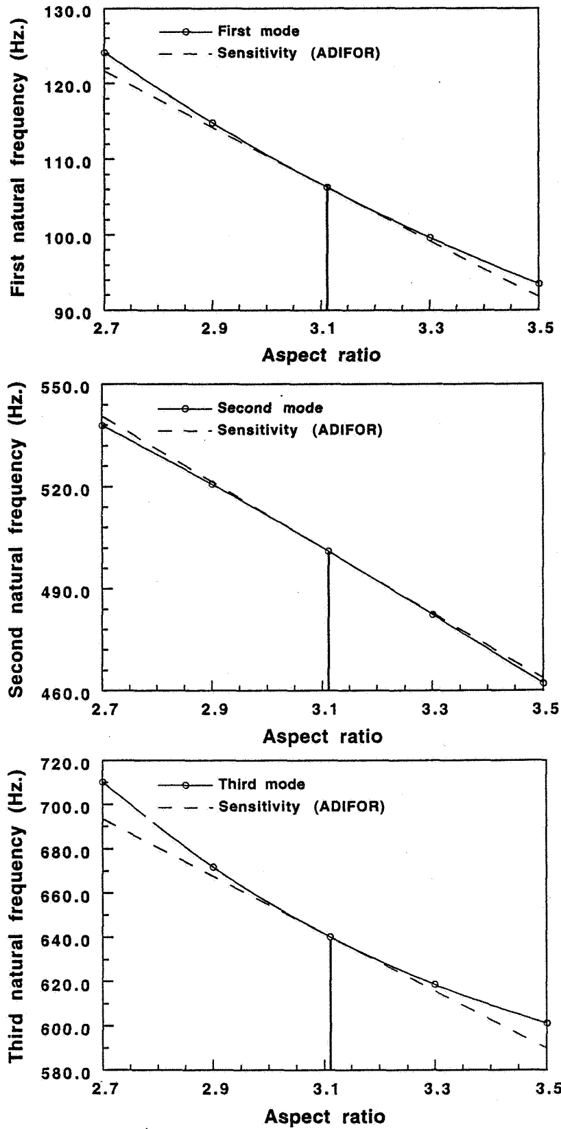
Fig. 6.1 First three natural frequencies vs Aspect ratio for a thick plate
