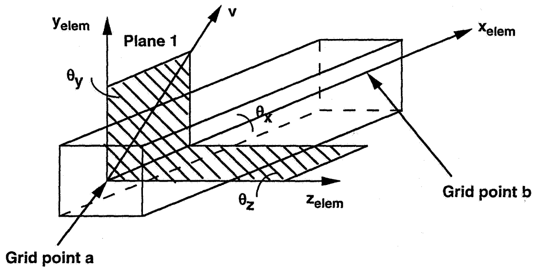
Fig. 5.3 CBAR beam element
