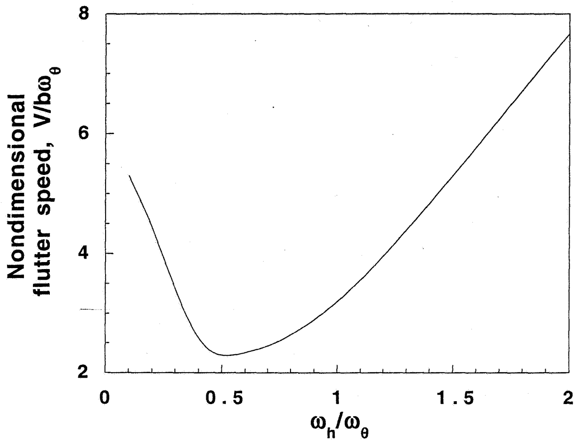
Fig. 2.3 Variation of nondimensional speed, V/b\omega_\theta with ratio of frequencies, \omega_h/\omega_\theta
