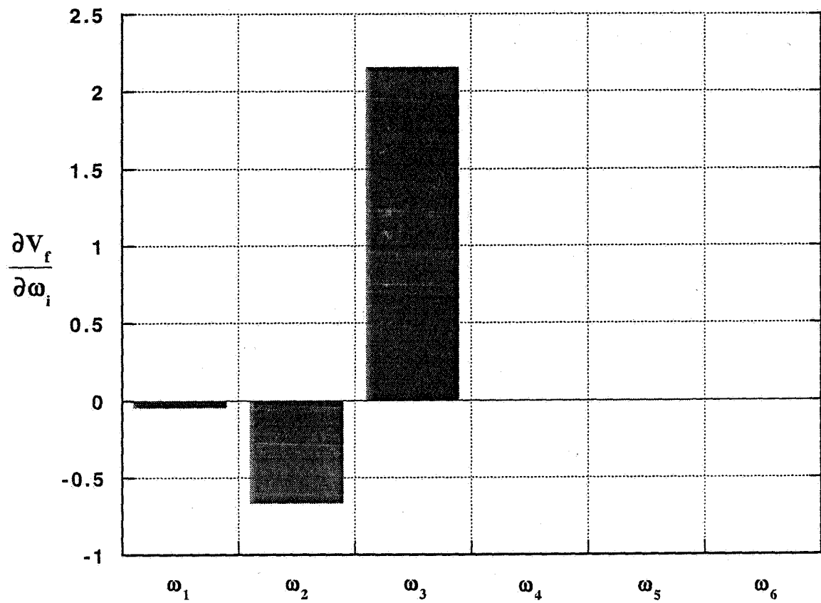
Fig. 5.17 Flutter speed sensitivity to natural frequency ( M=0.6 ) in (m/s)/(rad/s)
