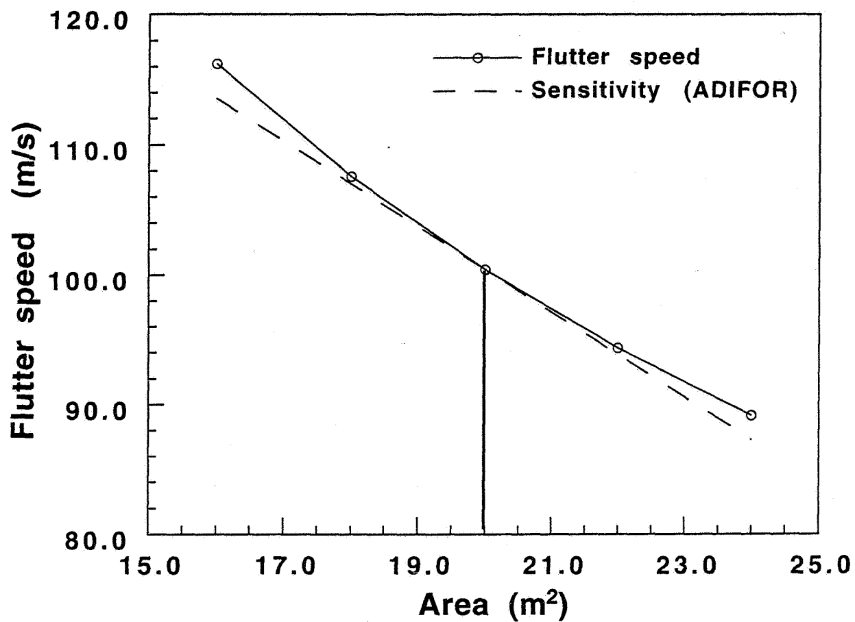
Fig 4.2 Flutter speed Vs Area (M=0.6) from FAST (AR=10, Area=20m², TR=0.5, Sweep=30°)
