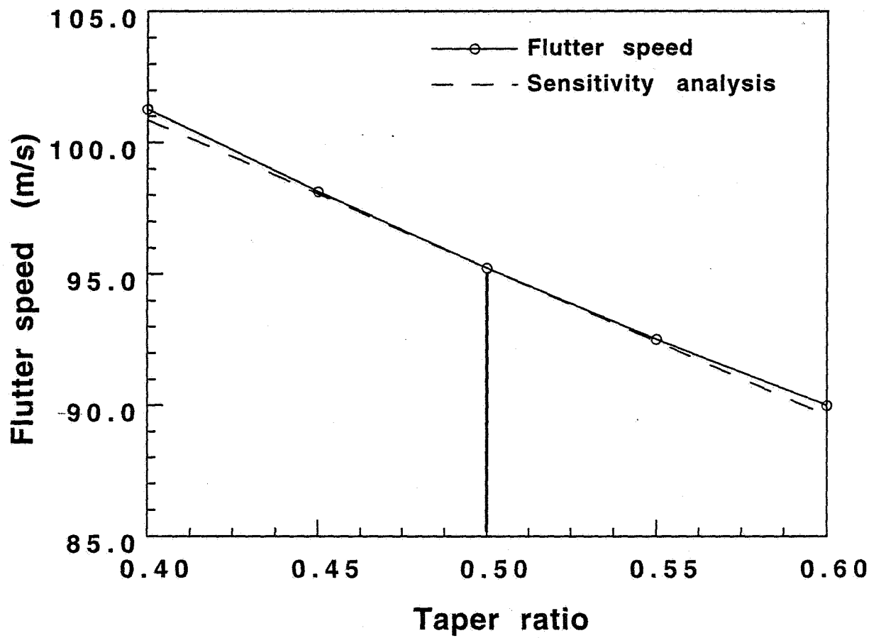
Fig. 3.18 Flutter speed vs Taper ratio ( M=0.7 ) ( AR=10 , Area=20m^2 , TR=0.5 , Sweep=15^\circ )
