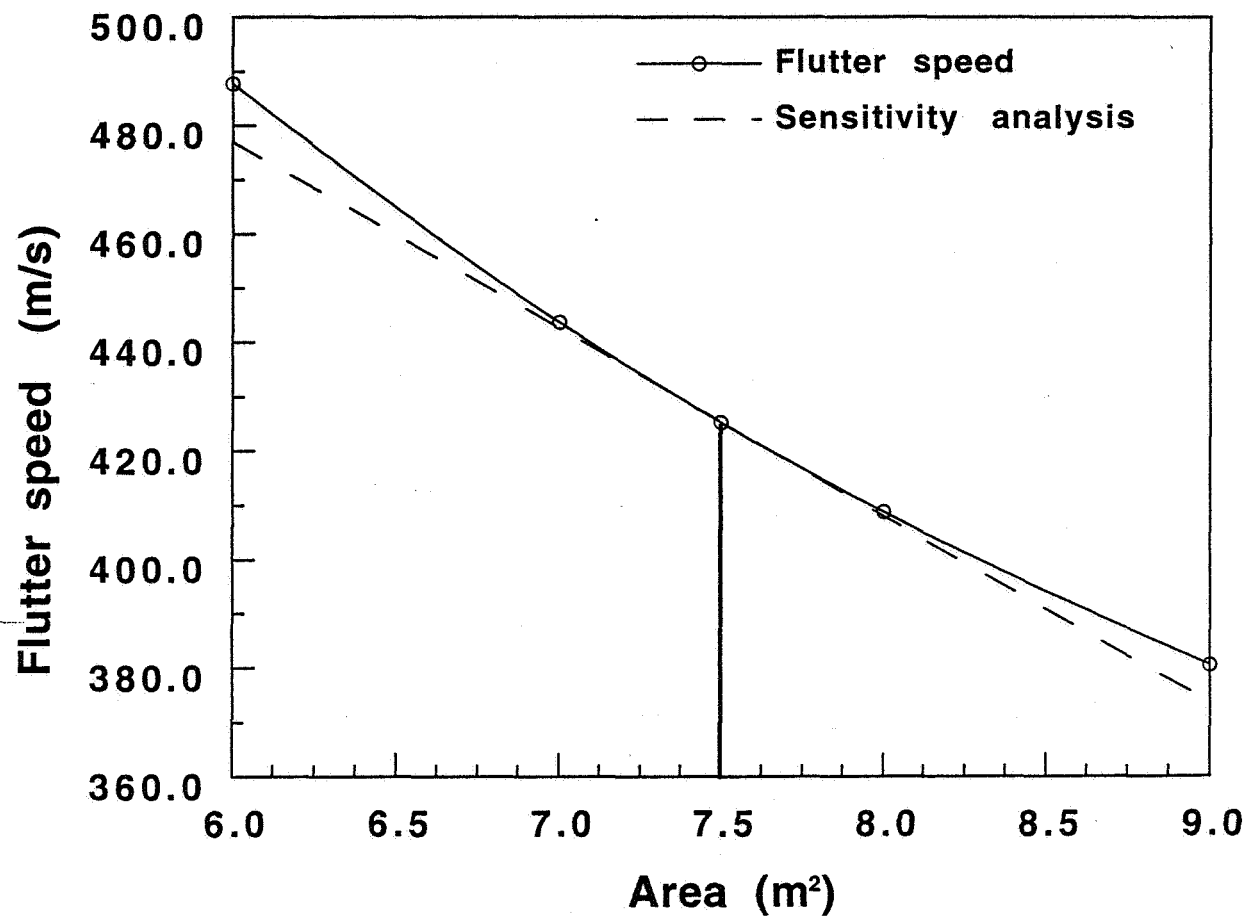
Fig. 5.14 Flutter speed vs Area ( M=0.6 ) ( AR=3.33 , Area=7.5m^2 , TR=0.5 , Sweep=15^\circ )
