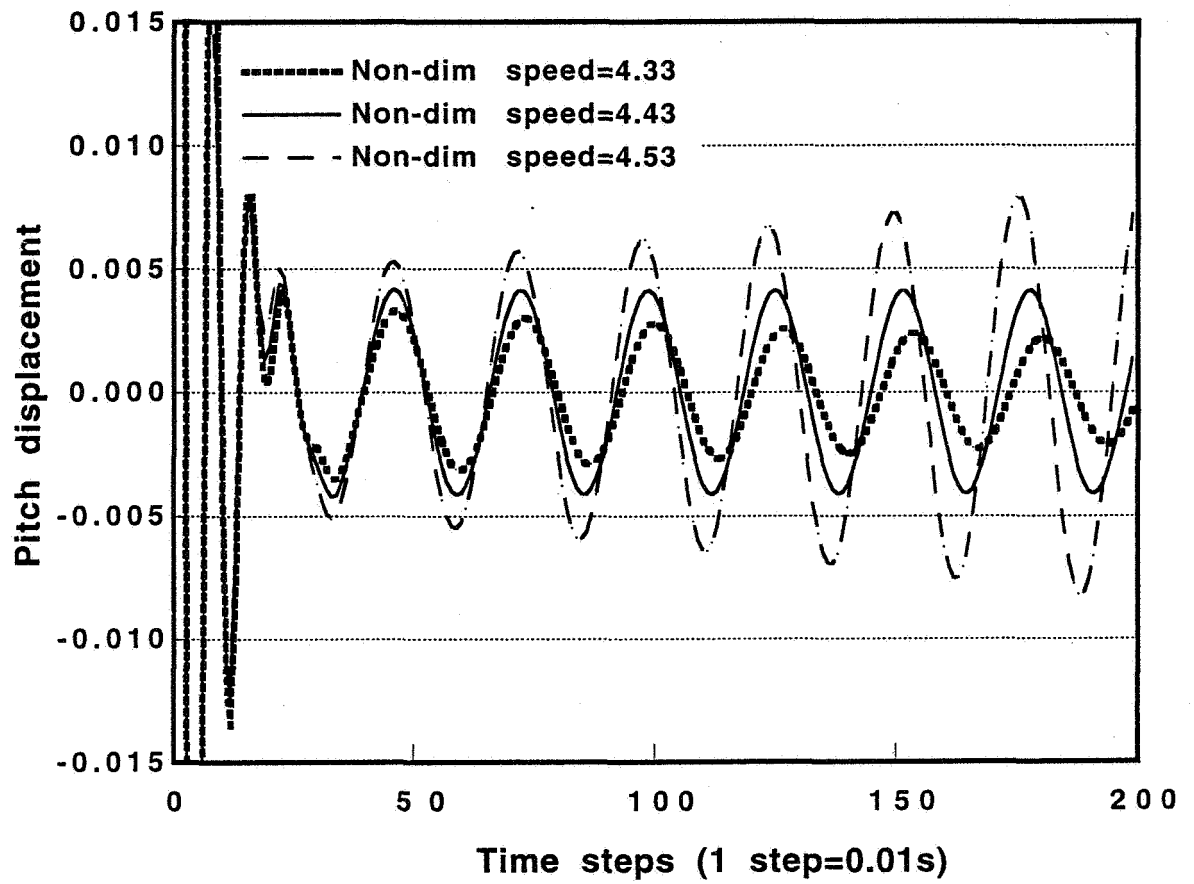
Fig. 2.5 Pitch displacement vs time
