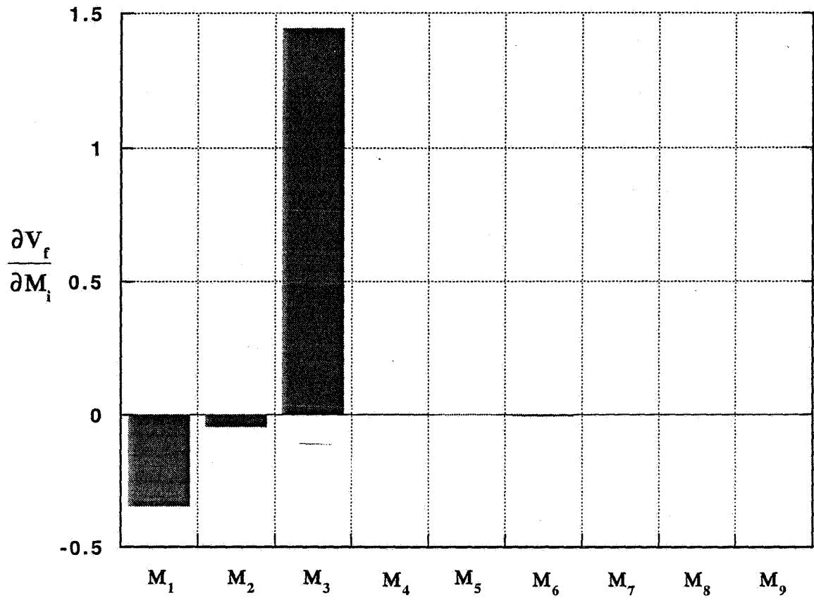
Fig. 4.6 Flutter speed sensitivity to generalized mass ( M=0.6 ) in (m/s)/(kg) ( AR=10 , Area=20m^2 , TR=0.5 , Sweep=30^\circ )
