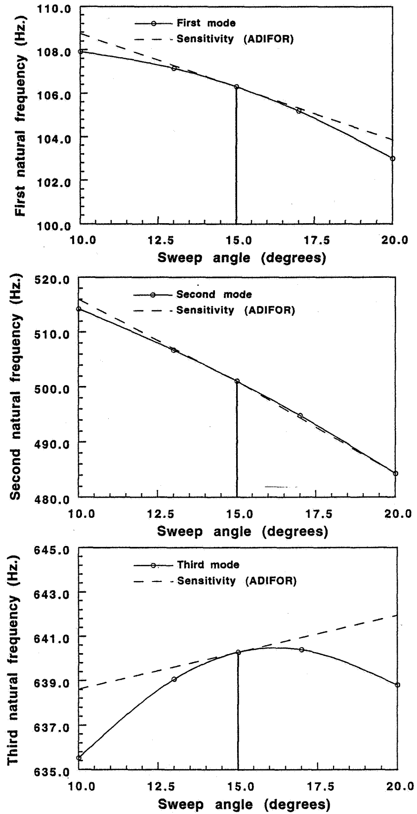
Fig. 6.4 First three natural frequencies vs Sweep angle for a thick plate ( AR=3.111 , Area=0.040645m^2 , TR=0.5 , Sweep=15^\circ )
