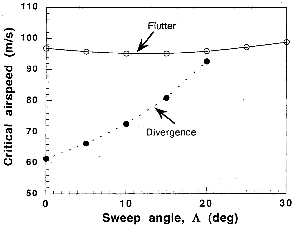
Fig. 3.11 Critical speed vs Sweep Angle ( AR=10 , Area=20 \text{ m}^2 , TR=0.5 )
