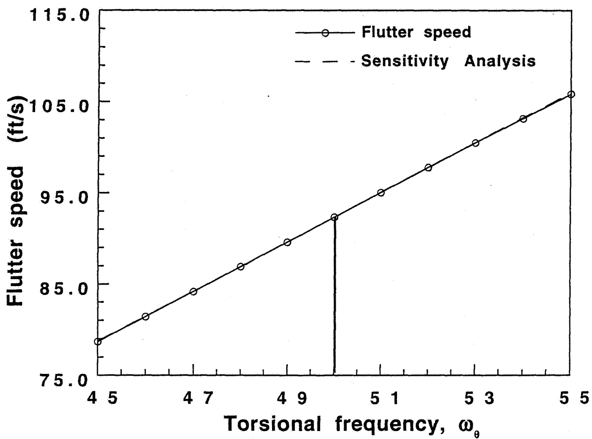
Fig. 2.10 Flutter speed vs Torsional frequency (M=0.85)
