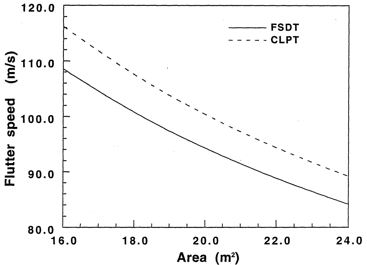
Fig. 6.6 Effect of transverse shear on flutter [Flutter speed Vs Area (M=0.6)] (AR=10, TR=0.5, Sweep=30°)
