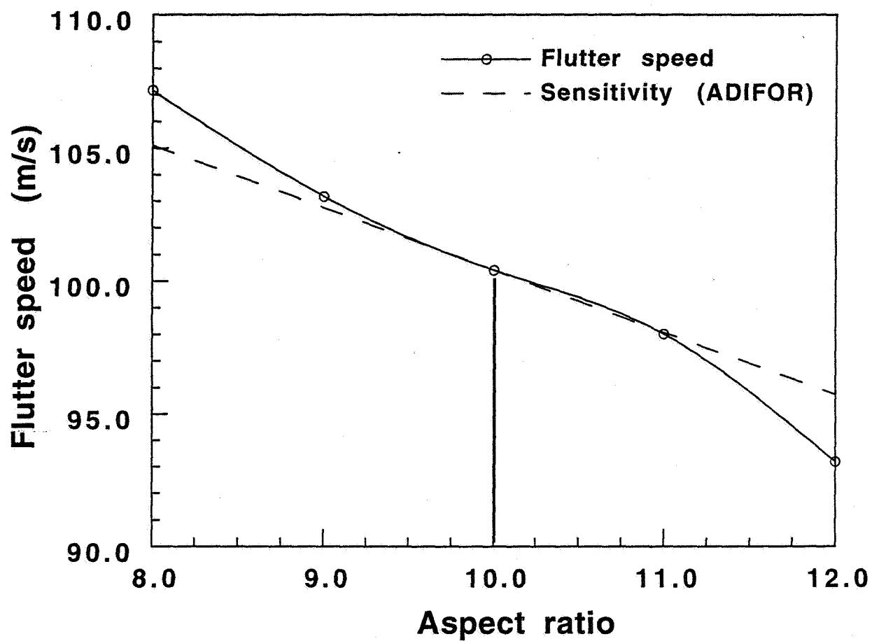
Fig. 4.1 Flutter speed vs Aspect ratio (M=0.6) from FAST
