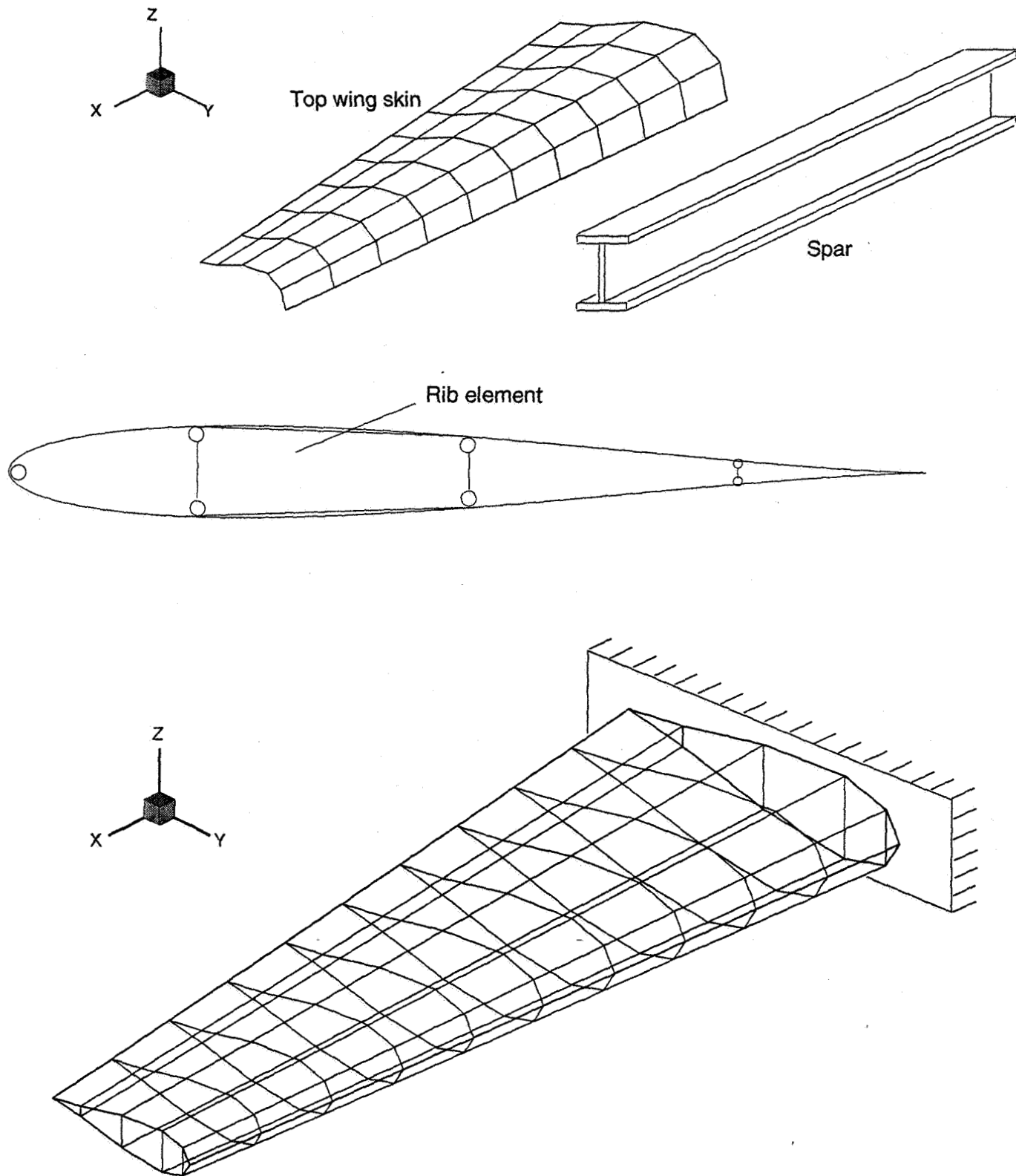
Fig. 5.11 Finite element discretization of the wing
