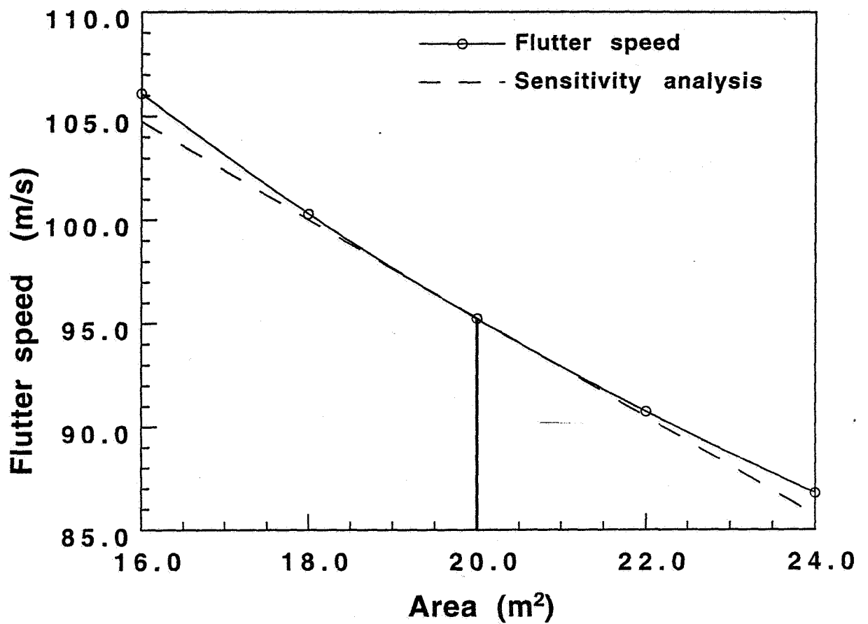
Fig. 3.17 Flutter speed vs Area (M=0.7) (AR=10, Area=20m², TR=0.5, Sweep=15°)
