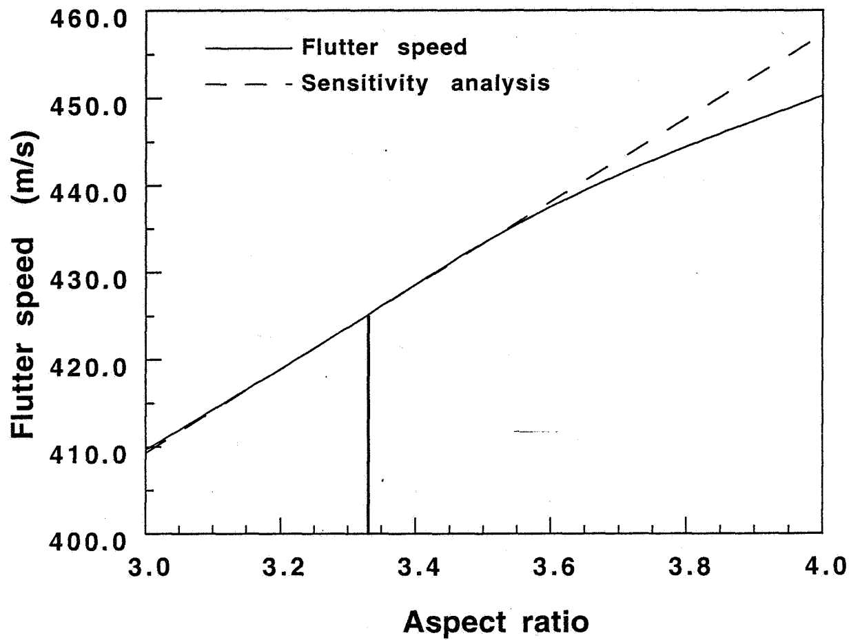
Fig. 5.13 Flutter speed vs Aspect ratio ( M=0.6 ) ( AR=3.33 , Area=7.5m^2 , TR=0.5 , Sweep=15^\circ )
