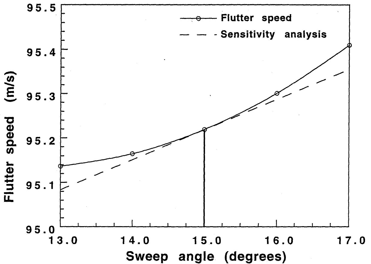
Fig. 3.19 Flutter speed vs Sweep angle ( M=0.7 ) ( AR=10 , Area=20m^2 , TR=0.5 , Sweep=15^\circ )
