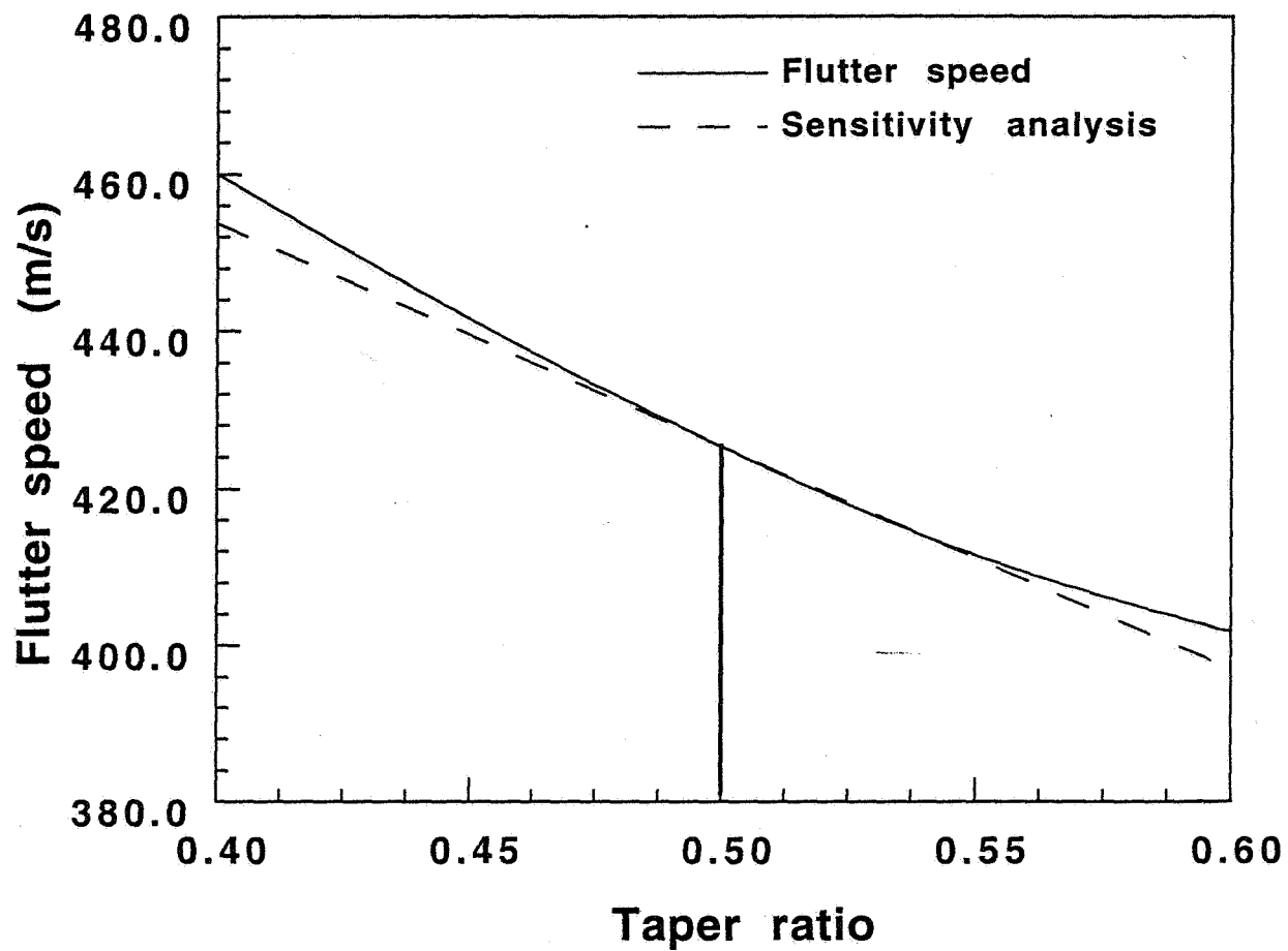
Fig. 5.15 Flutter speed vs Taper ratio ( M=0.6 ) ( AR=3.33 , Area=7.5m^2 , TR=0.5 , Sweep=15^\circ )
