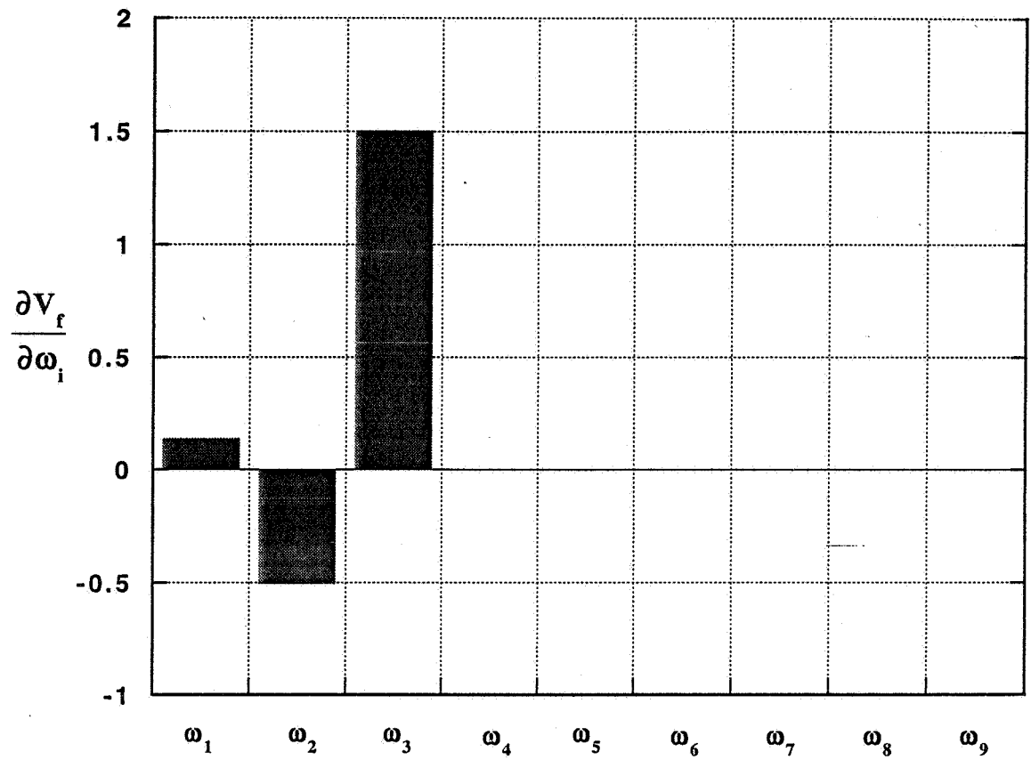
Fig. 4.5 Flutter speed sensitivity to natural frequency (M=0.6) in (m/s)/(rad/s)
