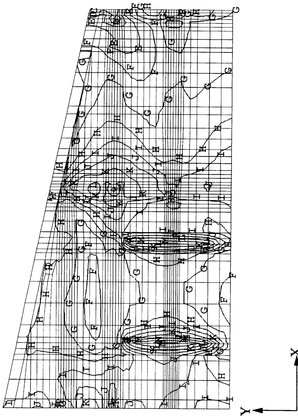
Figure 32. Predicted longitudinal strain contours at skin-side surface of upper cover due to 166,000 lb. tip load.
