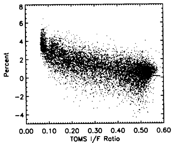
Figure 29. Evidence of signal level dependence in TOMS radiance measurement relative to SBUV. Data are from a five day period in March, 1985.
