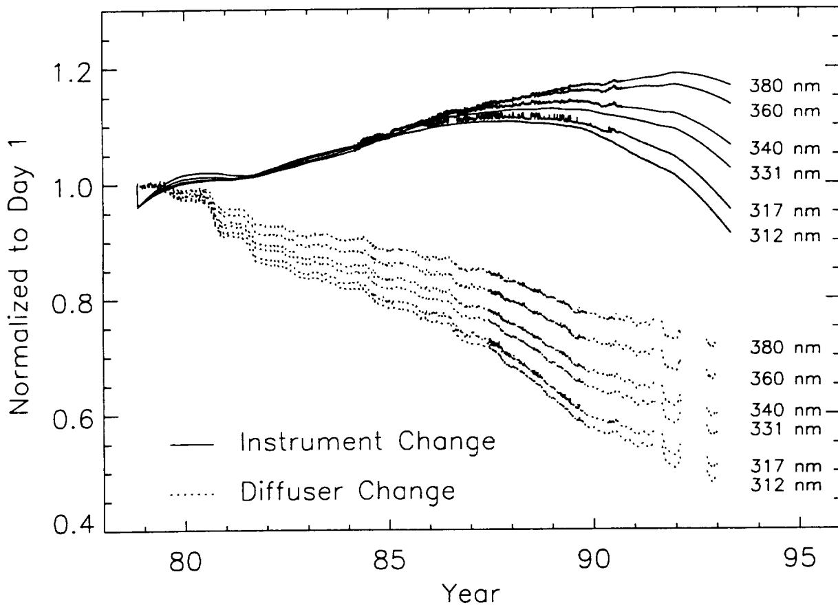
Figure 8. Diffuser and instrument components of the total change exhibited in TOMS “raw” solar flux (Figure 3) as derived using the radiance calibration methods described.
