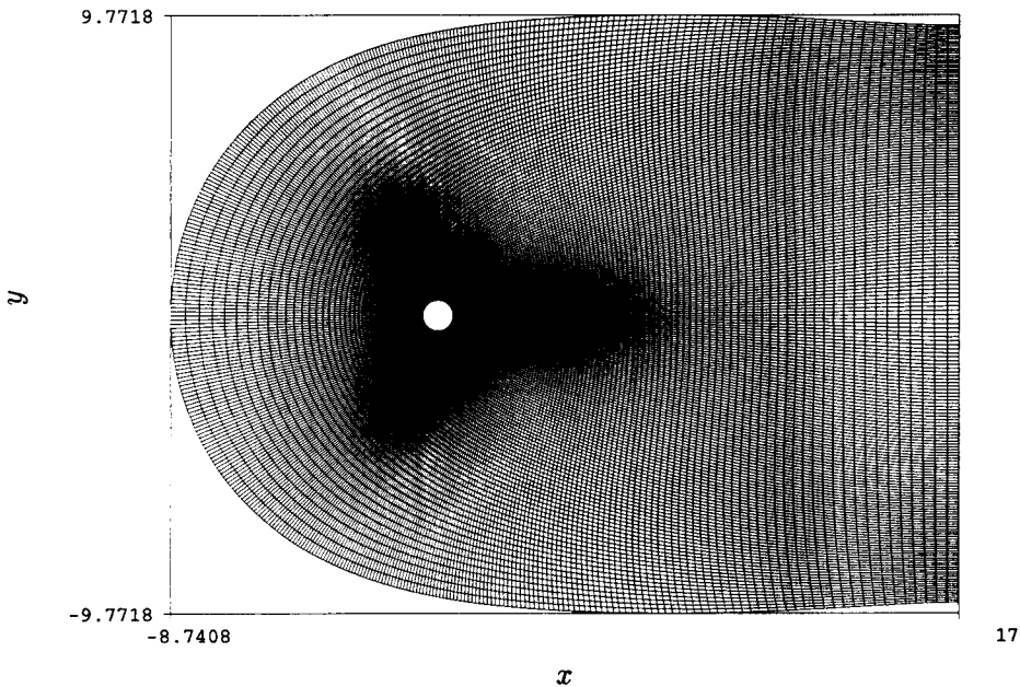
FIGURE 1. C -mesh used for Run-II.
