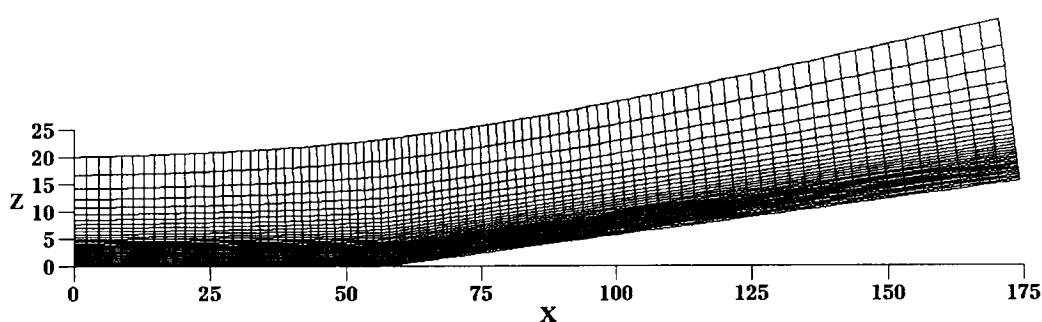
FIGURE 2. Grid for 7.5^\circ ramp, each 4th grid line shown.
