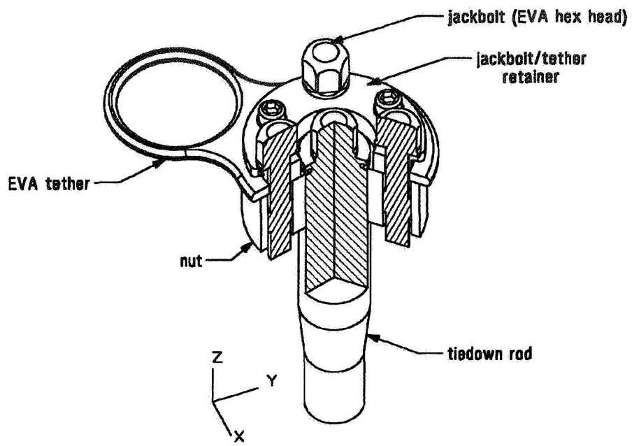
Figure 2. Superbolt Detail
