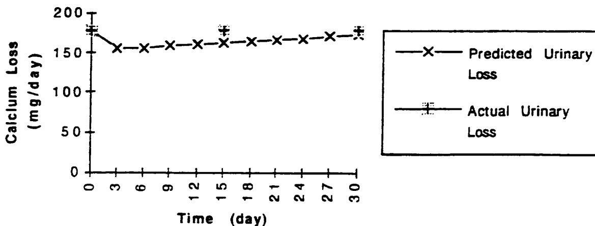
Figure 9: Urinary calcium excretion during head-down tilt where the sodium intake was restricted to 110 meq/day. (actual data taken from [9])
