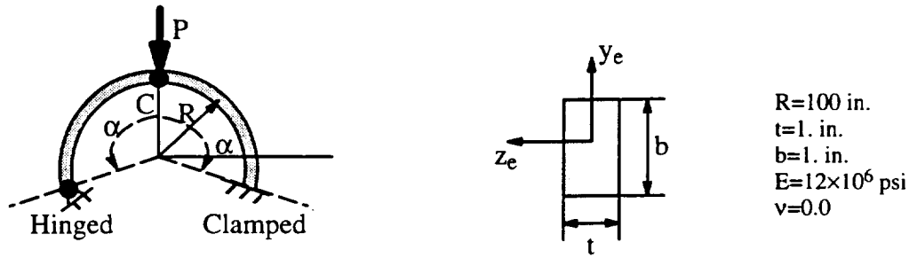
Figure 9. Clamped-hinged circular arch.
