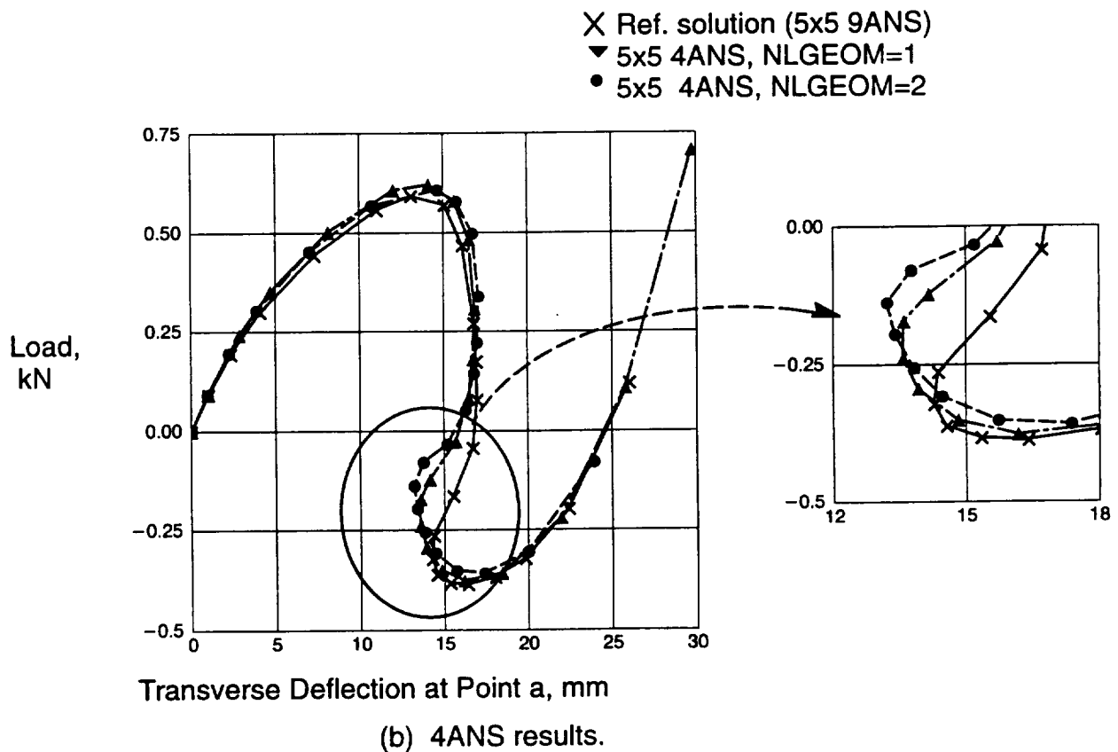
Figure 16. Hinged Cylinder: Load vs. Center Point Deflection
