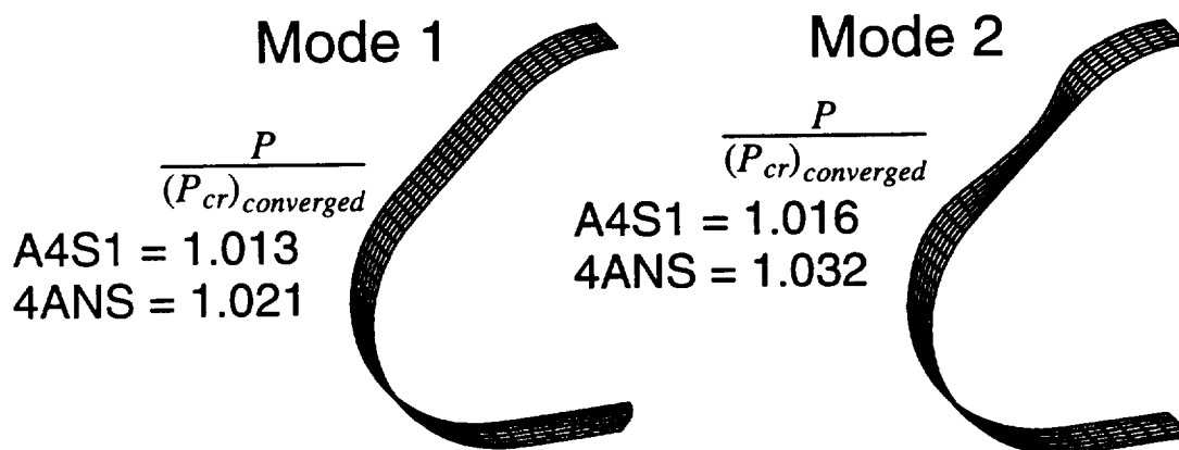
Figure 5. Comparison of linear buckling analysis results.
