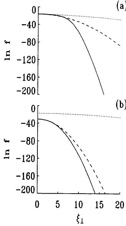
Figure 5: Distribution of perpendicular velocities of electrons at s = 4.375 \times 10^9 \text{cm} (solid lines) with (a) \xi_{\parallel} = \xi \cdot \hat{s} = 6 and (b) \xi_{\parallel} = 10 . The dotted curves are the equivalent result for the infinite homogeneous case.
