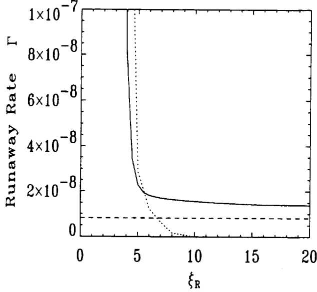
Figure 7: Variation of the rate \Gamma as a function of \xi_R for the case of the infinitely long homogeneous plasma(dotted line), and for position s = 4.375 \times 10^9 cm along the finite sized acceleration region(solid line). The horizontal broken line indicates the runaway rate computed from the expression of Kruskal and Bernstein given in section 2.
