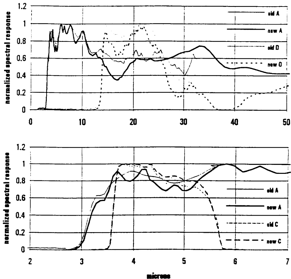
Figure 7. Revised NFR spectral response curves (heavy lines) compared to previous spectral response curves (light lines).
