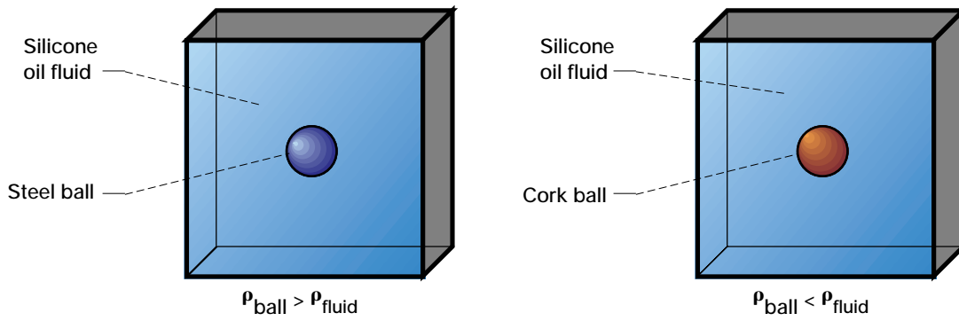
Figure 5.—Forward and reverse polarity fluidic sensor.
