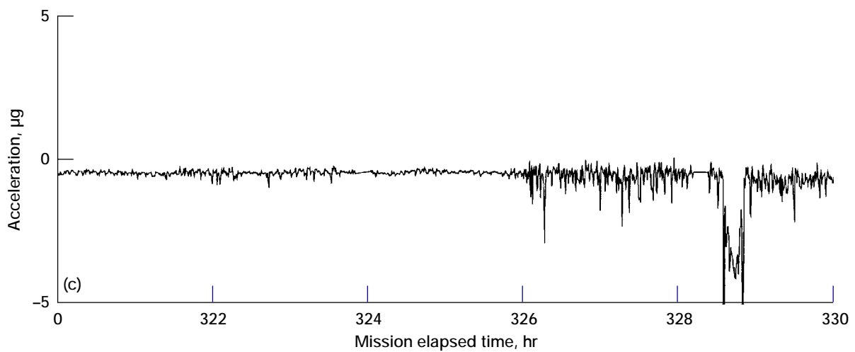
Figure 24.—Acceleration magnitude variation at orbital period with elliptical orbit. (a) X-axis. (b) Y-axis. (c) Z-axis.
