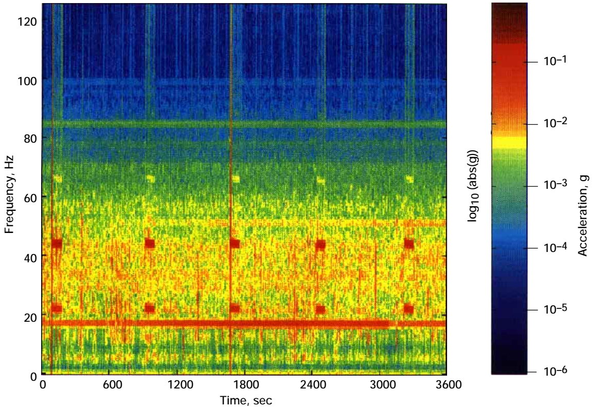
Figure 14.—Acceleration magnitude versus time versus frequency. STS-47, TSH-A, MET 000/23:00:00, 1 hr, f_c = 50 Hz; 250 s/s.
