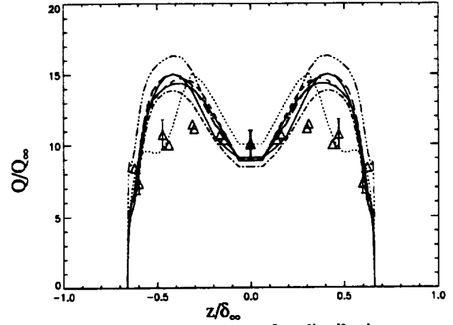
Fig. 7d. Surface heat transfer distribution on crossflow plane located at x/\delta_\infty = 7.78 and y/\delta_\infty = 0 .
