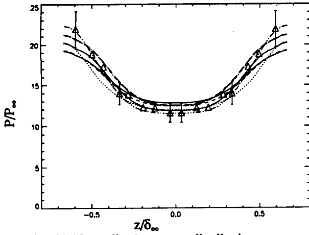
Fig. 6d. Normalized pressure distribution on cross-flow plane located at x/\delta_\infty = 8.3 and y/\delta_\infty = 0 .
