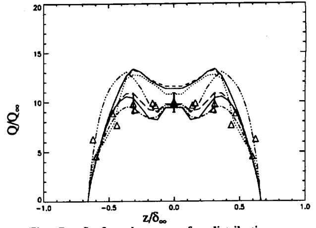
Fig. 7c. Surface heat transfer distribution on crossflow plane located at x/\delta_\infty = 6.4 and y/\delta_\infty = 0 .
