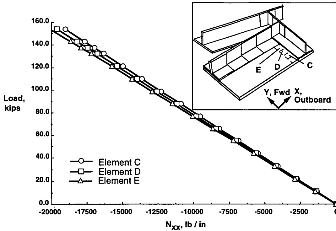
Figure 37. Axial stress resultants for skin elements near stringer runout 2.
