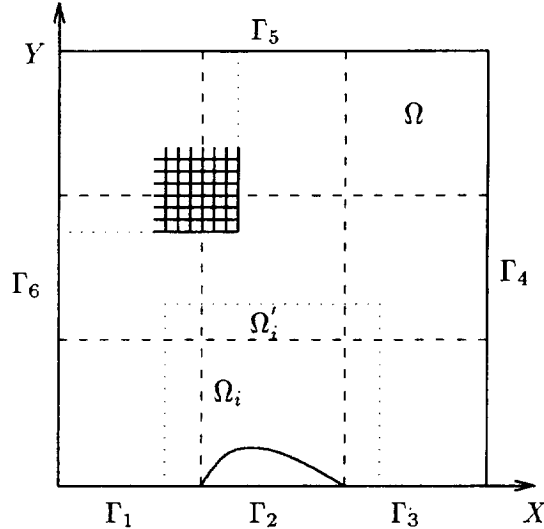
Figure 3: Domain \Omega with an exaggerated NACA 0012 curve at the bottom. The dashed lines indicate the partition of the domain into nonoverlapping substructures, and the dotted lines indicate the overlapping subdomains. The incomplete fine mesh of solid lines illustrates an overlap of 3 subintervals. \Gamma_6 is the inflow, \Gamma_5 the freestream, and \Gamma_4 the outflow boundary.
