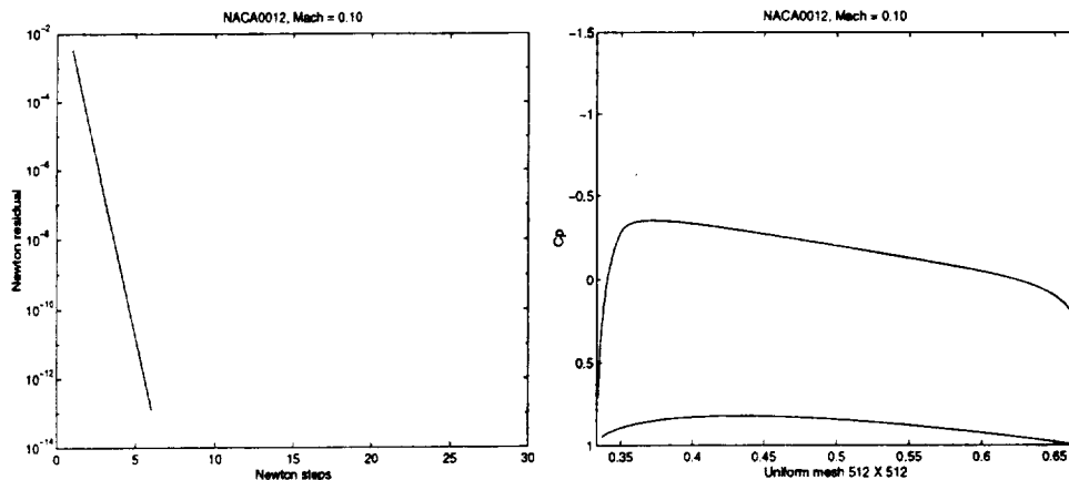
Figure 4: For M_\infty = 0.1 , the left figure shows the history of the Newton residual, and the right shows the (upper surface) C_p curve at convergence.
