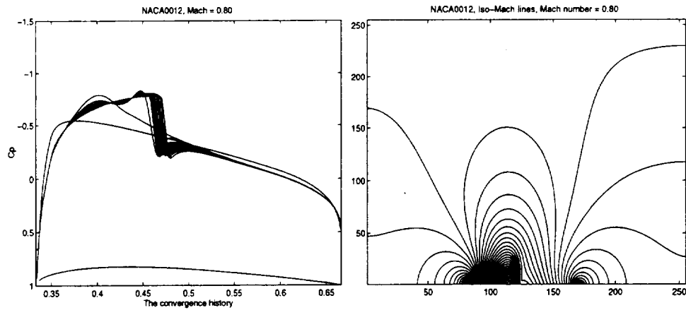
Figure 6: The left figure shows the convergence history of the C_p curves at M_\infty = 0.8 . The right figure shows the Mach contours of the final solution at M_\infty = 0.8 .
