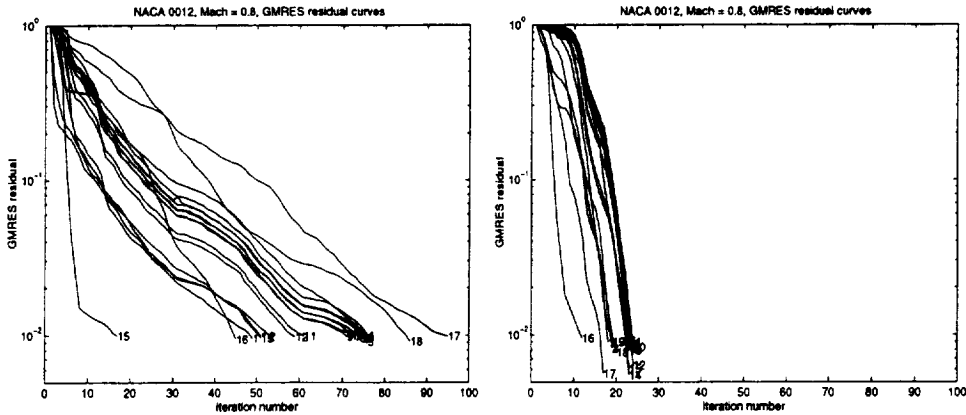
Figure 7: The GMRES convergence history for the entire nonlinear iteration. The left figure does not have a coarse space in the Schwarz preconditioner, the right figure contains a 7 \times 8 coarse space. The number at the tail of each curve corresponds to the Newton iteration number.
