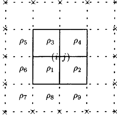
Figure 1: The finite element stencil. \Phi is stored at the cell vertices and \rho at the cell centers.
