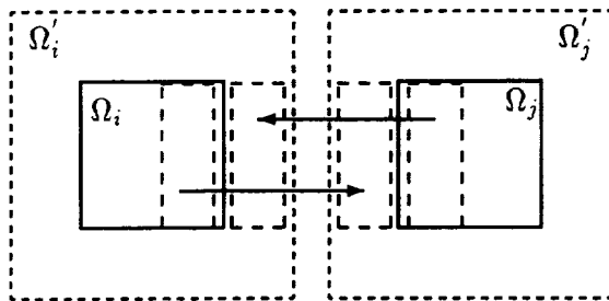
Figure 2: Illustration of two-way buffer copies required at each nearest-neighbor boundary. For each action of the Schwarz preconditioner on a vector the data needed in the extended regions are copied from the interior of neighboring subdomains. The amount of data moved for each processor is proportional to the area of overlap.
