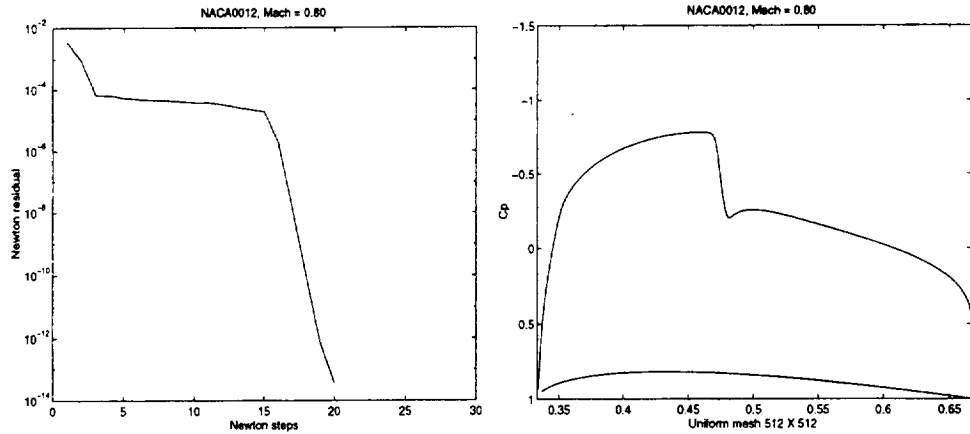
Figure 5: For M_\infty = 0.8 , the left figure shows the history of the Newton residual, and the right shows the (upper surface) C_p curve at convergence.
