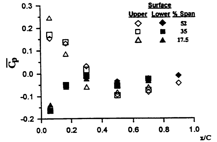
Fig. 10 Spanwise variation of airfoil surface pressure coefficient distribution, M=0.8, \alpha=10^\circ
