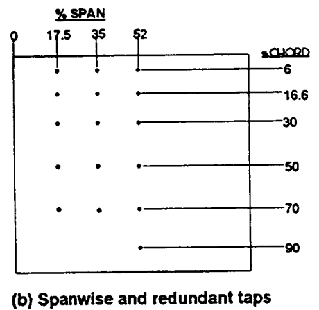
Fig. 5 Airfoil surface pressure taps
