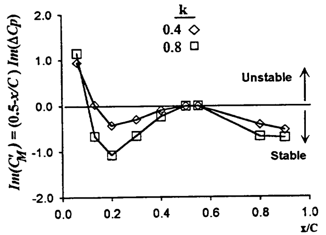
Fig. 17 Effect of reduced frequency on chordwise distribution of unsteady aerodynamic work/cycle, M=0.8
