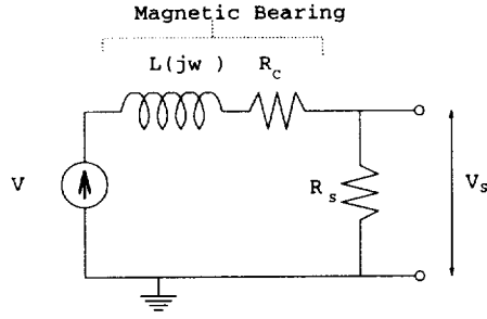
Figure 8: Test circuit.
