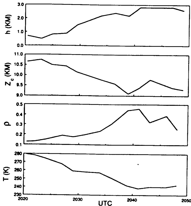
FIG. 17. Comparison of GOES and lidar observations along wind vector over FMC during 28 October 1986.
