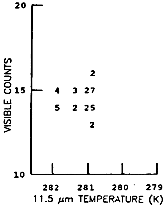
FIG. 4a. VIS-IR histogram of GOES pixels over FMC at 1500 UTC 27 October 1986 (numbers denote frequency of occurrence of temperature-count pairs).
