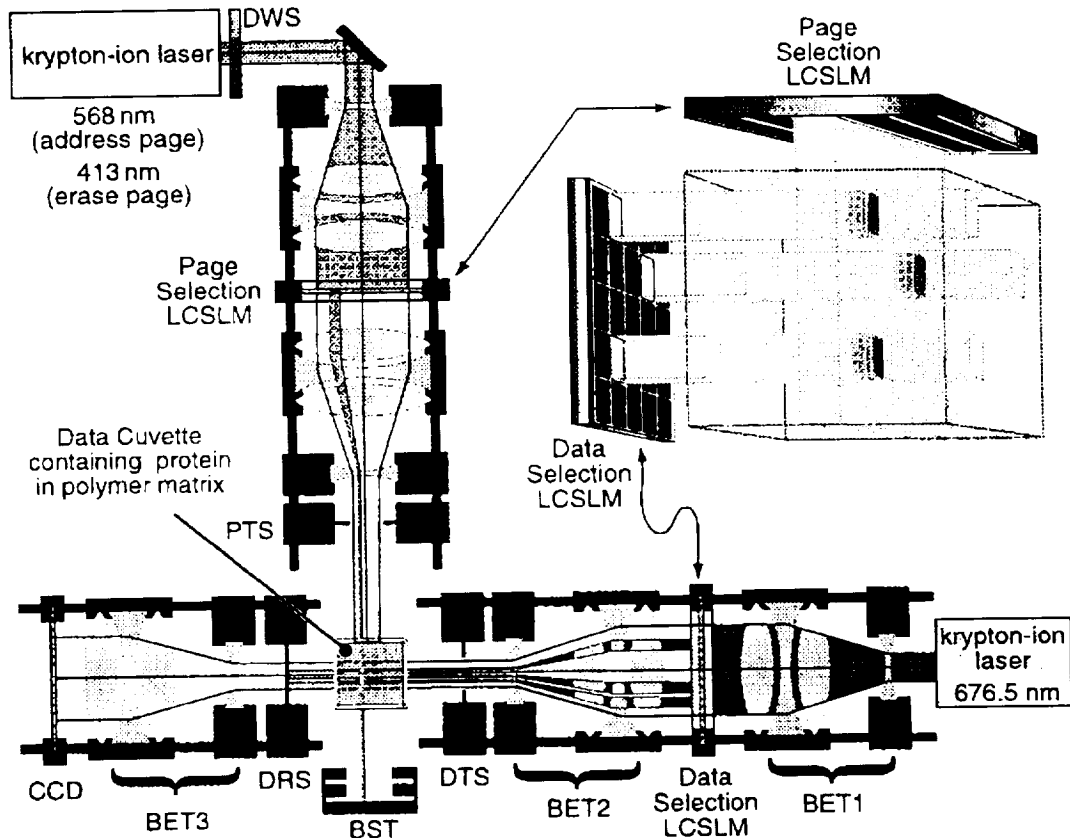
Figure 8. Schematic diagram of the branched-photocycle volumetric memory prototype base on bR.
