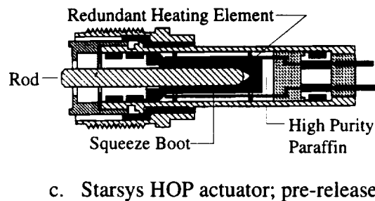
Figure 5. NEA pin-pullers.
