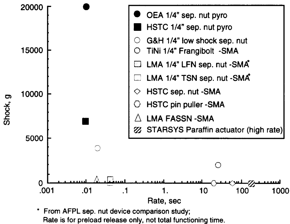
Figure 2. Functional shock versus operational rates for some pyrotechnics and NEAs.
