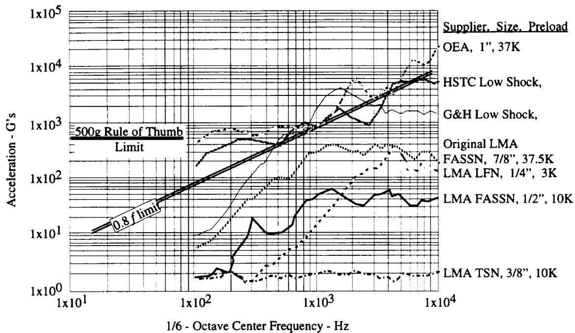
Figure 8. LMA plate tests - functional shock comparison.
