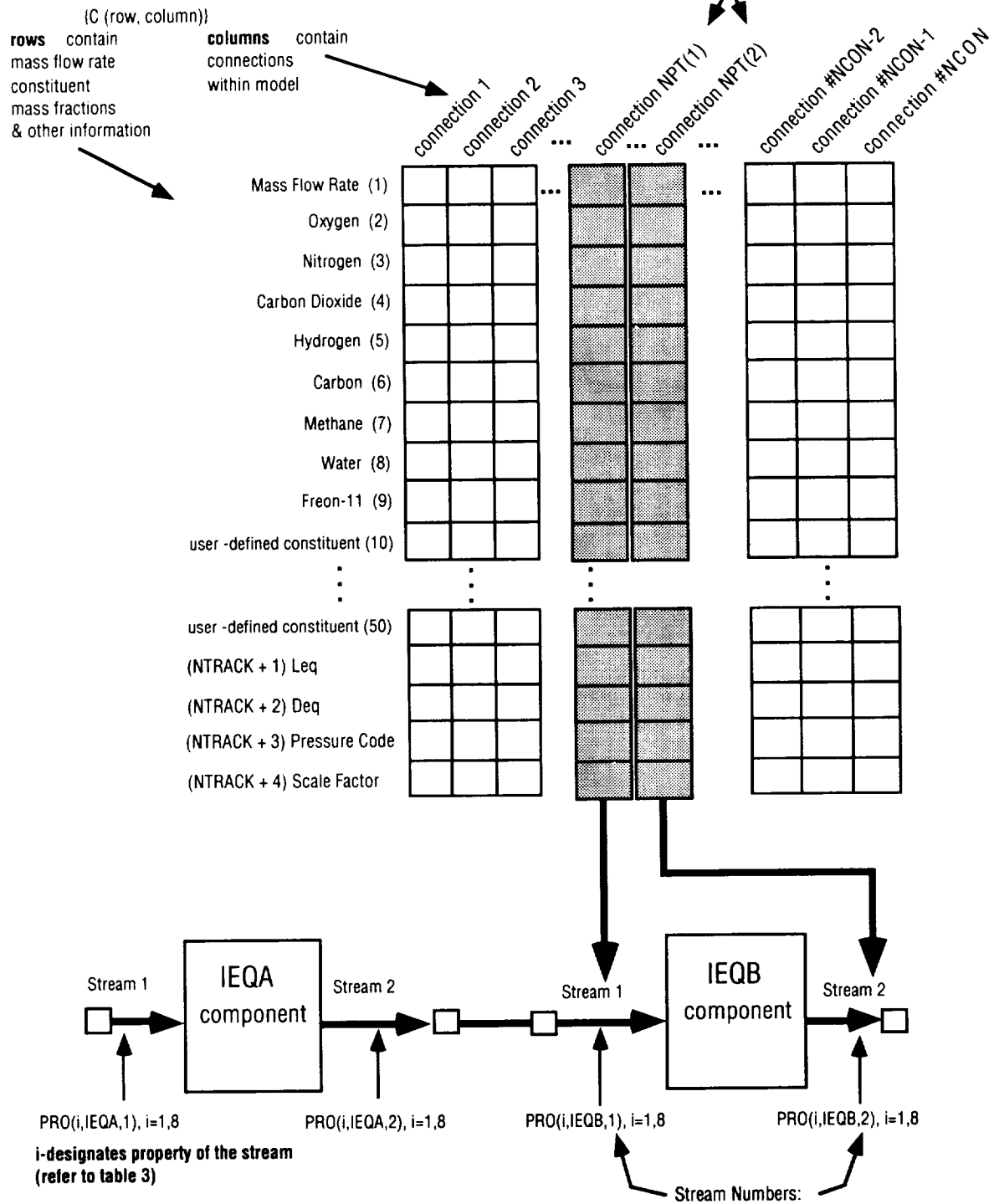
Figure 18. Stream properties and composition arrays.
