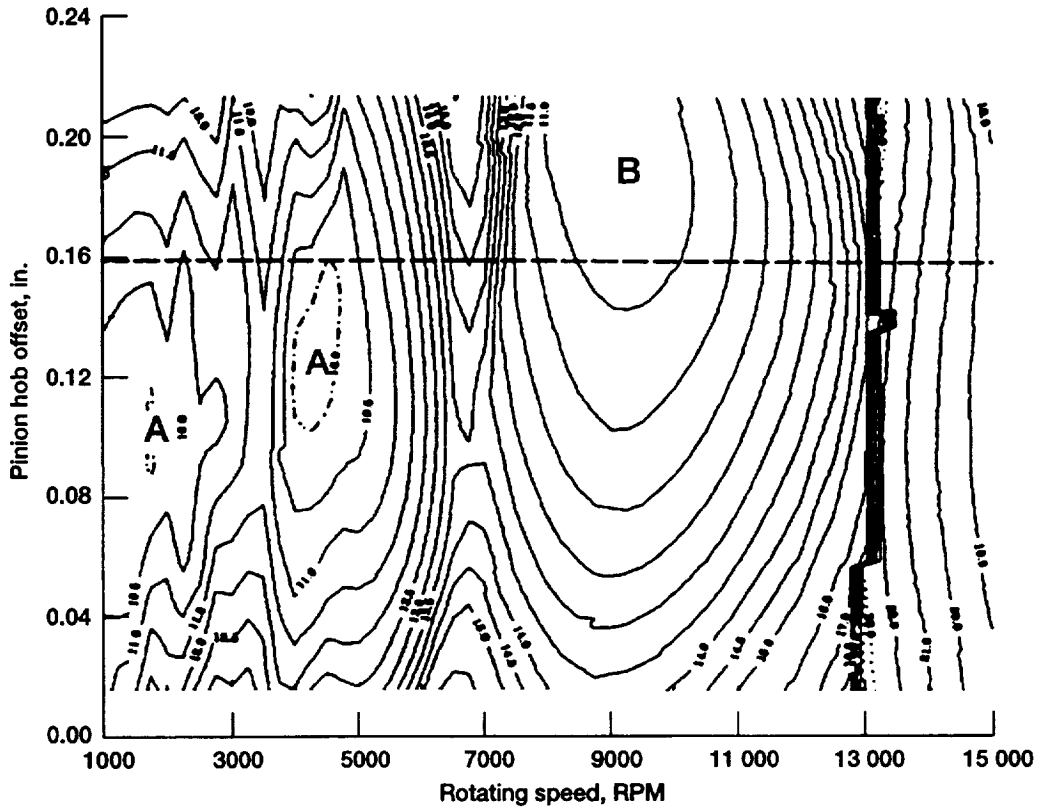
Figure 3.—Contour diagram showing the effect of pinion hob offset and rotating speed on pinion dynamic stress. (The optimal static case hob offset is shown by the dashed line.)
