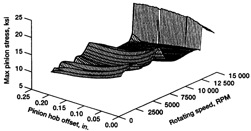
Figure 4.—Effect of pinion hob offset ( e_1 ) and rotating speed on gear dynamic stress. (The hob offset for the gear is determined from eq. 1.)
