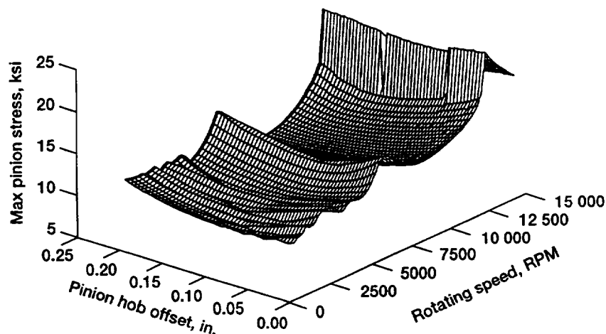
Figure 2.—Effect of pinion hob offset ( e_1 ) and rotating speed on pinion dynamic stress.
