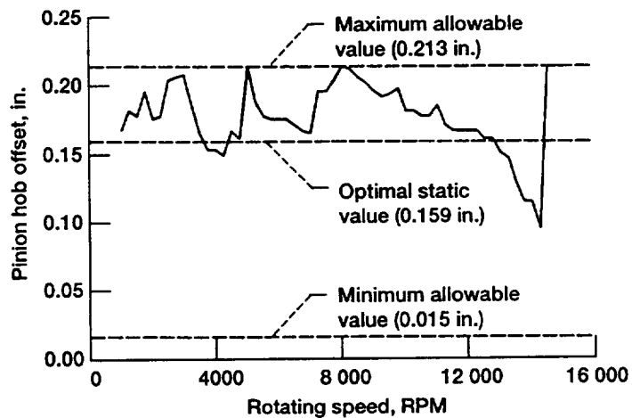
Figure 6.—Determining pinion hob offset to balance dynamic tooth strength of pinion and gear at different speeds.
