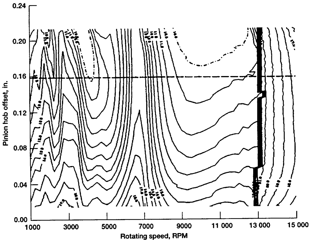
Figure 5.—Contour diagram showing the effect of pinion hob offset and rotating speed on gear dynamic stress. (The hob offset for the gear is determined from eq. 1. The optimal static case hob offset is shown by the dashed line.)
