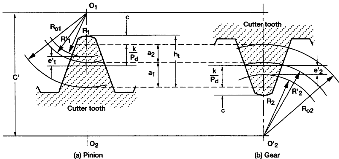
Figure 1.—Gear pair cut by offset hobs to mesh at an extended center distance.
