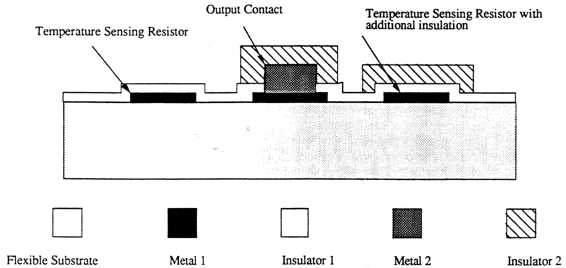
Figure 4: Cross section of a single heat flux sensor.
