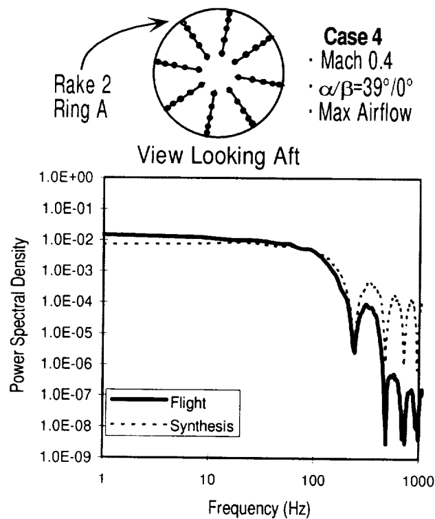
Figure 18. Power Spectral Density of Filtered Flight and Synthesized Time Histories
