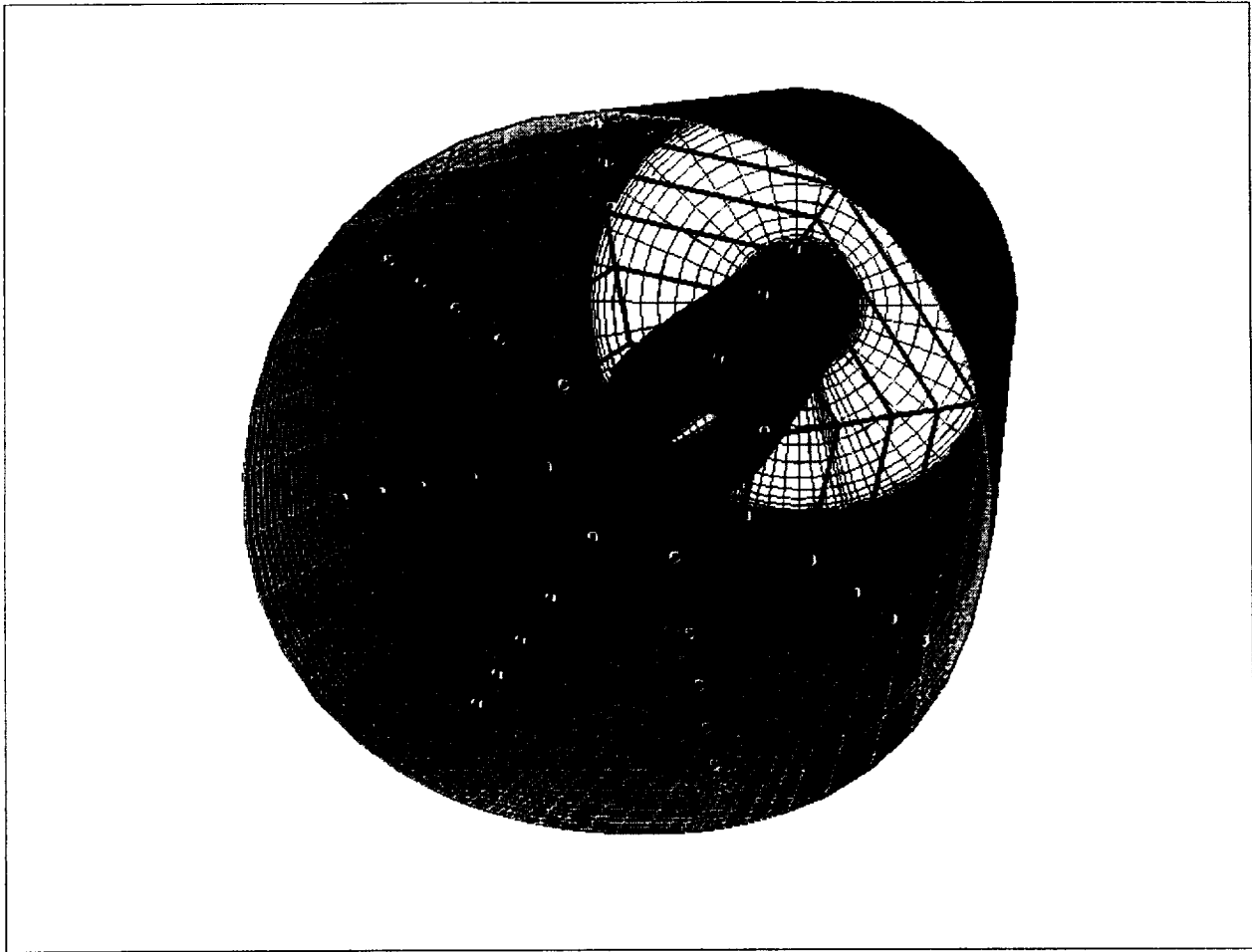
Figure 7. Aft Diffuser Modeling Showing AIP Probe Positions and Centerbody Shape
