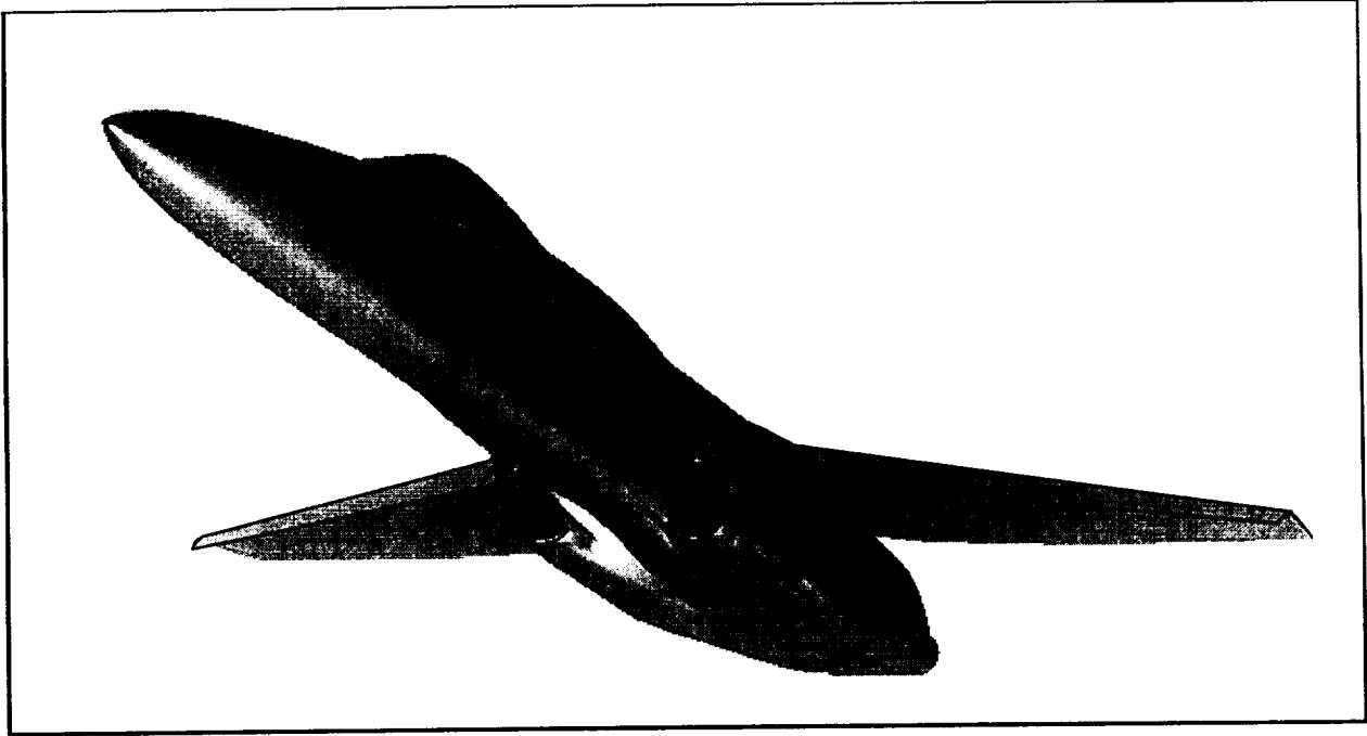
Figure 4. Surface Geometry for HARV CFD Solutions
