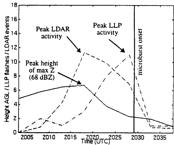
Figure 3. Time series of height of maximum reflectivity (Z) in km (solid curve), number of LDAR events (in 1000's, dashed curve), and number of LLP events (dash-dot curve). LDAR and LLP events are summed over the time of one volume scan and the volume encompassed by storm reflectivities greater than 30 dBZ.
