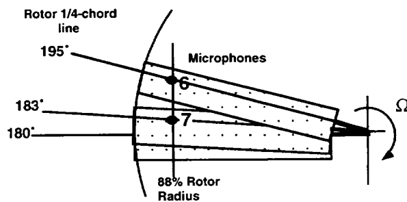
Figure 2.4 Schematic of rotor quarter-chord line passing over microphones.
