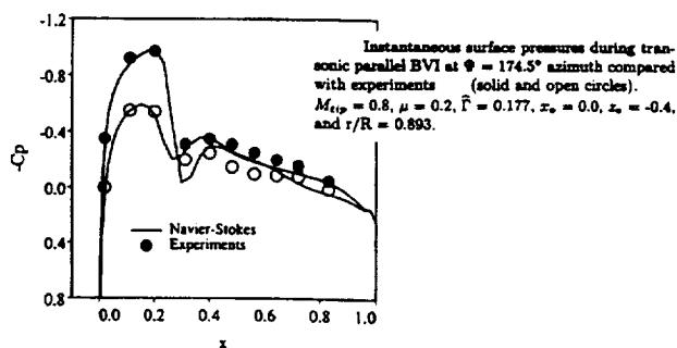
Figure 3.4 Comparison of experimental and computational blade-surface pressures for a rotor in forward flight (ref. 38).
