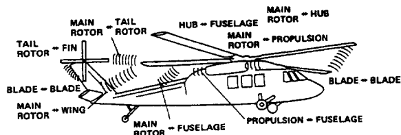
Figure 1.1 Examples of aerodynamic interactions of a helicopter that are possible noise sources.
