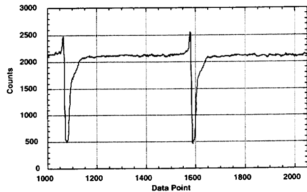
Figure 2.9 Example of a single revolution of pressure data, unaveraged in original units. Case I, M_{tip} = 0.6 , microphone 6.
