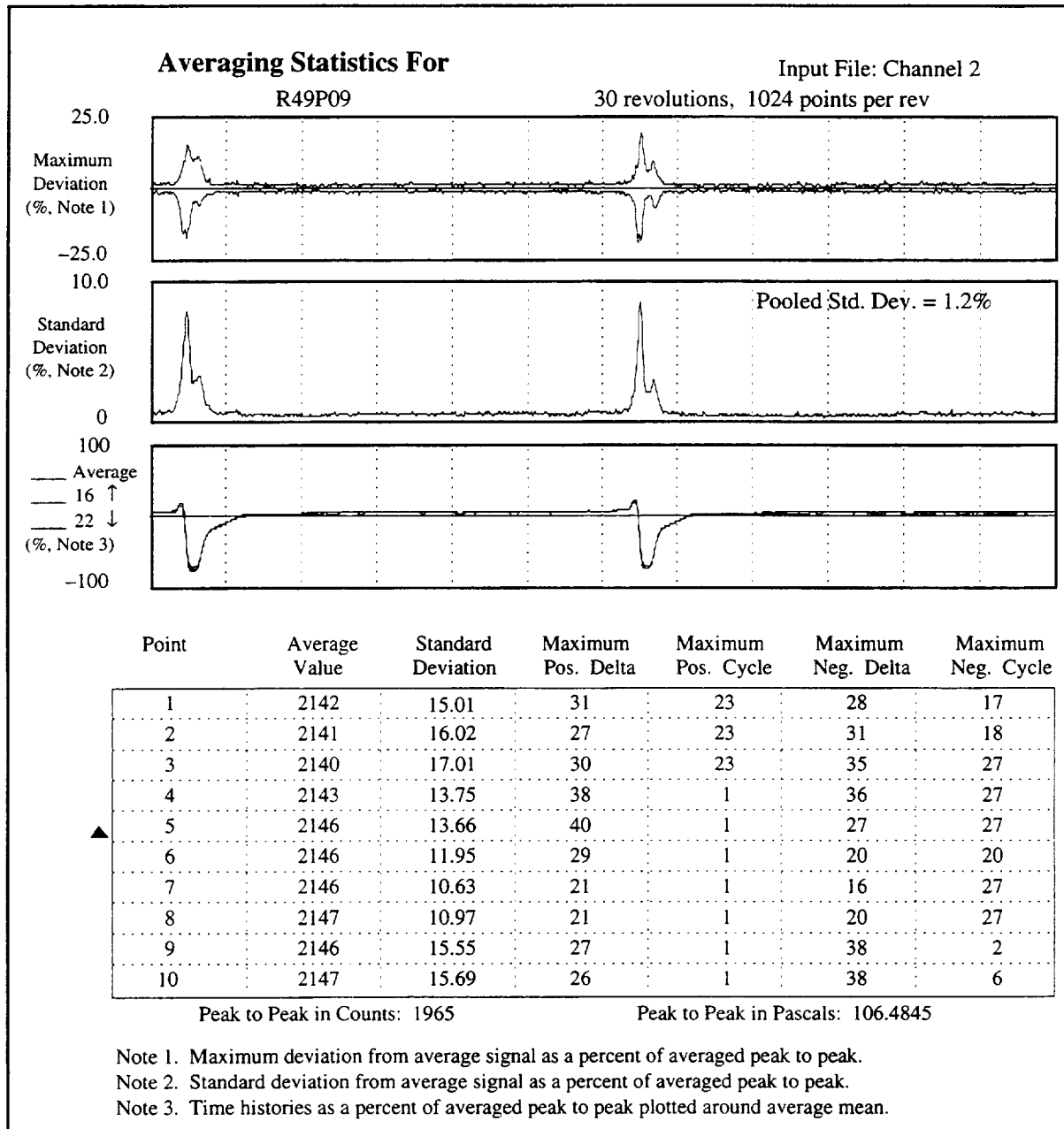
Figure 2.11 Averaging Statistics for Run 49, Point 09, Case I, M_{tip} = 0.6 , microphone 6.
