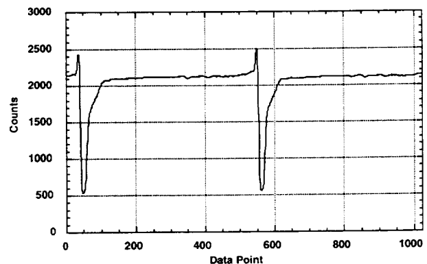
Figure 2.10 Example of one revolution of averaged pressure data. Case I, M_{tip} = 0.6 , microphone 6.
