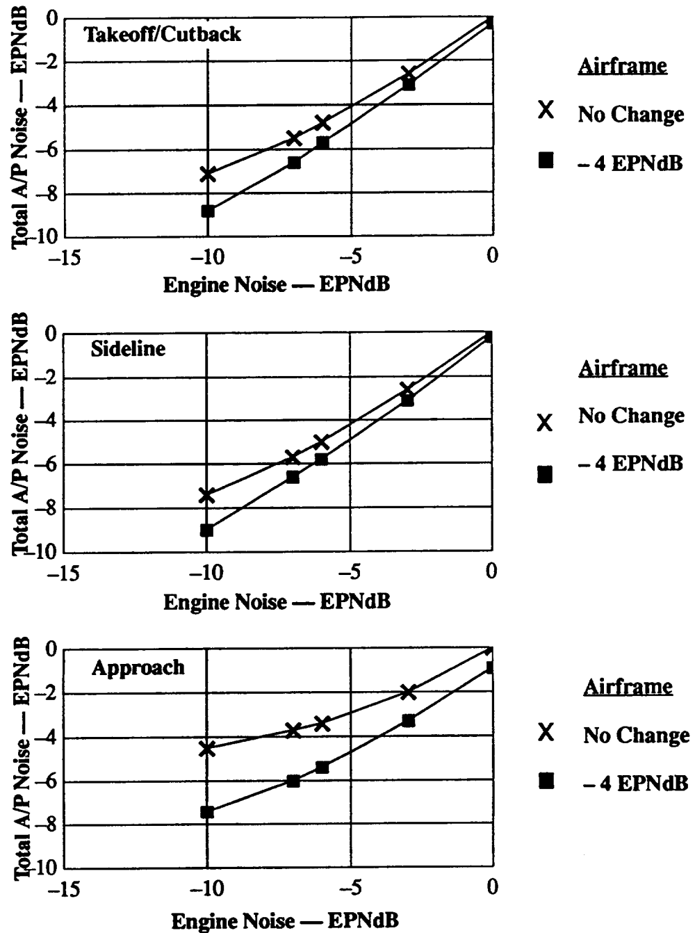
Figure 5d. Estimated Impact of Engine and Airframe Noise Reduction on Total Airplane Noise—Four-Engine Large Commercial Transport.
