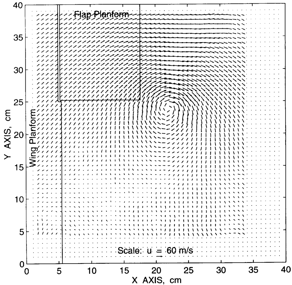
Figure 12. Baseline configuration with Flap Edge Device; Velocity field at 18 inches aft of flap trailing edge.
