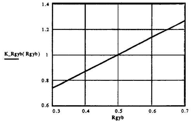
Fig. 17 Radius of gyration ratio correction factor K_{R_{gyb}} .
