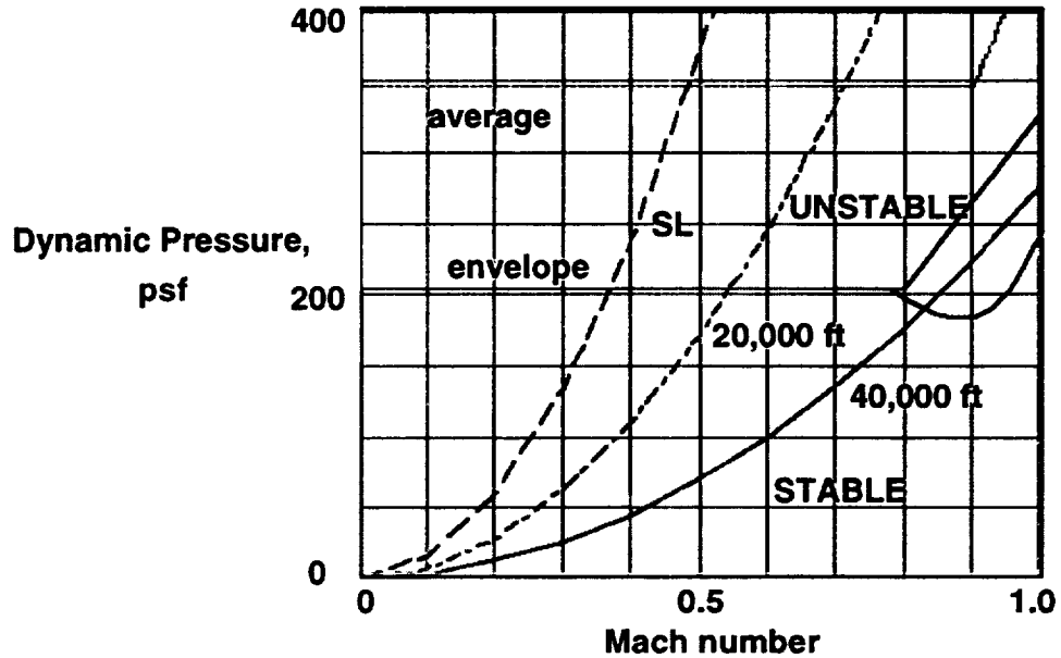
Fig. 8. Outer wing flutter dynamic pressure boundary vs. Mach number for wing-root torsional stiffness 40 \times 10^8 lb-ft 2 .
