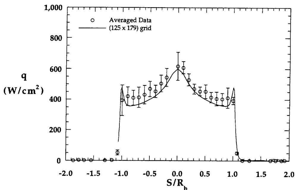
Figure 8.2.52a Comparison with Experimental Forebody Heating Distribution, MP-2 Configuration, HYPULSE, \text{CO}_2
