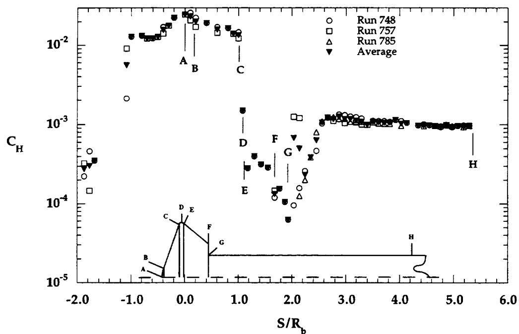
Figure 6.2.5b MP-1 Configuration, \alpha = -4 deg, \text{CO}_2 in HYPULSE (log scale)
