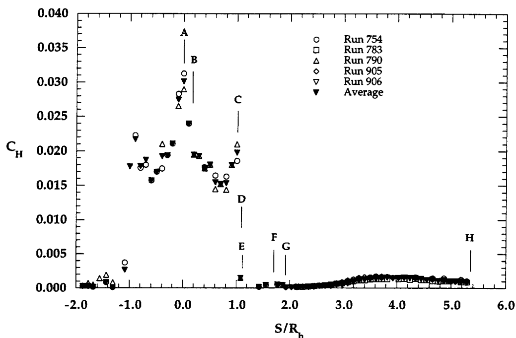
Figure 6.2.6a MP-1 Configuration, \alpha = 0^\circ , Air in HYPULSE (linear scale)
