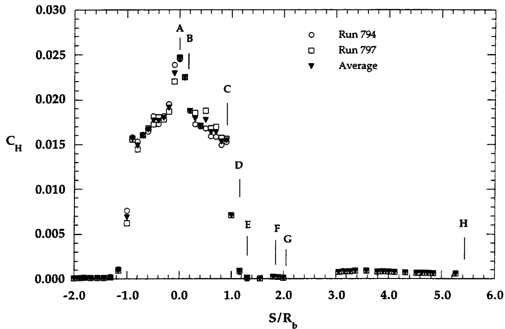
Figure 6.2.12a MP-4 Configuration, \alpha = 0^\circ , \text{CO}_2 in HYPULSE (linear scale)
