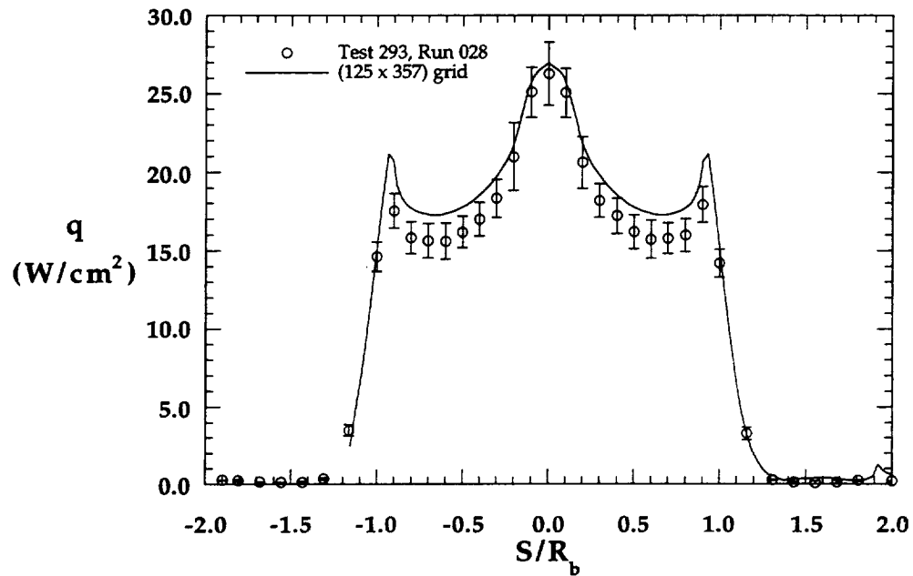
Figure 8.1.74a Comparison with Experimental Forebody Heating Distribution, MP-4 Configuration, 31-Inch Mach 10, Re_{\infty} = 2.0 \times 10^6 \text{ ft}^{-1}
