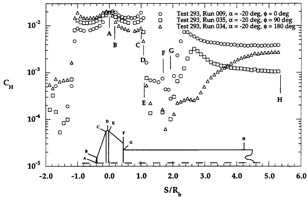
Figure 6.1.12b MP-1 C_H Distributions, \alpha = -20^\circ , Re_\infty = 1.0 \times 10^6 \text{ ft}^{-1} (log scale)
