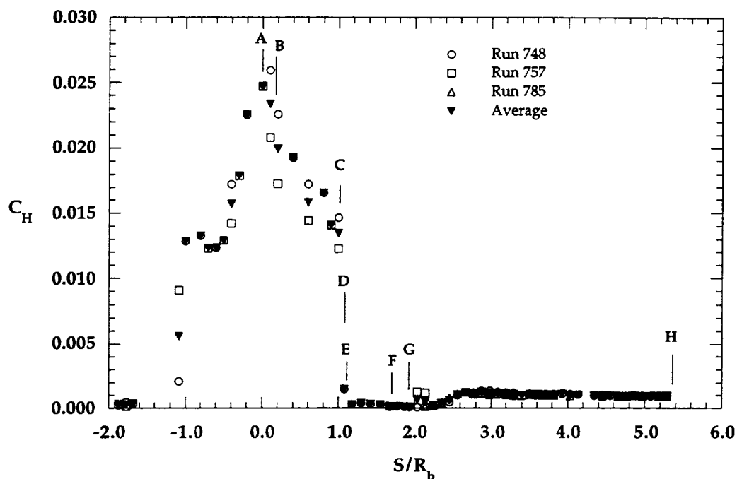
Figure 6.2.5a MP-1 Configuration, \alpha = -4 deg, \text{CO}_2 in HYPULSE (linear scale)
