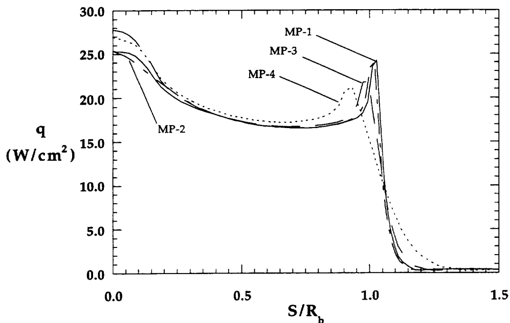
Figure 8.1.62a Configuration Effects on Forebody Heating, 31-Inch Mach 10, \text{Re}_\infty = 2.0 \times 10^6 \text{ ft}^{-1}
