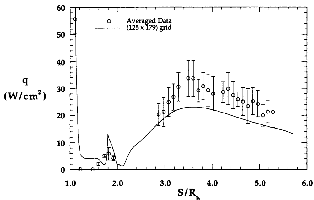
Figure 8.2.53b Comparison with Experimental Wake Heating Distribution, MP-3 Configuration, HYPULSE, \text{CO}_2
