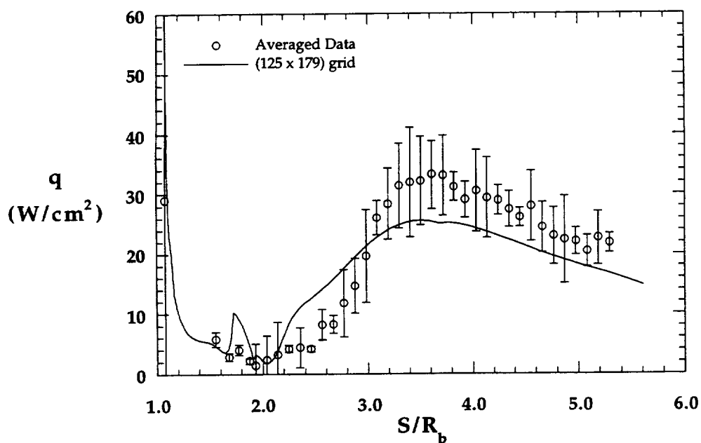
Figure 8.2.50b Comparison with Experimental Wake Heating Distribution, MP-1 Configuration, HYPULSE, \text{CO}_2
