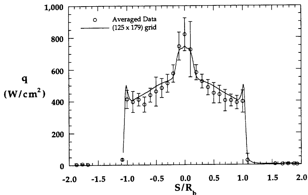
Figure 8.2.50a Comparison with Experimental Forebody Heating Distribution, MP-1 Configuration, HYPULSE, \text{CO}_2
