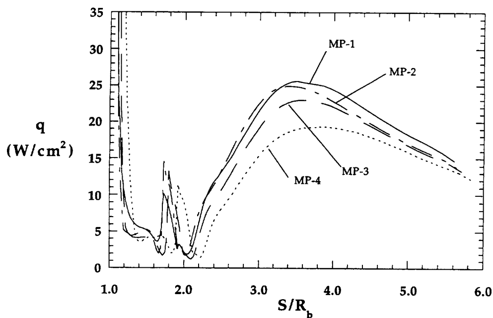
Figure 8.2.44b Configuration Effects on Wake Heating Distributions, HYPULSE, CO 2
