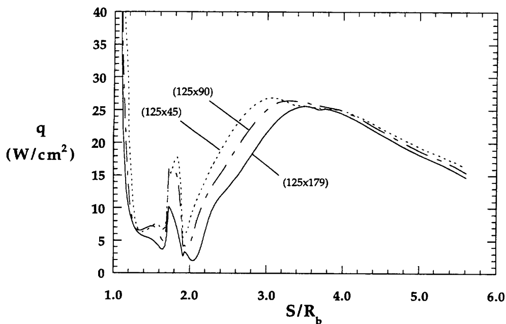
Figure 8.2.6b Grid Resolution Effects on Wake Heating, MP-1 Configuration, HYPULSE, \text{CO}_2
