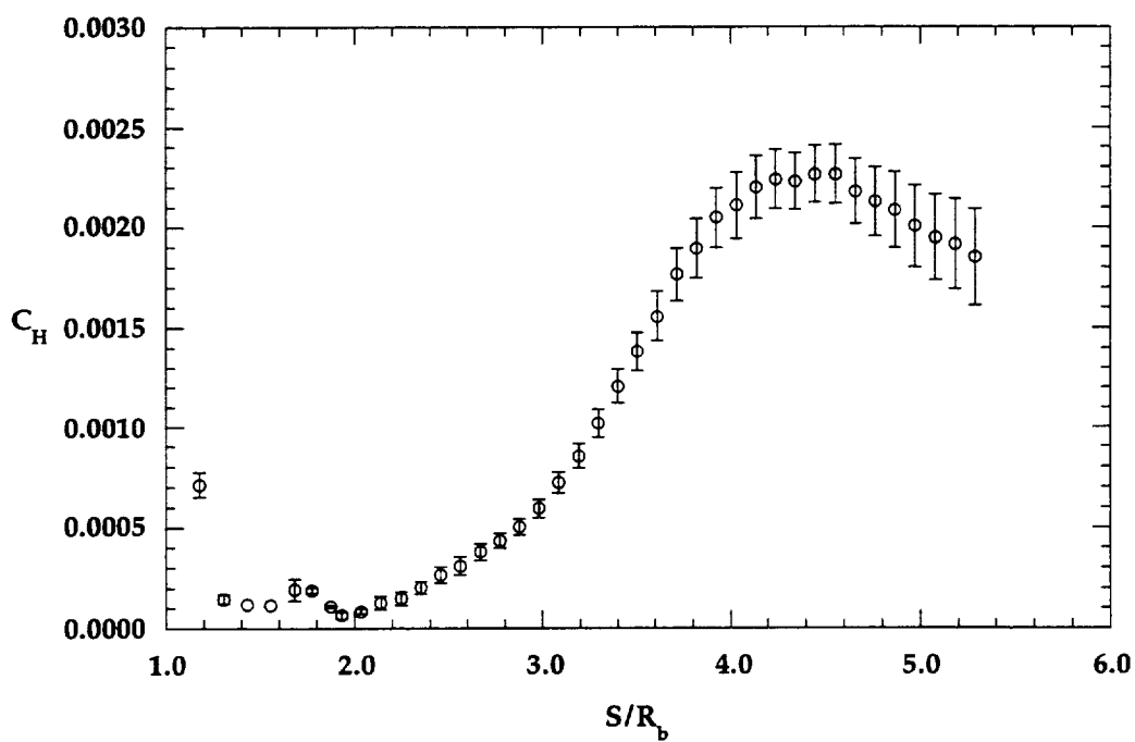
Figure 6.3.1b MP-1 Wake Uncertainty Estimates, Re=1.0 \times 10^6 \text{ ft}^{-1} in Mach 10
