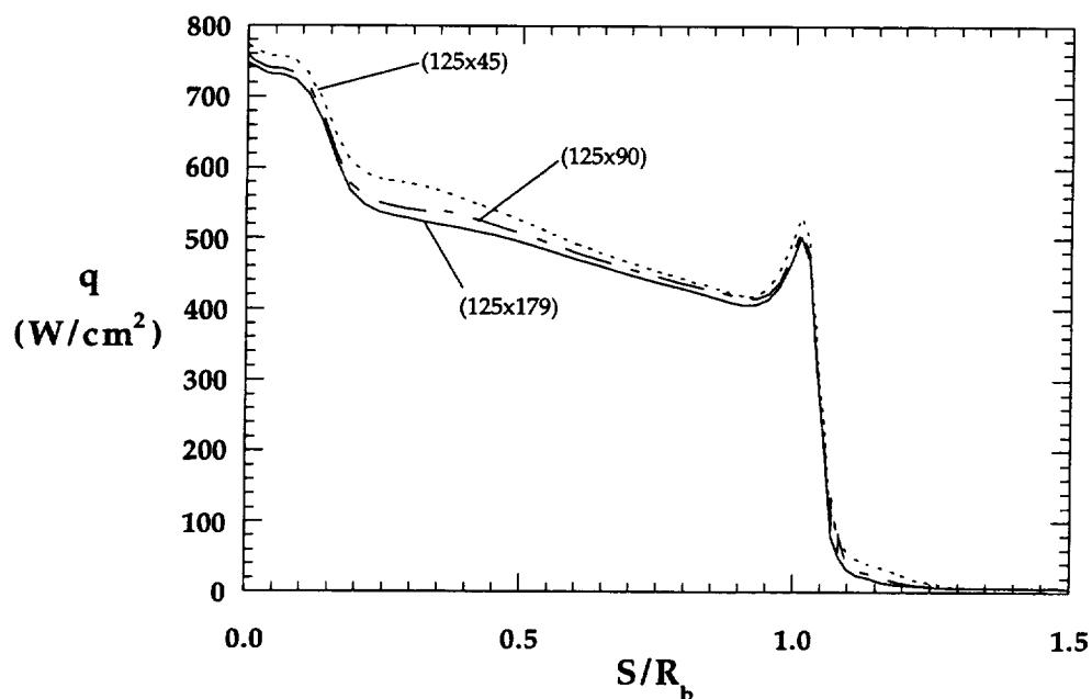
Figure 8.2.6a Grid Resolution Effects on Forebody Heating, MP-1 Configuration, HYPULSE, \text{CO}_2
