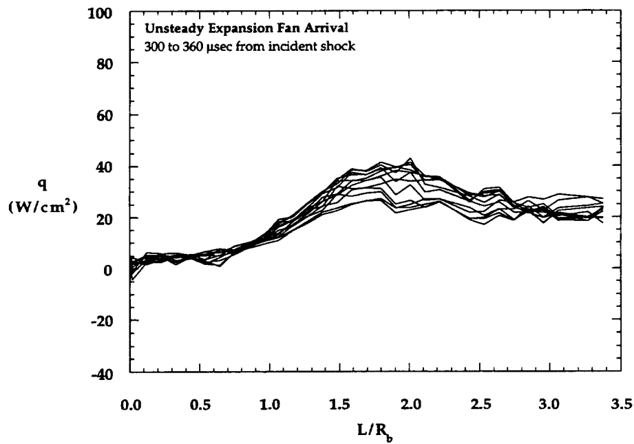
Figure 6.2.1f Wake Flow Establishment Movie, Run 749: 300 to 360 \mu\text{sec}
