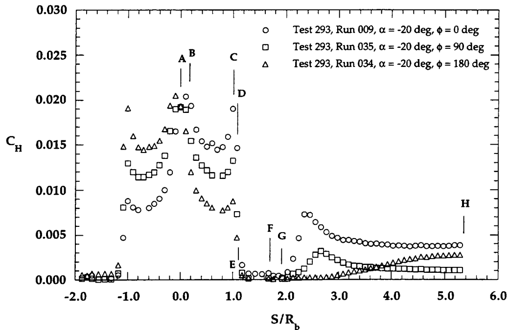
Figure 6.1.12a MP-1 C_H Distributions, \alpha = -20^\circ , Re_\infty = 1.0 \times 10^6 \text{ ft}^{-1} (linear scale)
