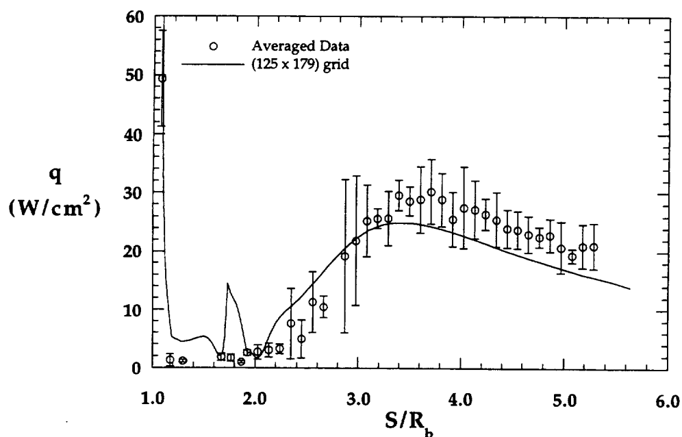
Figure 8.2.52b Comparison with Experimental Wake Heating Distribution, MP-2 Configuration, HYPULSE, \text{CO}_2
