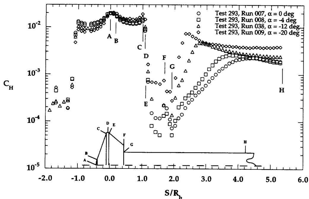
Figure 6.1.9b \alpha Effects on MP-1 Configuration, Re_\infty = 1.0 \times 10^6 \text{ ft}^{-1} (log scale)
