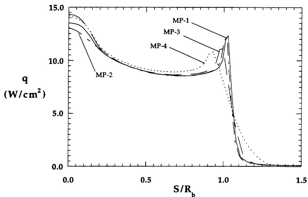
Figure 8.1.60a Configuration Effects on Forebody Heating, 31-Inch Mach 10, \text{Re}_\infty = 0.5 \times 10^6 \text{ ft}^{-1}
