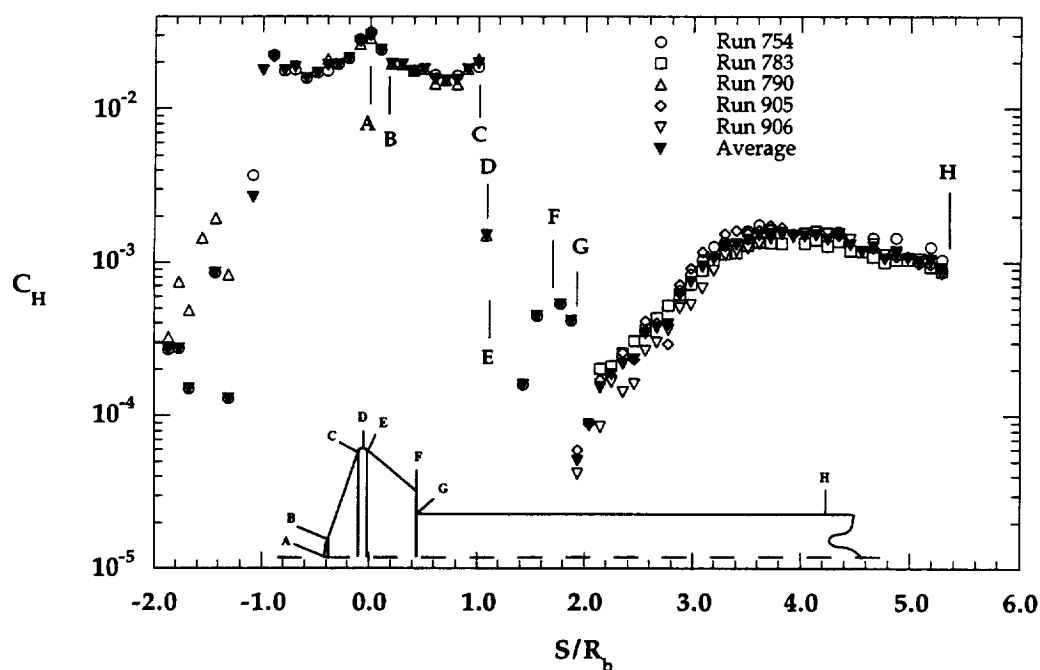
Figure 6.2.6b MP-1 Configuration, \alpha = 0^\circ , Air in HYPULSE (log scale)
