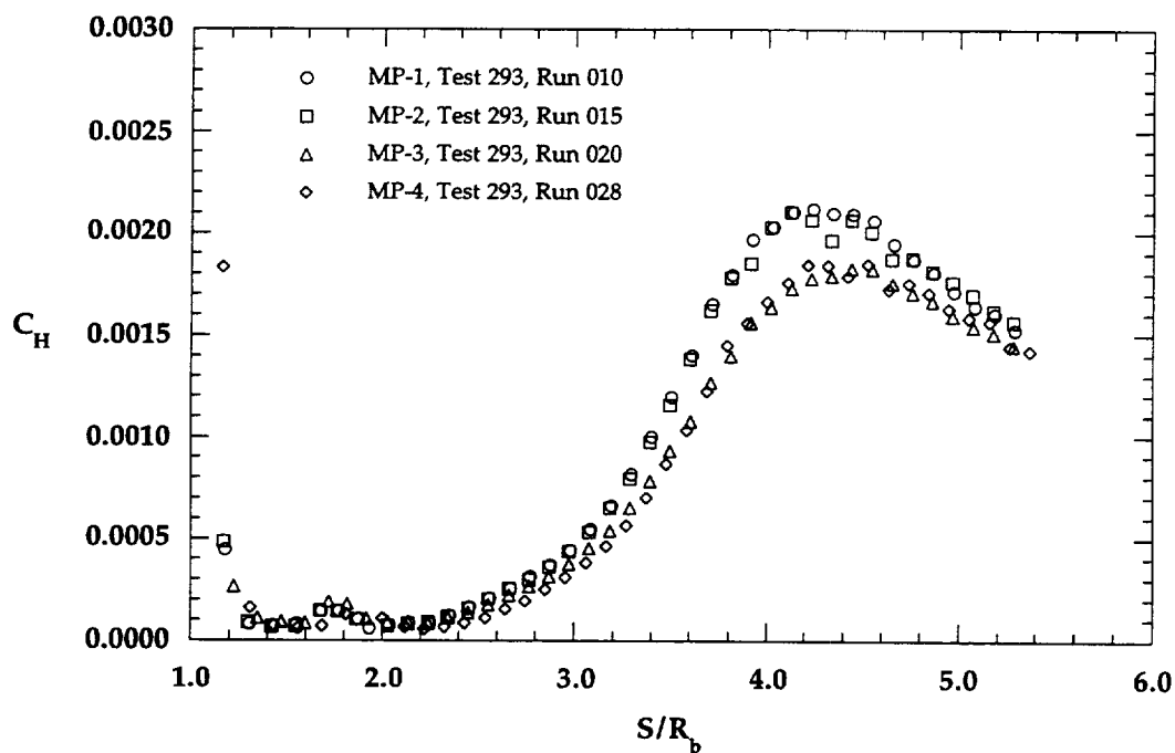
Figure 6.1.19b Configuration Effects on Wake, \alpha = 0^\circ , Re_\infty = 2.0 \times 10^6 \text{ ft}^{-1}
