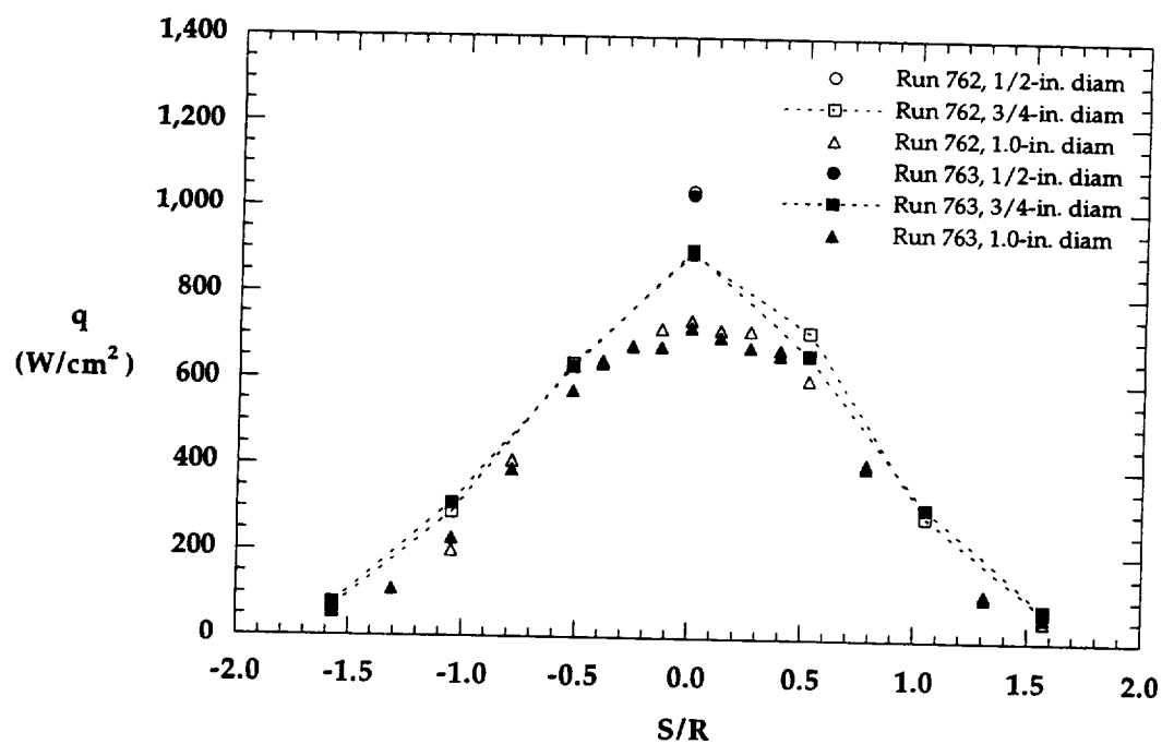
Figure C.2.3 HYPULSE Hemisphere Heating Data, \text{CO}_2 Tests
