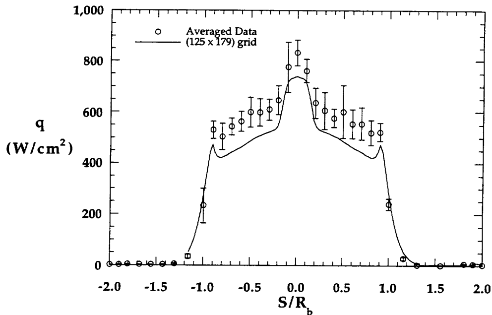
Figure 8.2.54a Comparison with Experimental Forebody Heating Distribution, MP-4 Configuration, HYPULSE, \text{CO}_2
