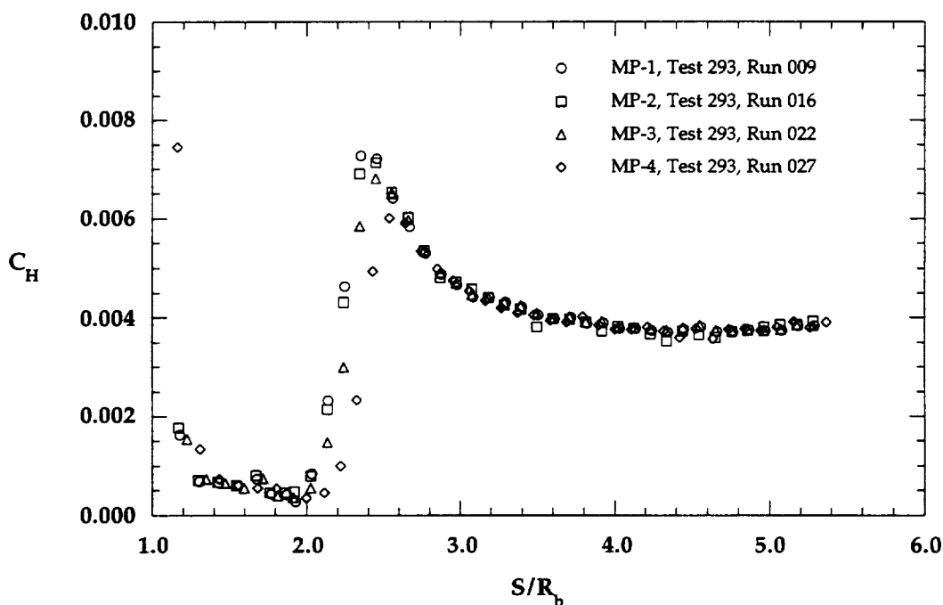
Figure 6.1.21b Configuration Effects on Wake, \alpha = -20 deg, Re_\infty = 1.0 \times 10^6 \text{ ft}^{-1}
