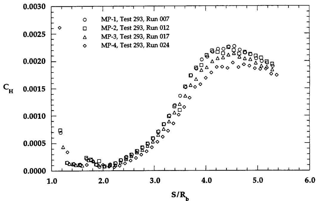
Figure 6.1.18b Configuration Effects on Wake, \alpha = 0^\circ , Re_\infty = 1.0 \times 10^6 \text{ ft}^{-1}
