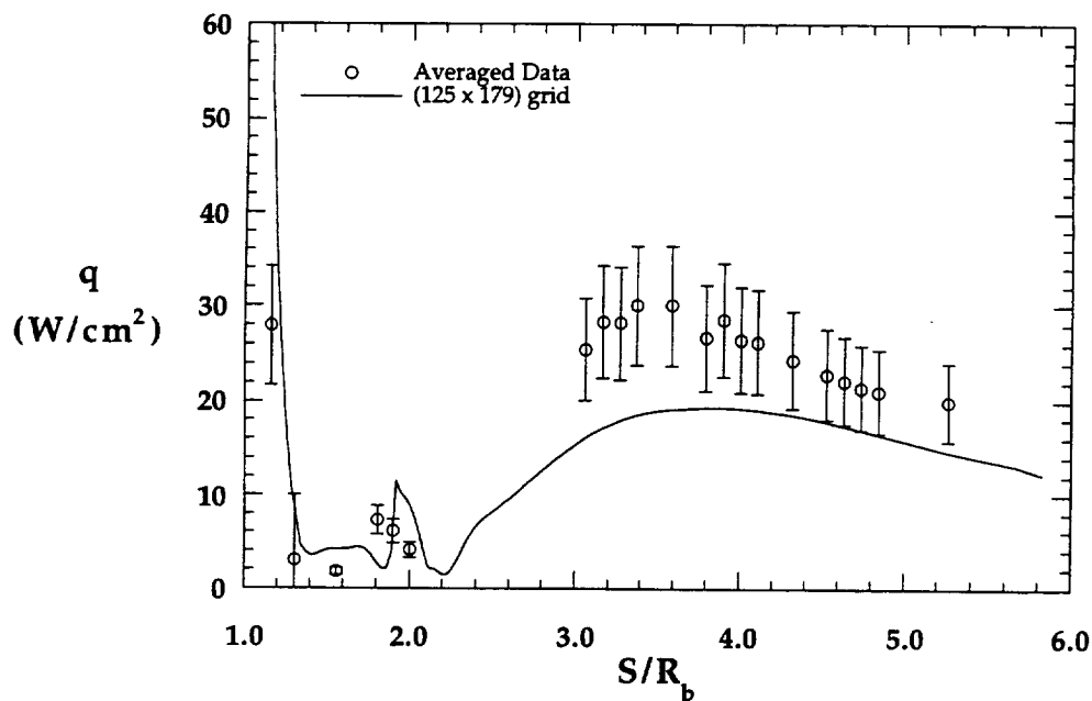
Figure 8.2.54b Comparison with Experimental Wake Heating Distribution, MP-4 Configuration, HYPULSE, \text{CO}_2
