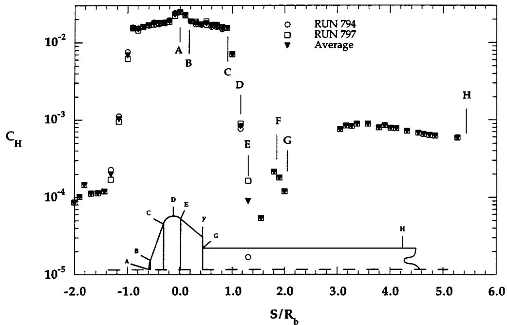
Figure 6.2.12b MP-4 Configuration, \alpha = 0^\circ , \text{CO}_2 in HYPULSE (log scale)
