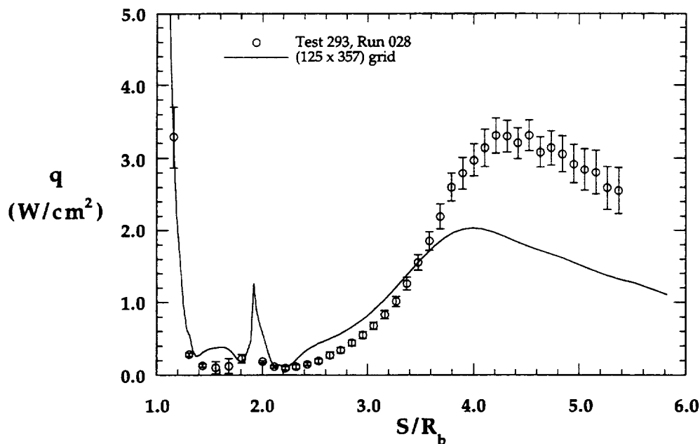
Figure 8.1.74b Comparison with Experimental Wake Heating Distribution, MP-4 Configuration, 31-Inch Mach 10, Re_{\infty} = 2.0 \times 10^6 \text{ ft}^{-1}
