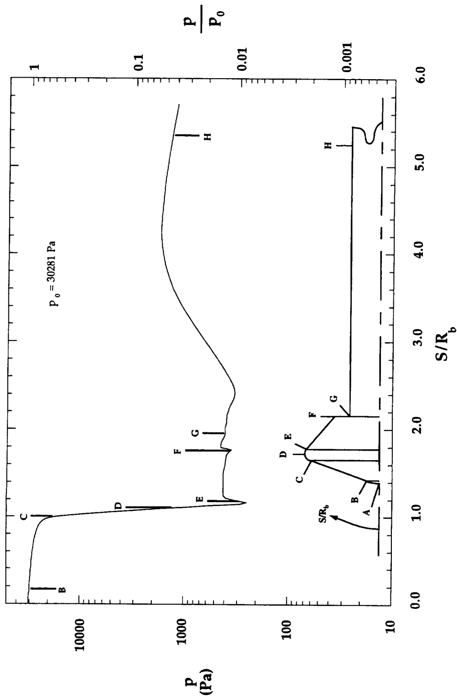
Figure 8.1.47 Computed Surface Pressure Distribution, MP-3 Configuration, 31-Inch Mach 10, Re_\infty = 2.0 \times 10^6
