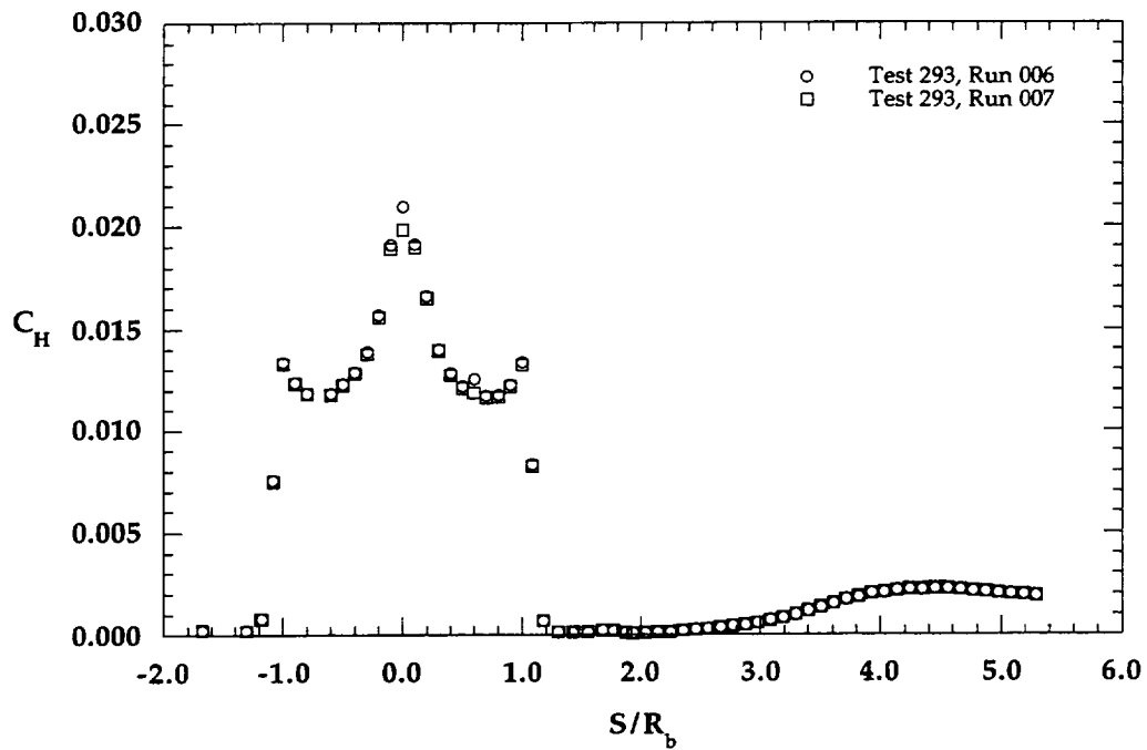
Figure 6.1.23a Repeatability, MP-1 Configuration, Re_\infty = 1.0 \times 10^6 \text{ ft}^{-1} (linear scale)
