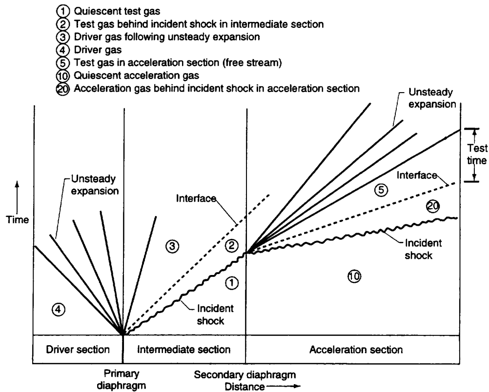
Figure 4.3.2 X-T Diagram for NASA HYPULSE Expansion Tube
