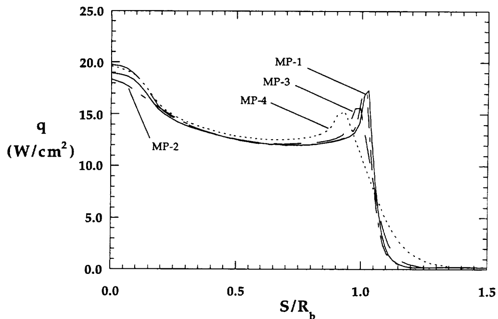
Figure 8.1.61a Configuration Effects on Forebody Heating, 31-Inch Mach 10, Re_\infty = 1.0 \times 10^6 \text{ ft}^{-1}
