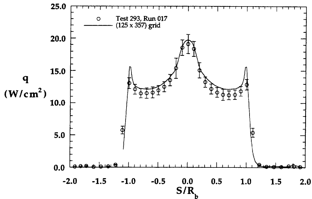
Figure 8.1.70a Comparison with Experimental Forebody Heating Distribution, MP-3 Configuration, 31-Inch Mach 10, Re_{\infty} = 1.0 \times 10^6 \text{ ft}^{-1}
