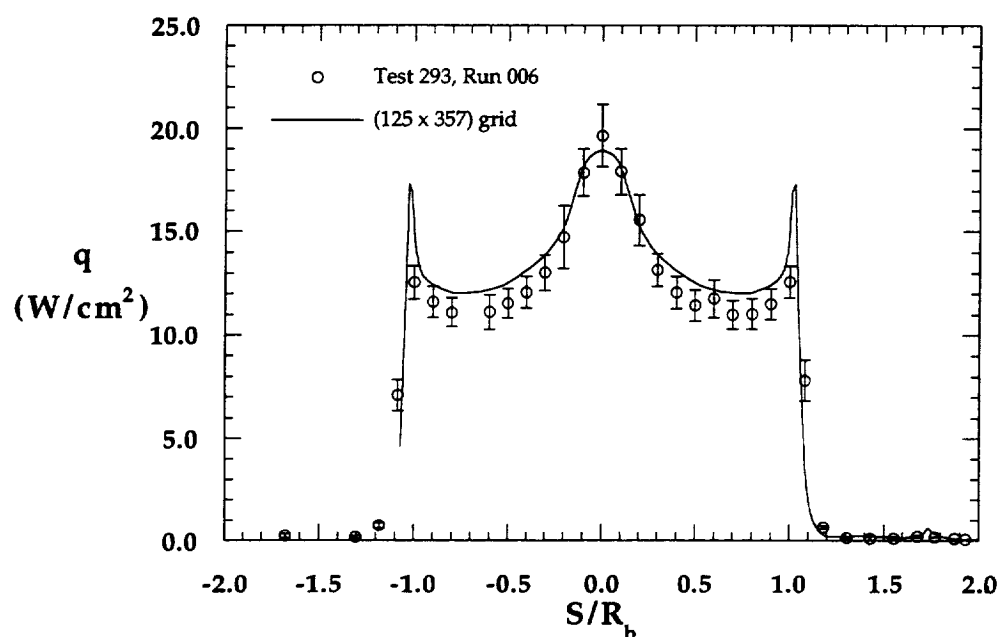
Figure 8.1.64a Comparison with Experimental Forebody Heating Distribution, MP-1 Configuration, 31-Inch Mach 10, \text{Re}_\infty = 1.0 \times 10^6 \text{ ft}^{-1}
