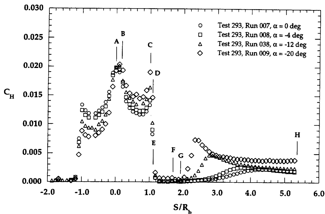
Figure 6.1.9a \alpha Effects on MP-1 Configuration, Re_\infty = 1.0 \times 10^6 \text{ ft}^{-1} (linear scale)
