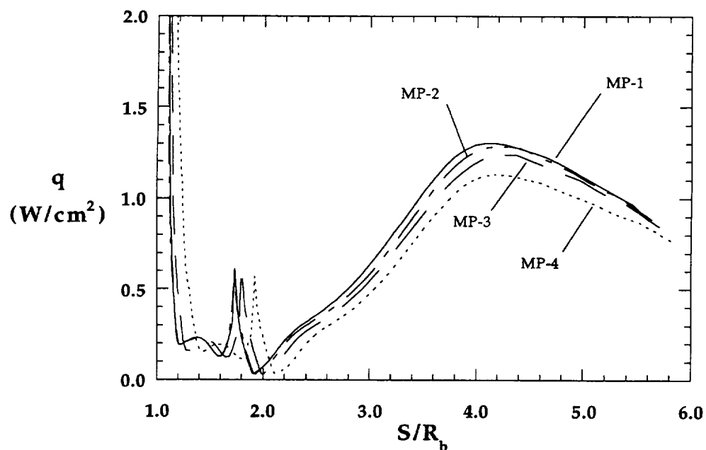
Figure 8.1.61b Configuration Effects on Wake Heating, 31-Inch Mach 10, Re_\infty = 1.0 \times 10^6 \text{ ft}^{-1}
