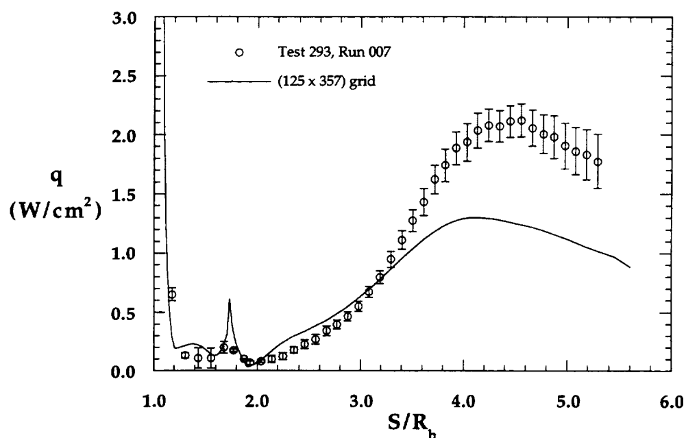
Figure 8.1.64b Comparison with Experimental Wake Heating Distribution, MP-1 Configuration, 31-Inch Mach 10, \text{Re}_\infty = 1.0 \times 10^6 \text{ ft}^{-1}
