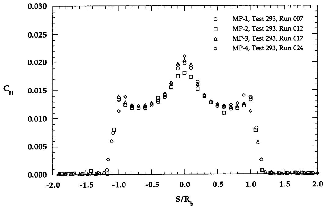
Figure 6.1.18a Configuration Effects on Forebody, \alpha = 0^\circ , Re_\infty = 1.0 \times 10^6 \text{ ft}^{-1}
