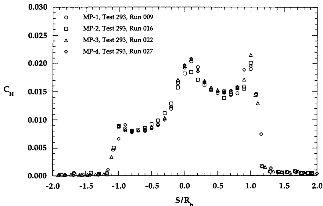
Figure 6.1.21a Configuration Effects on Forebody, \alpha = -20 deg, Re_\infty = 1.0 \times 10^6 \text{ ft}^{-1}
