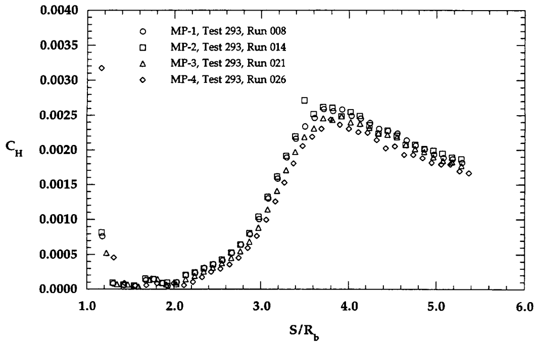
Figure 6.1.20b Configuration Effects on Wake, \alpha = -4 deg, Re_\infty = 1.0 \times 10^6 \text{ ft}^{-1}
