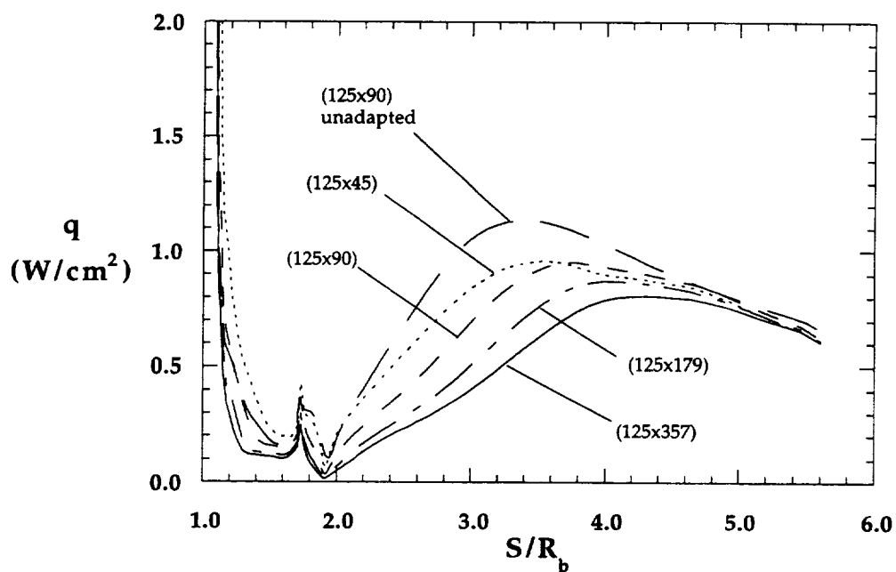
Figure 8.1.4b Grid Resolution Effects on Wake Heating, MP-1 Configuration, 31-Inch Mach 10, \text{Re}_\infty = 0.5 \times 10^{-6} \text{ ft}^{-1}
