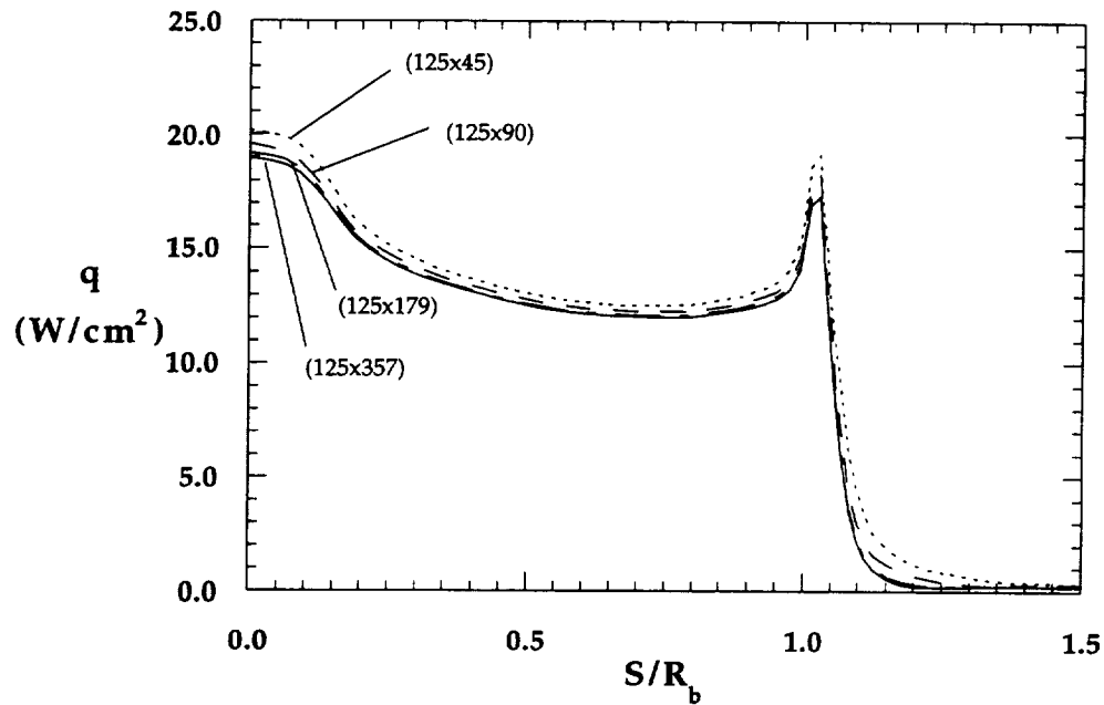
Figure 8.1.6a Grid Resolution Effects on Forebody Heating, MP-1 Configuration, 31-Inch Mach 10, \text{Re}_\infty = 1.0 \times 10^{-6} \text{ ft}^{-1}
