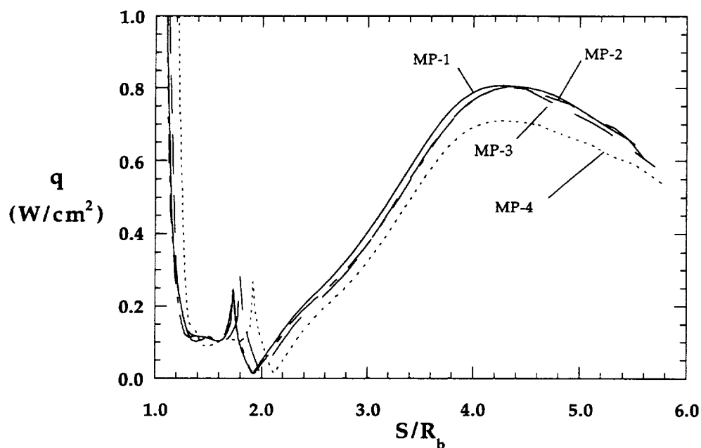
Figure 8.1.60b Configuration Effects on Wake Heating, 31-Inch Mach 10, \text{Re}_\infty = 0.5 \times 10^6 \text{ ft}^{-1}
