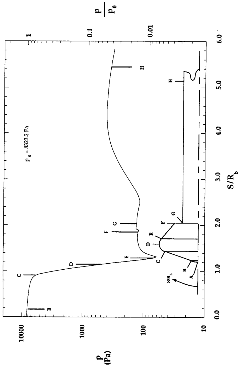
Figure 8.1.49 Computed Surface Pressure Distribution, MP-4 Configuration, 31-Inch Mach 10, Re_\infty = 0.5 \times 10^6
