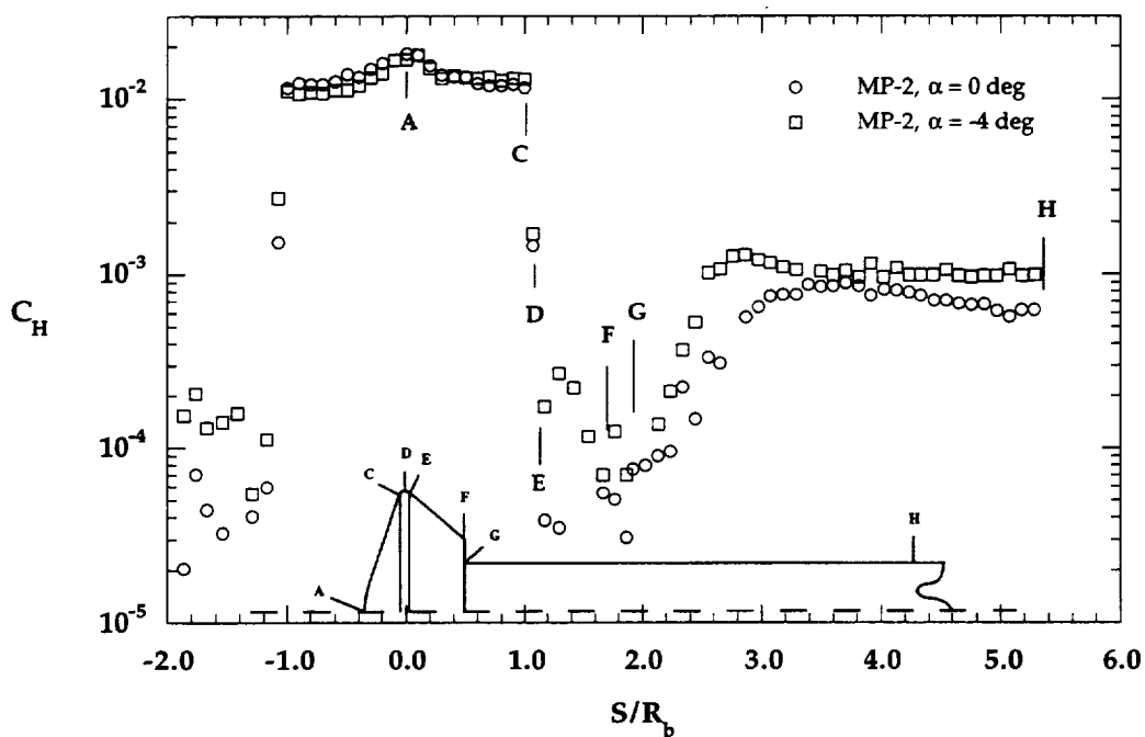
Figure 6.2.15b \alpha Effects on MP-2 Configuration, \text{CO}_2 in HYPULSE (log scale)
