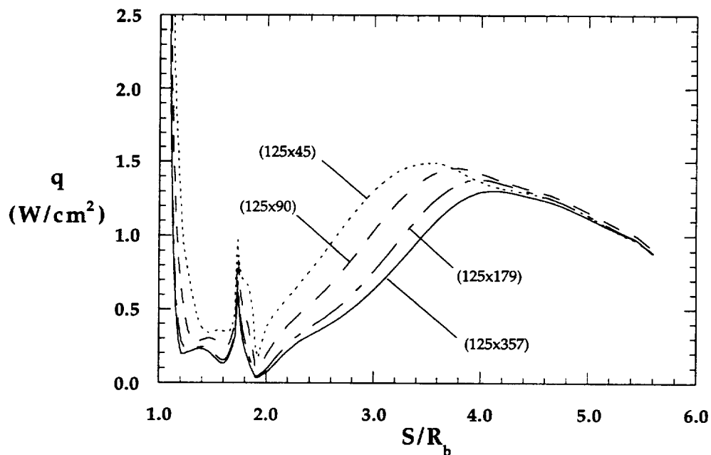
Figure 8.1.6b Grid Resolution Effects on Wake Heating, MP-1 Configuration, 31-Inch Mach 10, \text{Re}_\infty = 1.0 \times 10^{-6} \text{ ft}^{-1}
