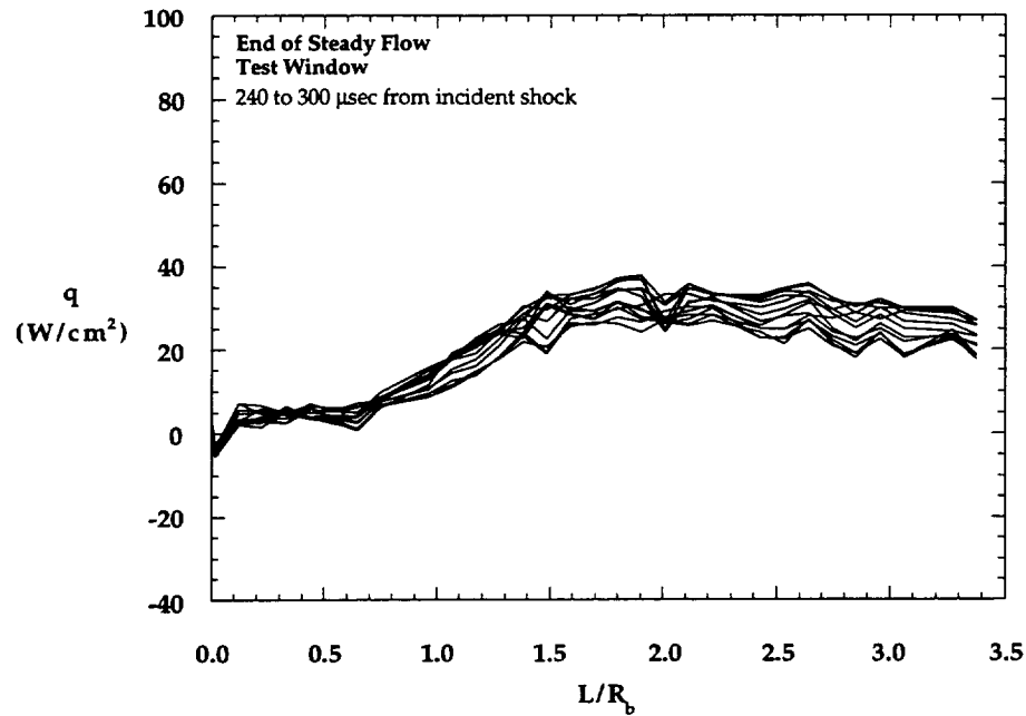
Figure 6.2.1e Wake Flow Establishment Movie, Run 749: 240 to 300 \mu\text{sec}
