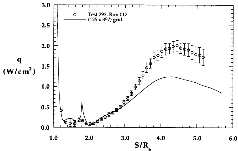
Figure 8.1.70b Comparison with Experimental Wake Heating Distribution, MP-3 Configuration, 31-Inch Mach 10, Re_{\infty} = 1.0 \times 10^6 \text{ ft}^{-1}
