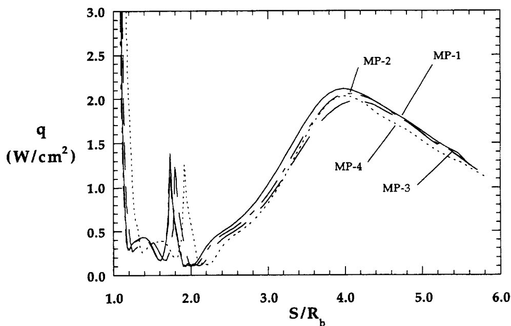
Figure 8.1.62b Configuration Effects on Wake Heating, 31-Inch Mach 10, \text{Re}_\infty = 2.0 \times 10^6 \text{ ft}^{-1}
