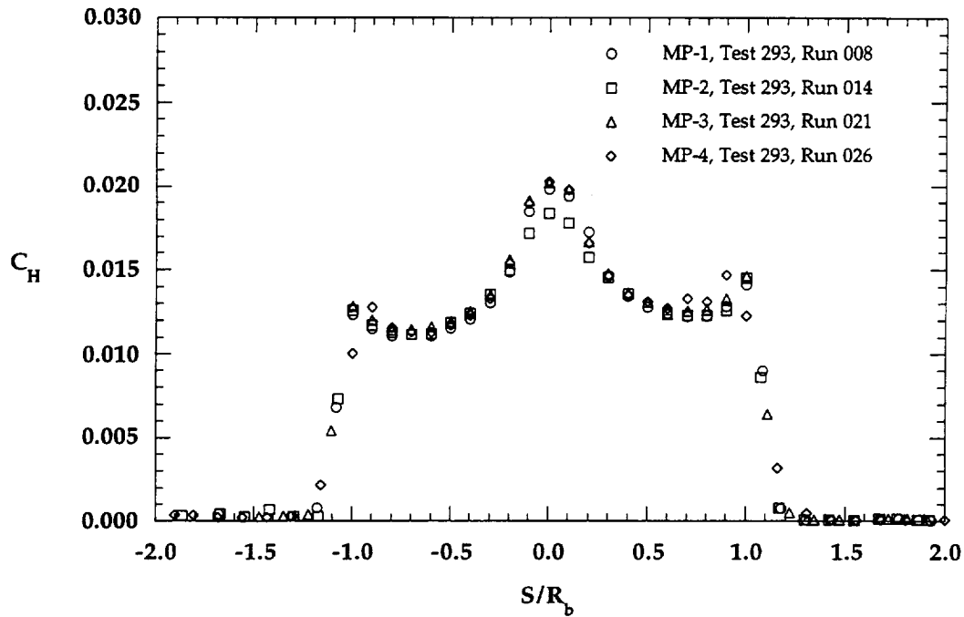
Figure 6.1.20a Configuration Effects on Forebody, \alpha = -4 deg, Re_\infty = 1.0 \times 10^6 \text{ ft}^{-1}
