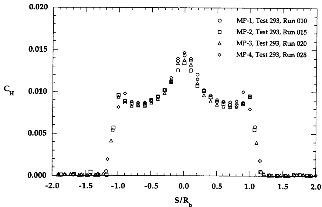
Figure 6.1.19a Configuration Effects on Forebody, \alpha = 0^\circ , Re_\infty = 2.0 \times 10^6 \text{ ft}^{-1}
