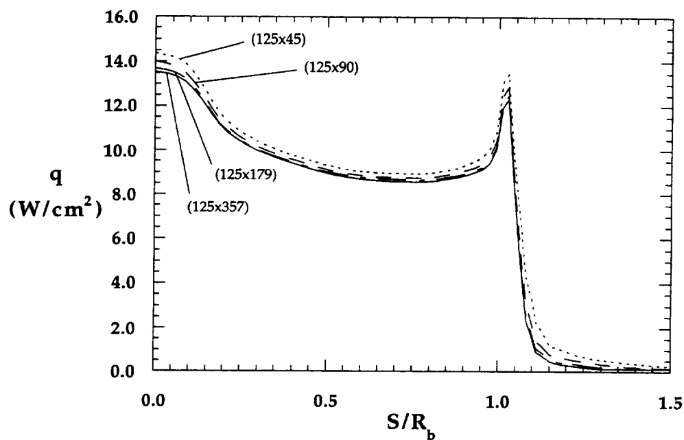
Figure 8.1.4a Grid Resolution Effects on Forebody Heating, MP-1 Configuration, 31-Inch Mach 10, \text{Re}_\infty = 0.5 \times 10^{-6} \text{ ft}^{-1}
