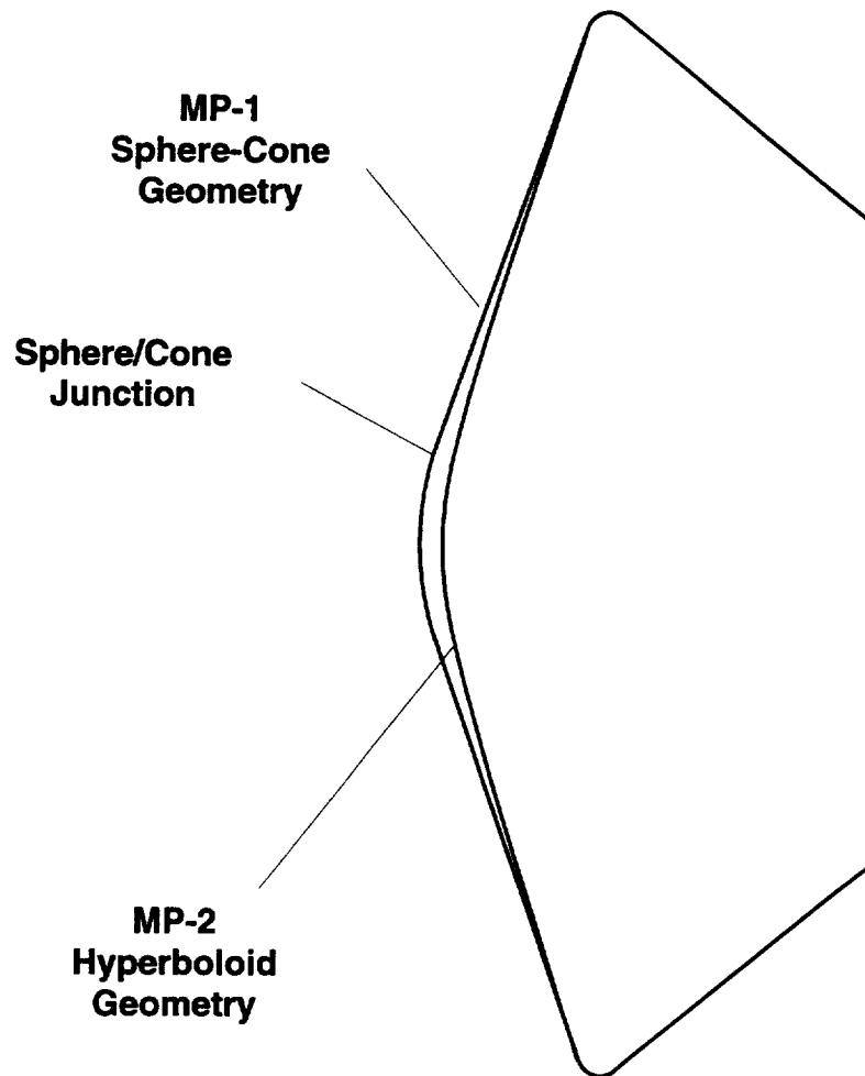
Figure 3.1.4 MP-1 and MP-2 Configurations
