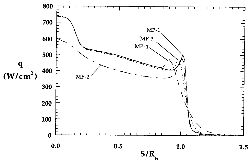
Figure 8.2.44a Configuration Effects on Forebody Heating Distributions, HYPULSE, CO 2
