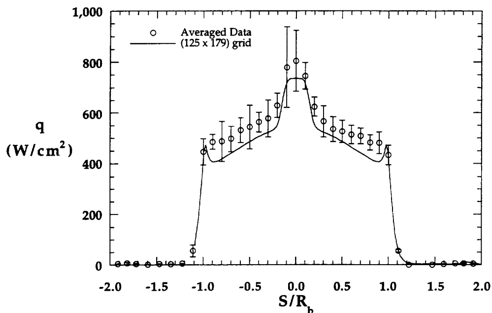
Figure 8.2.53a Comparison with Experimental Forebody Heating Distribution, MP-3 Configuration, HYPULSE, \text{CO}_2
