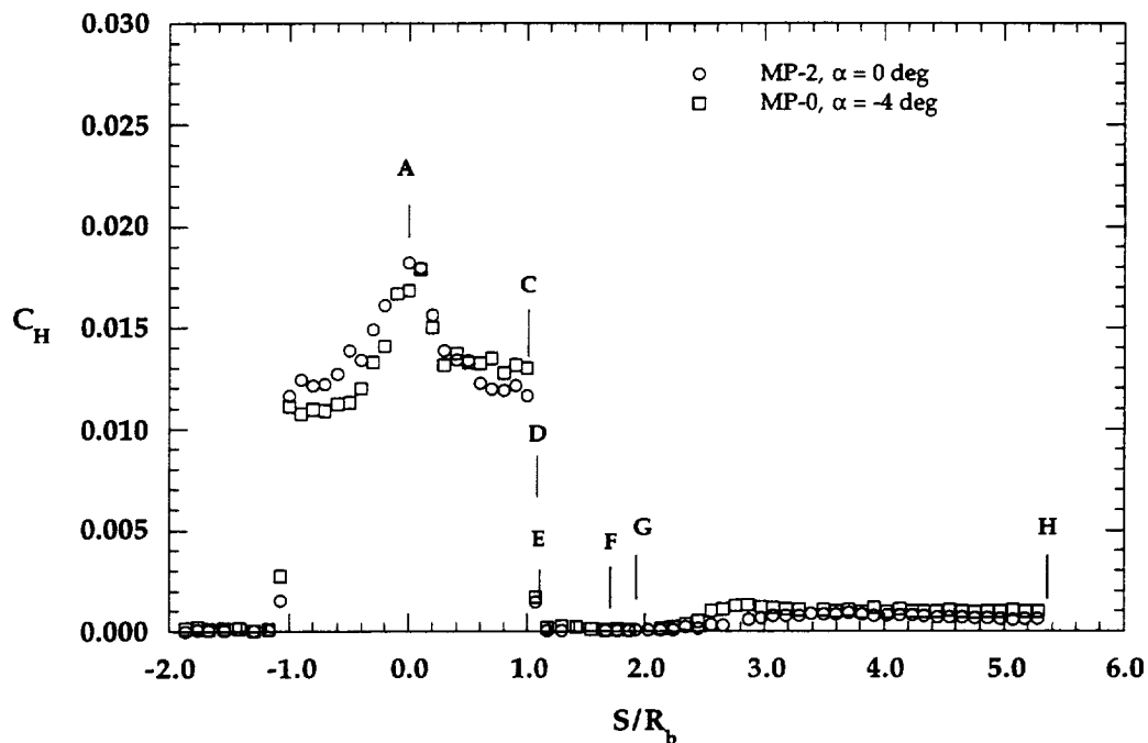
Figure 6.2.15a \alpha Effects on MP-2 Configuration, \text{CO}_2 in HYPULSE (linear scale)
