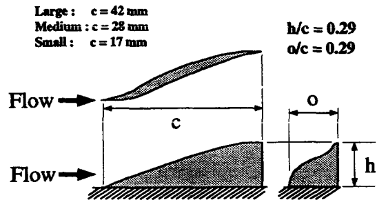
Figure 5 Geometry of the tapered fin vortex generator.
