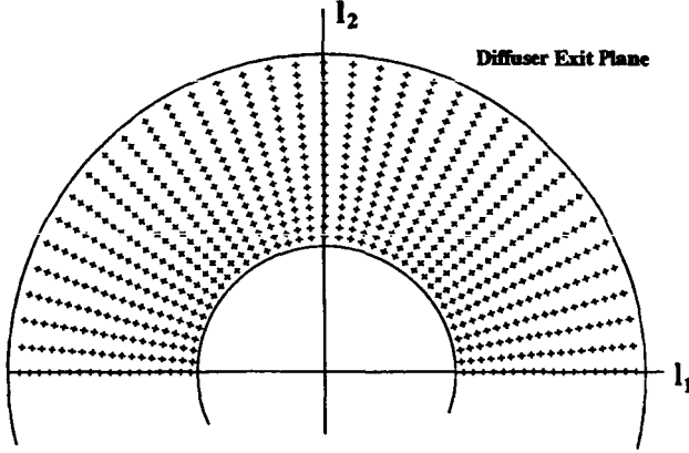
Figure 6 The experimental grid at the diffuser exit showing lines of flow field symmetry.
