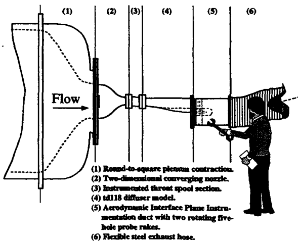
Figure 4 The diffuser test rig.
