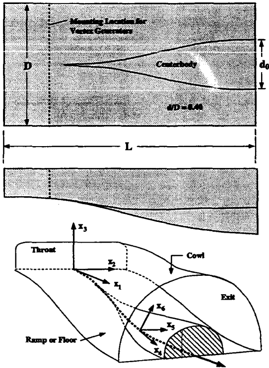
Figure 3 Three views of the td118 diffuser.
