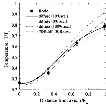
Fig. 15 Effect of wall interaction models on the rotational temperature profiles at the plane near the exit.
