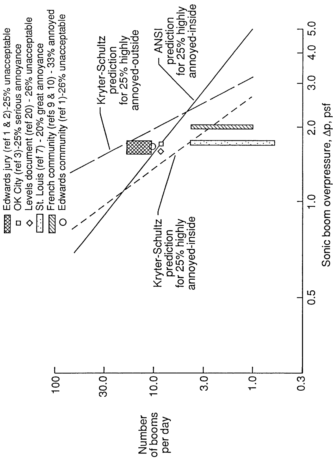
Figure 15. Comparisons of predicted and observed community exposures to sonic booms for a 25 percent highly annoyed community response
