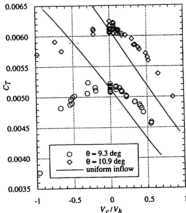
Figure 5. Comparison of predicted and measured rotor thrust with uniform inflow and fixed collective.
