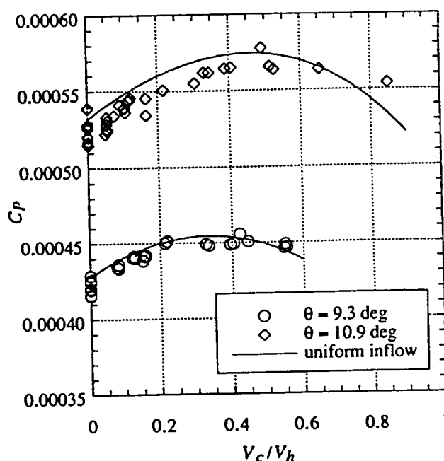
Figure 7. Comparison of predicted and measured rotor power with uniform inflow. Collective pitch varied to match measured thrust.
