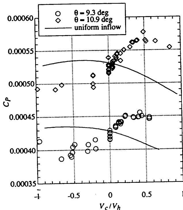
Figure 6. Comparison of predicted and measured rotor power with uniform inflow and fixed collective.
