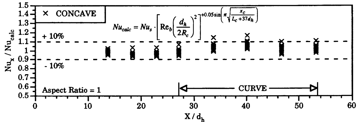
Figure 5c. Concave surface results from test section TS3 with the Kumakawa et al. 3 curvature factor applied.
